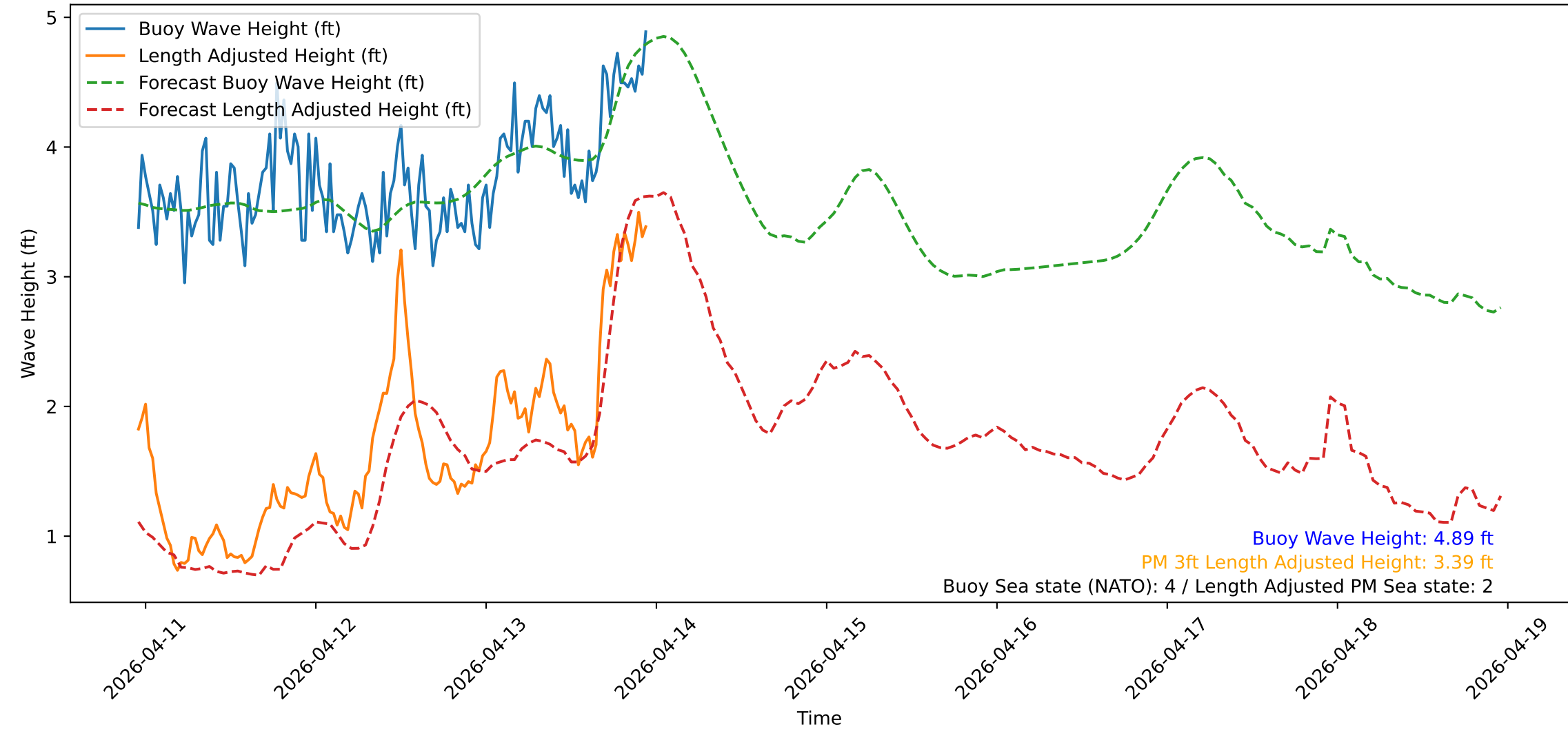
Wave Heights over Time for Green Beach at 2026-04-13 23:11:12
