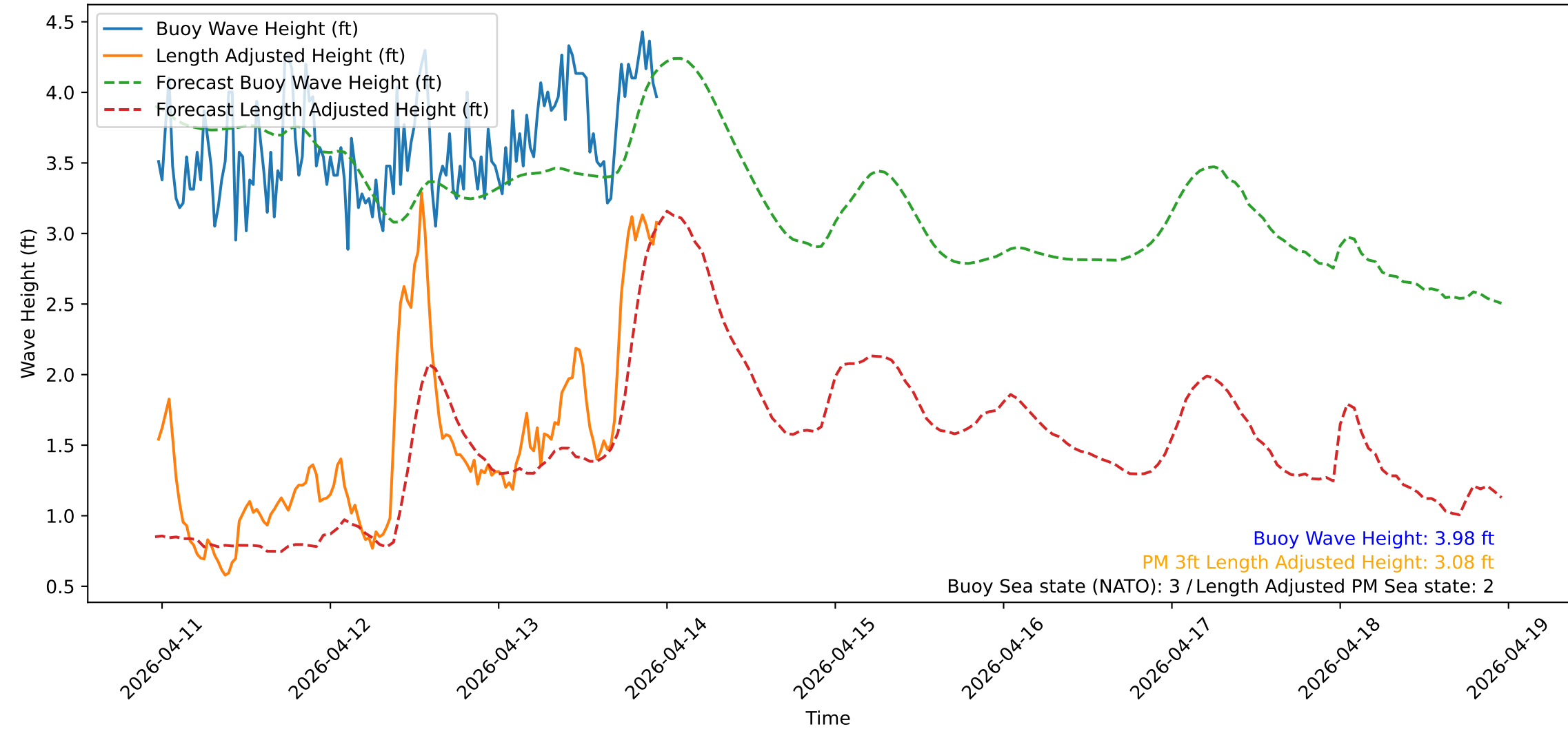
Wave Heights over Time for Red Beach at 2026-04-13 23:10:50
