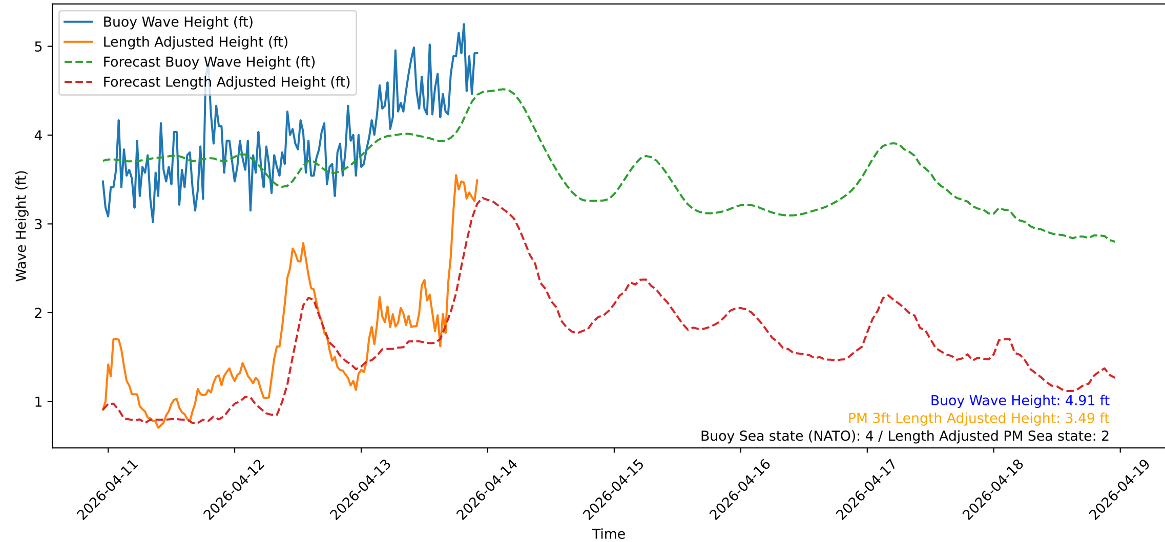
Wave Heights over Time for Oceanside Harbor at 2026-04-13 23:10:31
