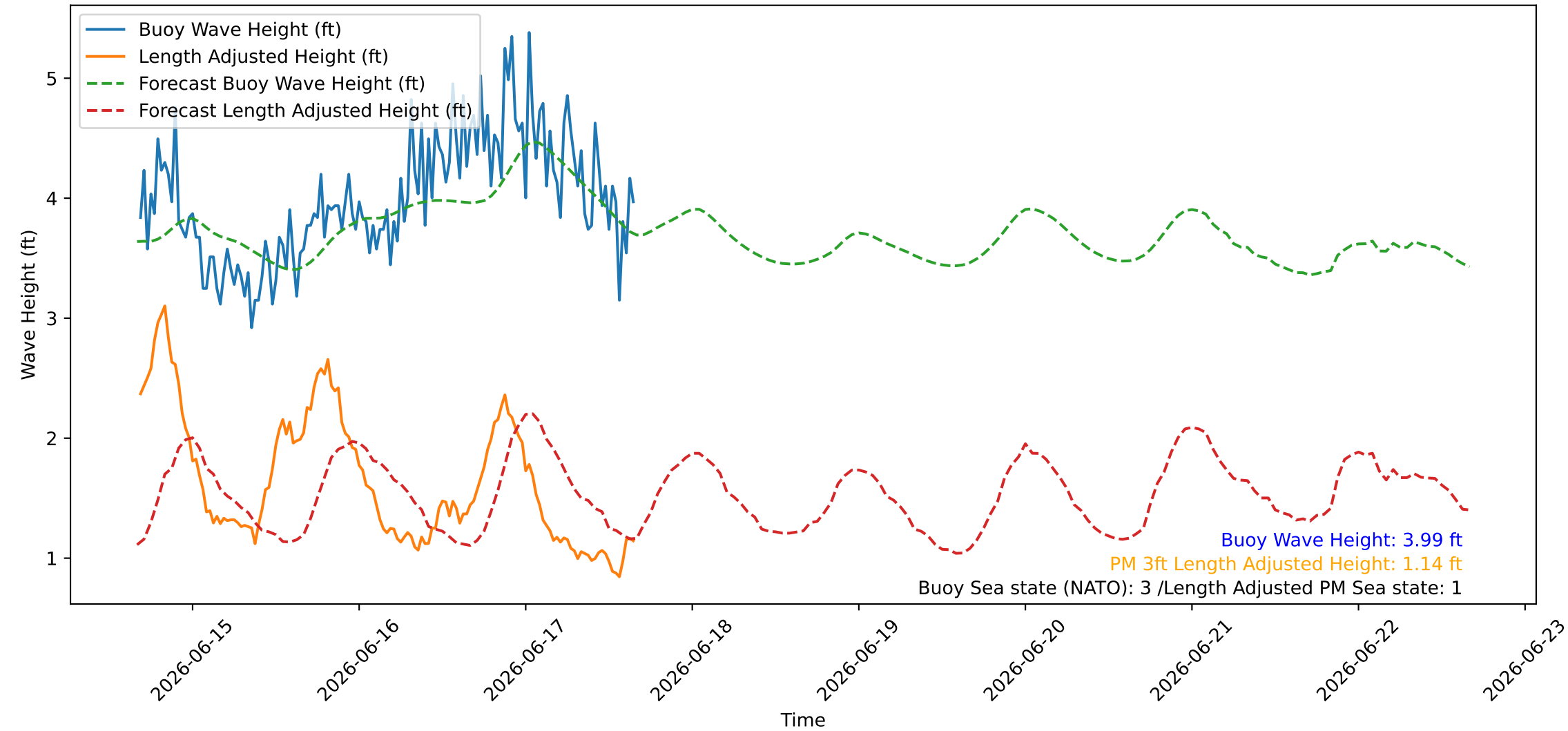
Wave Heights over Time for Red Beach at 2026-06-17 16:20:47
