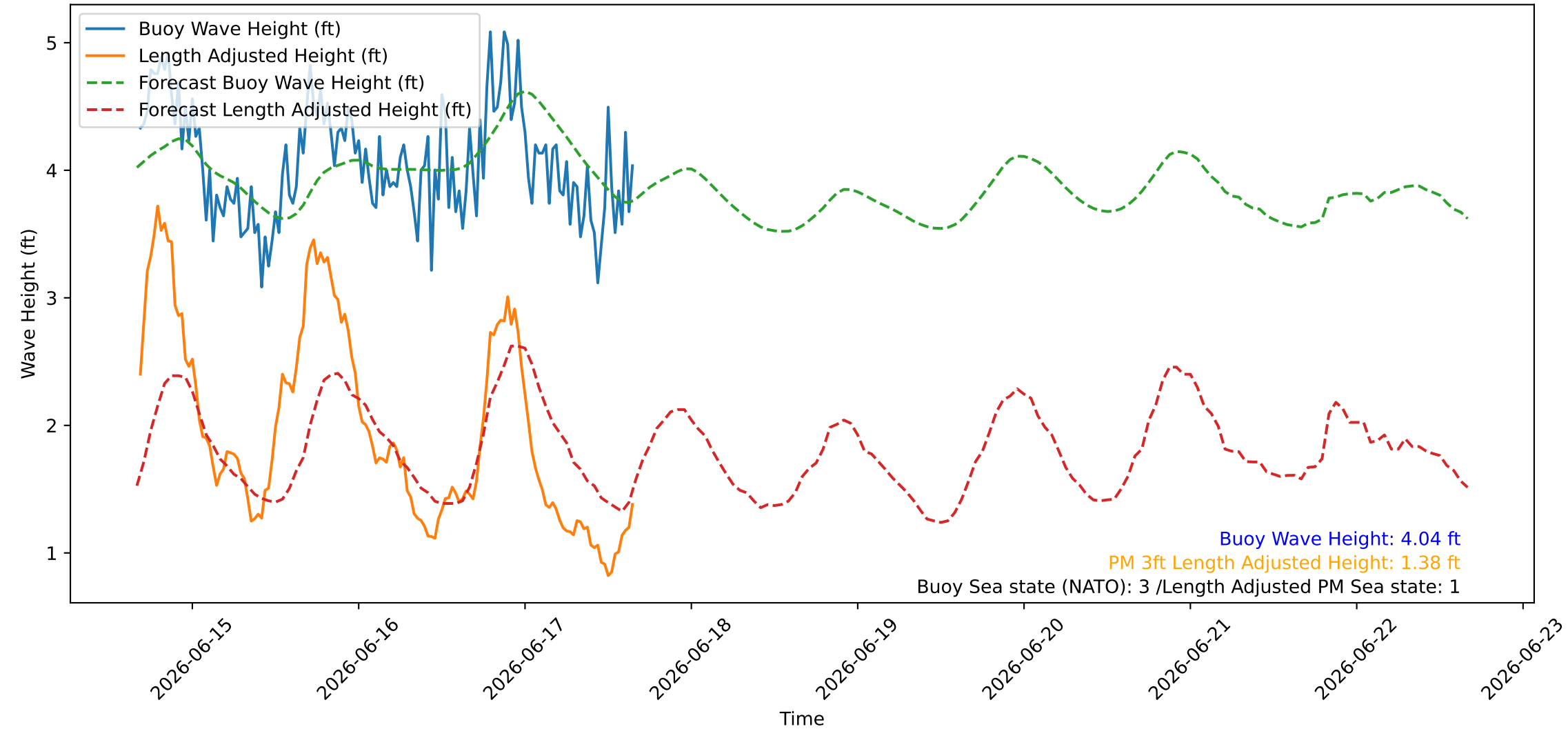
Wave Heights over Time for Green Beach at 2026-06-17 16:21:10
