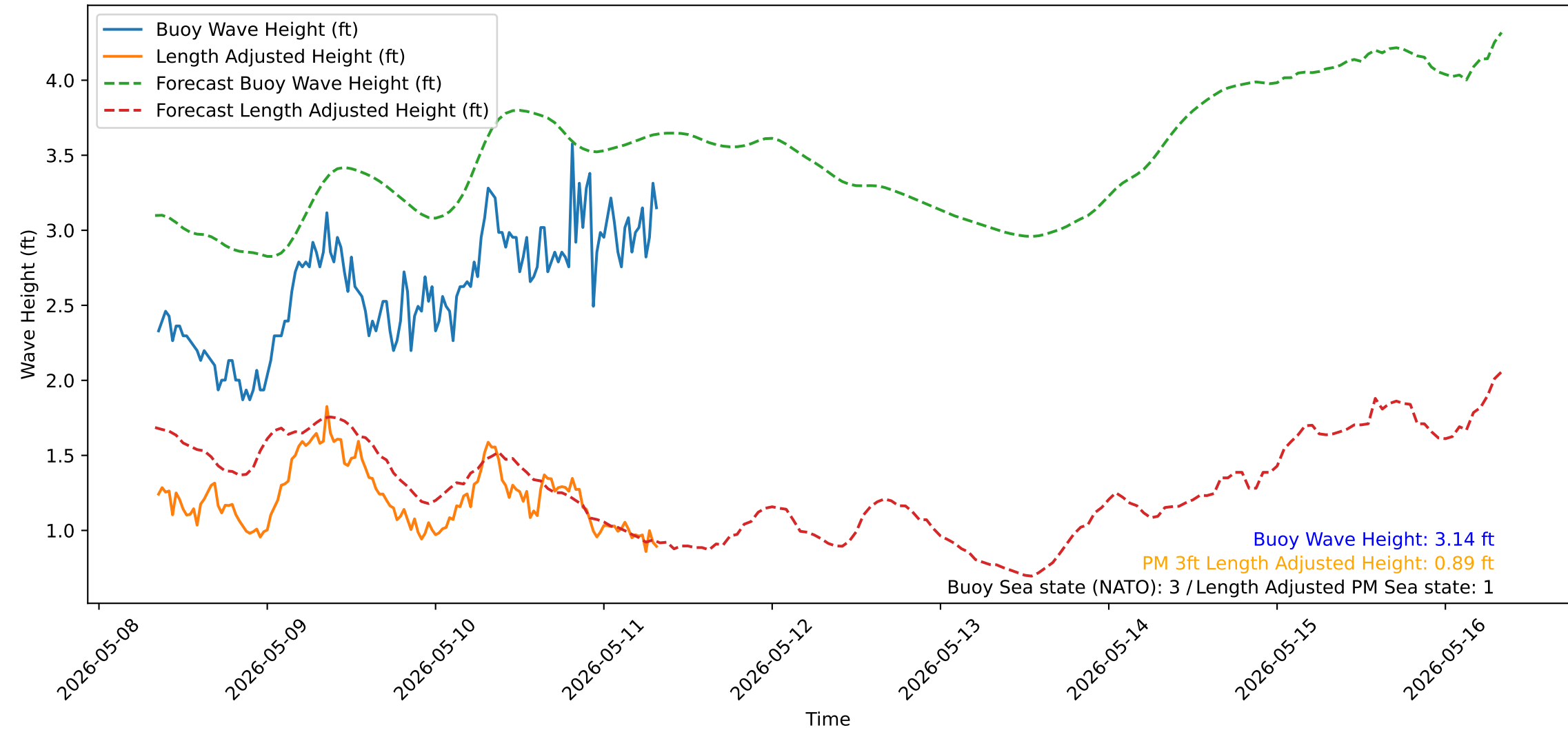
Wave Heights over Time for Oceanside Harbor at 2026-05-11 08:20:31
