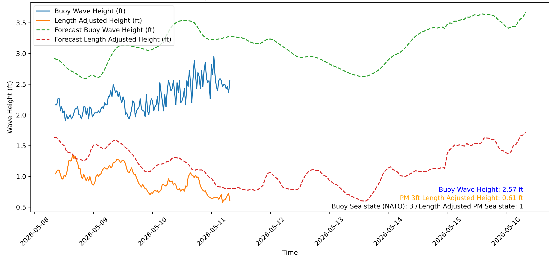
Wave Heights over Time for Red Beach at 2026-05-11 08:20:52
