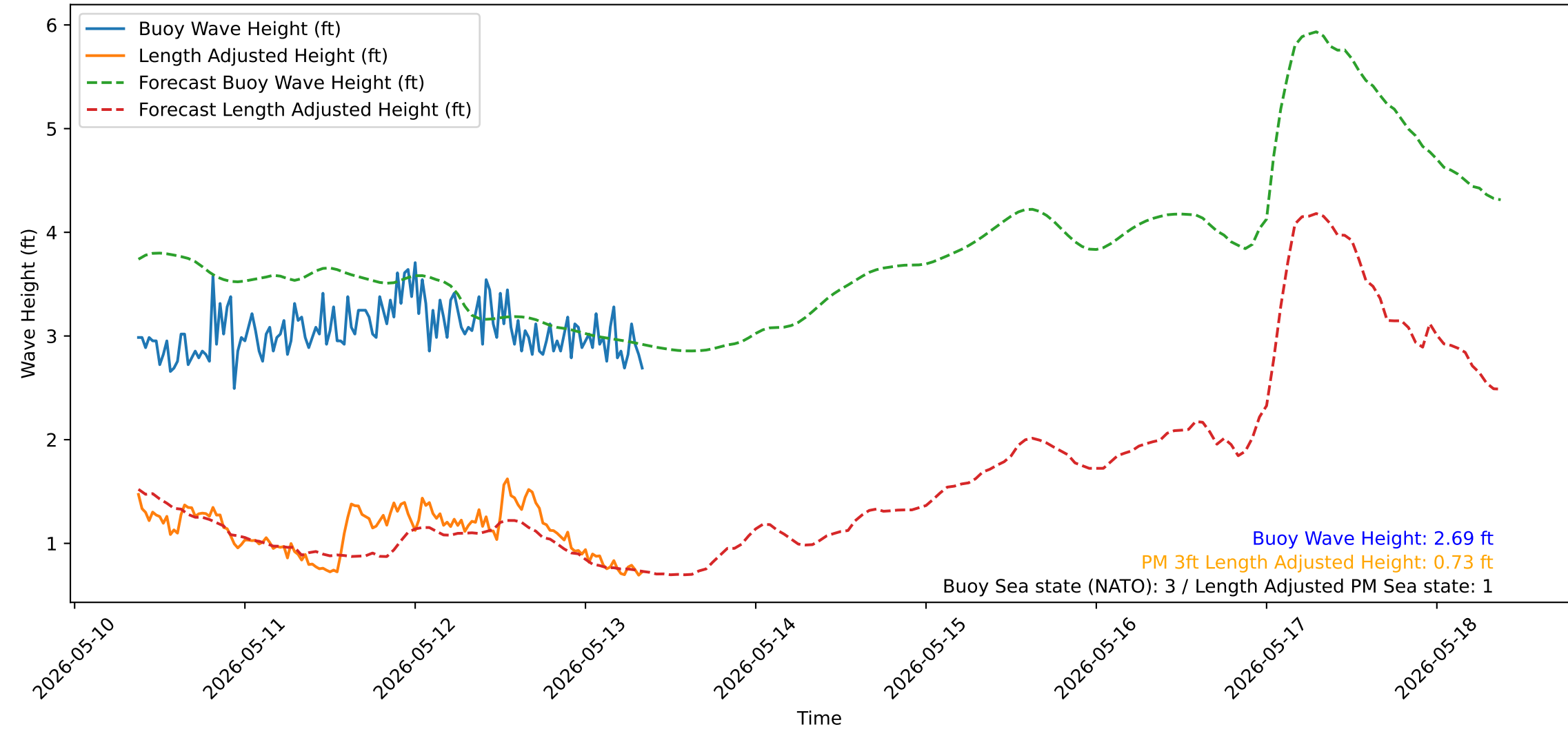
Wave Heights over Time for Oceanside Harbor at 2026-05-13 08:50:32
