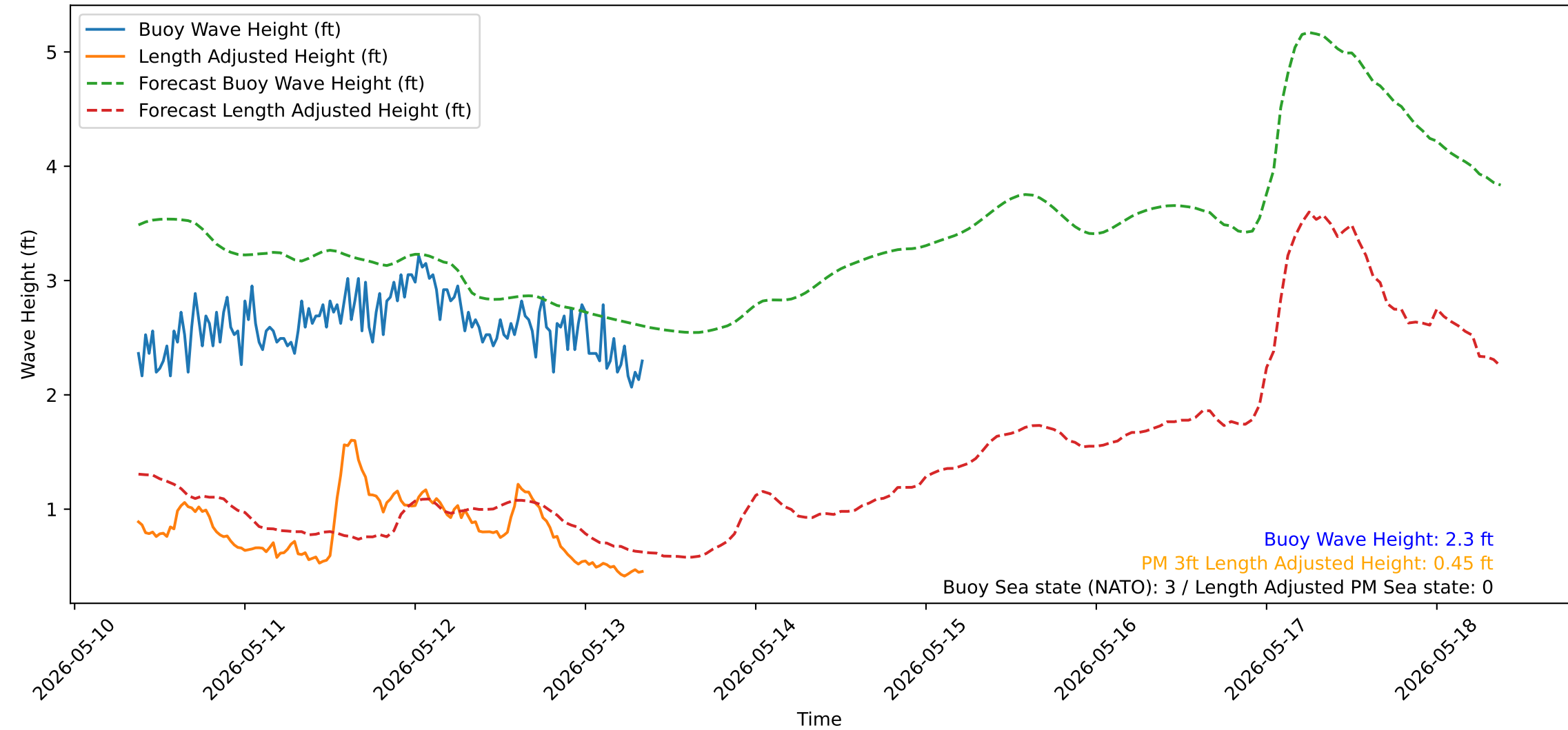
Wave Heights over Time for Red Beach at 2026-05-13 08:50:52
