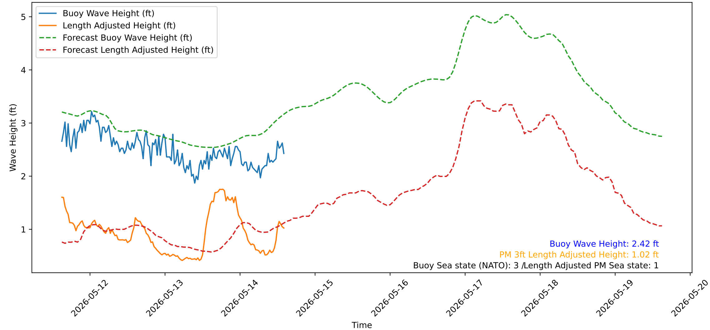
Wave Heights over Time for Red Beach at 2026-05-14 14:40:51
