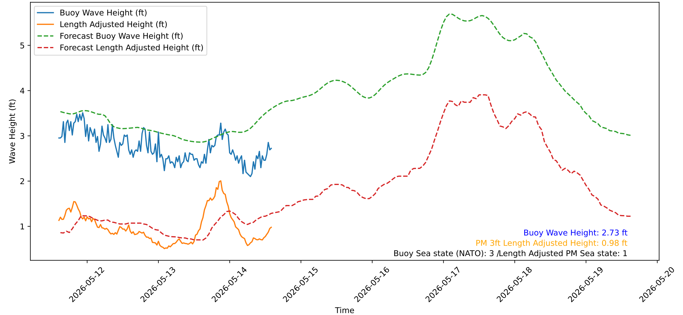
Wave Heights over Time for Green Beach at 2026-05-14 14:41:15
