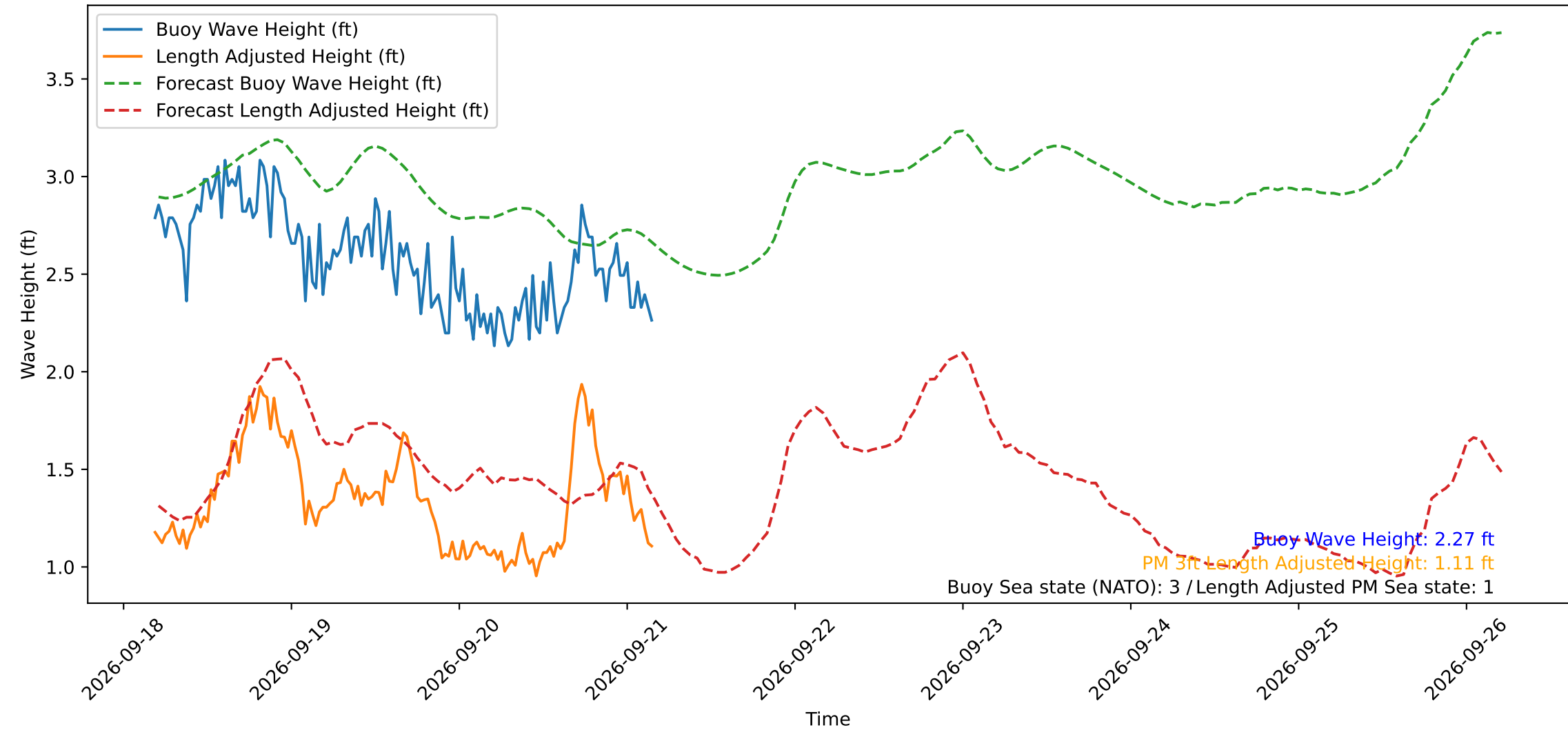
Wave Heights over Time for Oceanside Harbor at 2026-09-21 04:30:29
