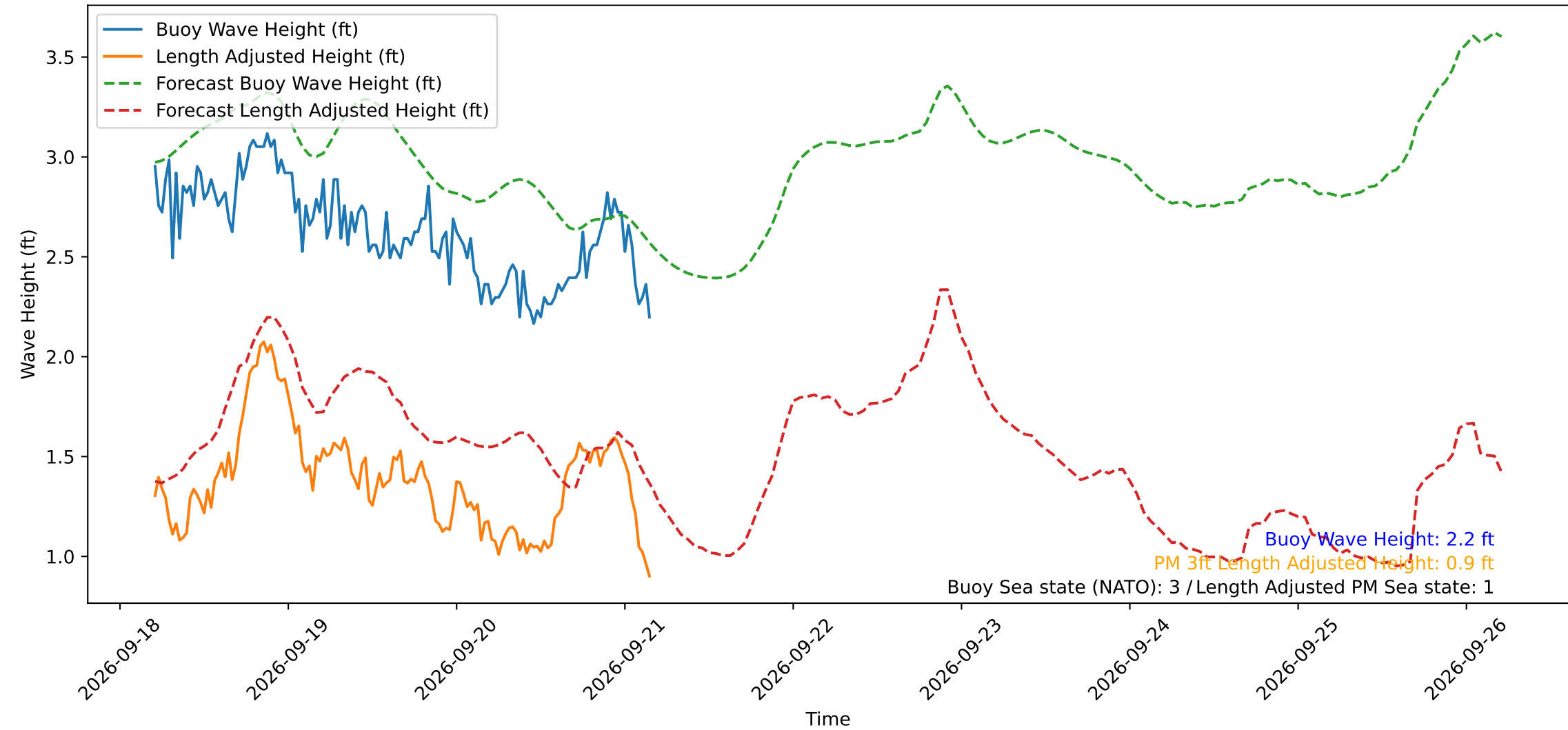
Wave Heights over Time for Green Beach at 2026-09-21 04:31:11
