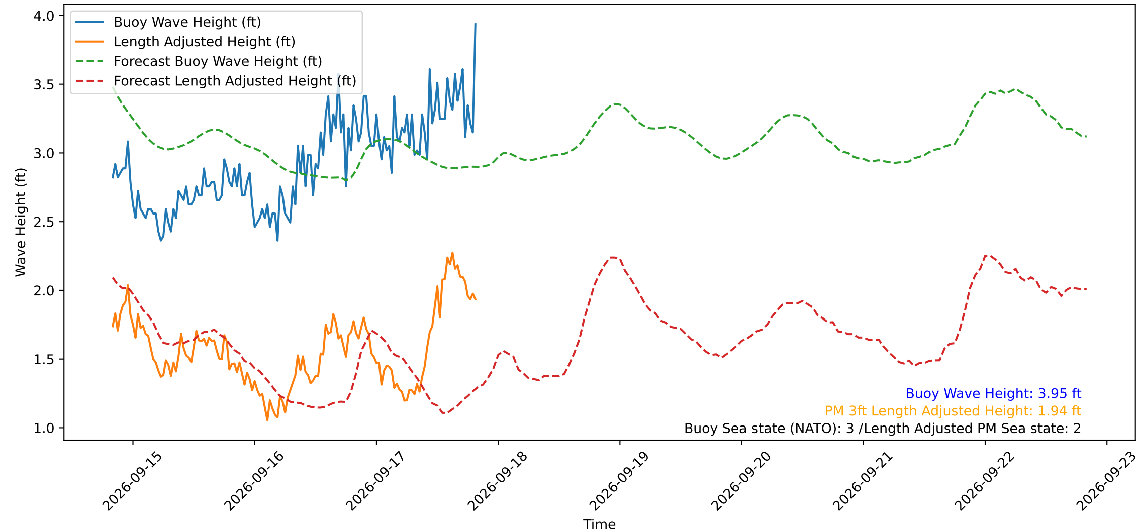
Wave Heights over Time for Oceanside Harbor at 2026-09-17 20:10:29
