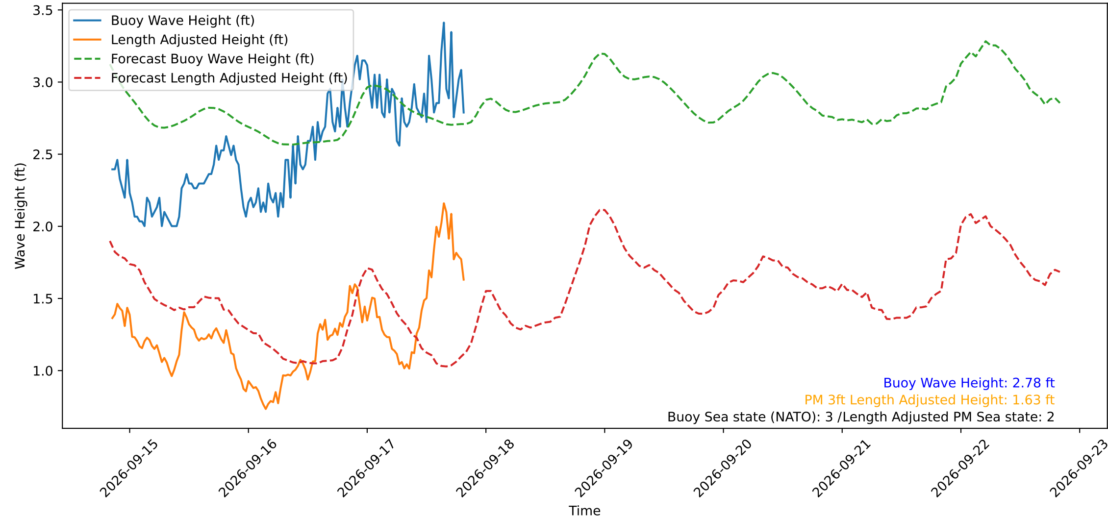
Wave Heights over Time for Red Beach at 2026-09-17 20:10:50
