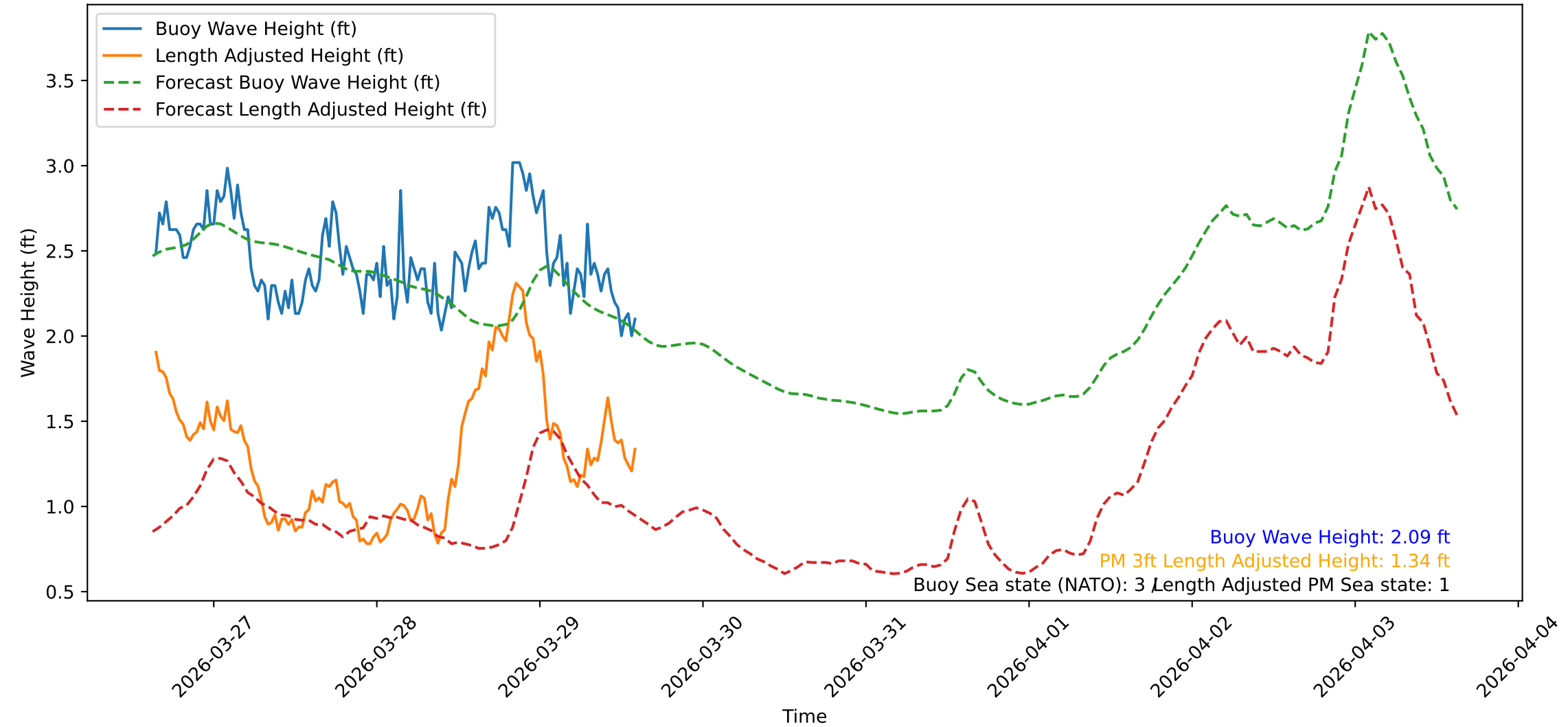
Wave Heights over Time for Red Beach at 2026-03-29 15:00:47
