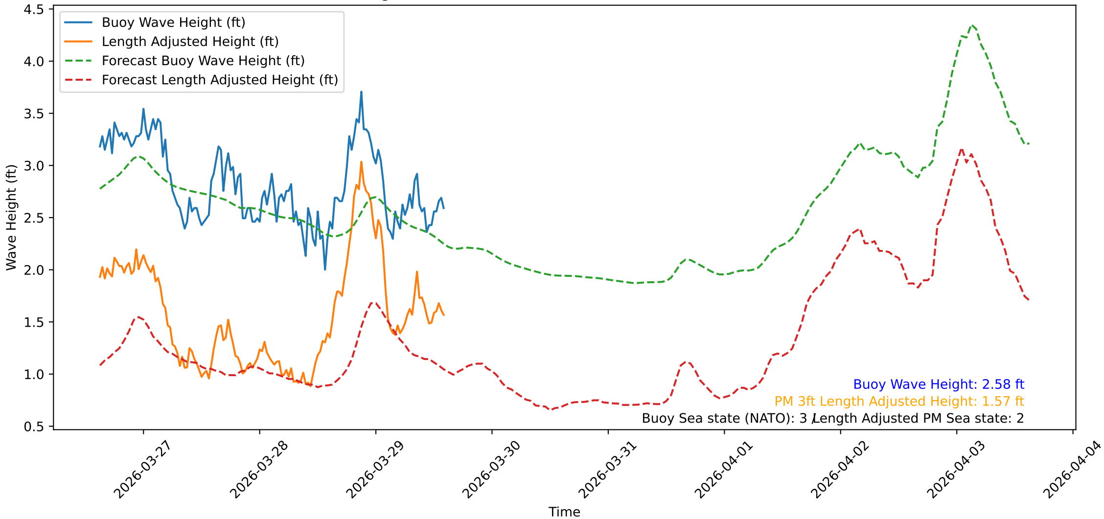
Wave Heights over Time for Green Beach at 2026-03-29 15:01:09
