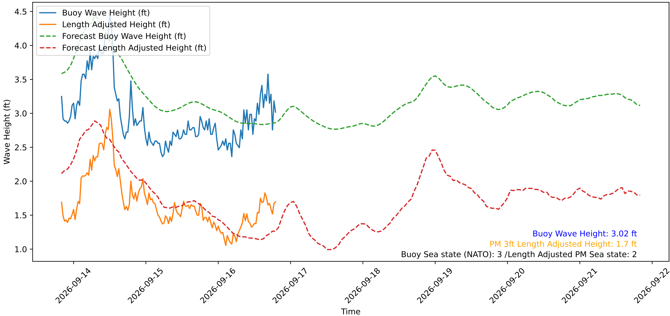
Wave Heights over Time for Oceanside Harbor at 2026-09-16 20:00:30
