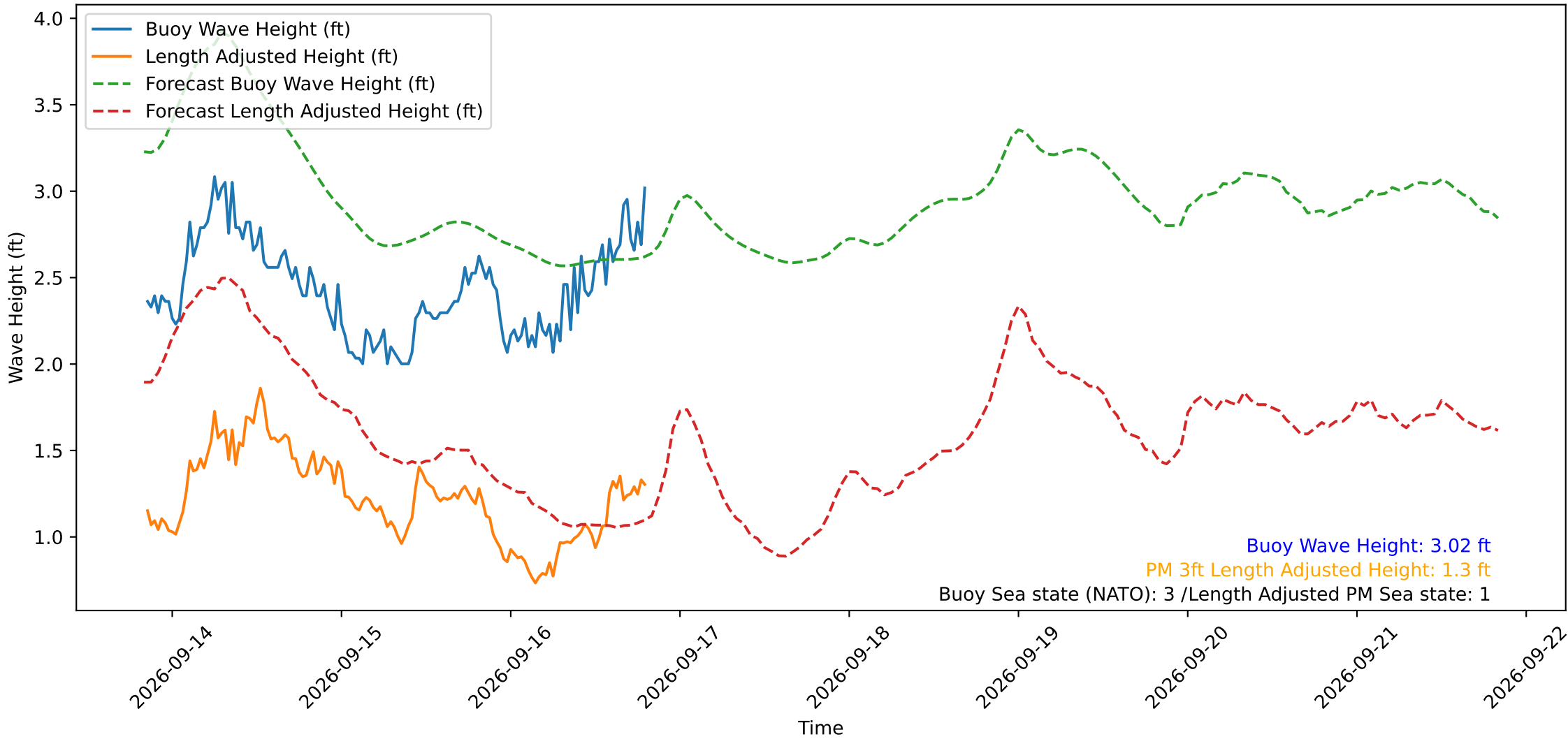
Wave Heights over Time for Red Beach at 2026-09-16 20:00:50
