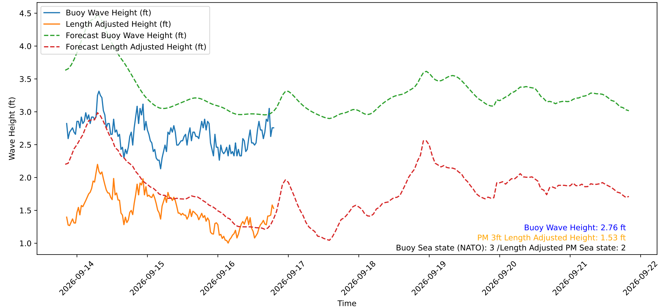
Wave Heights over Time for Green Beach at 2026-09-16 20:01:12
