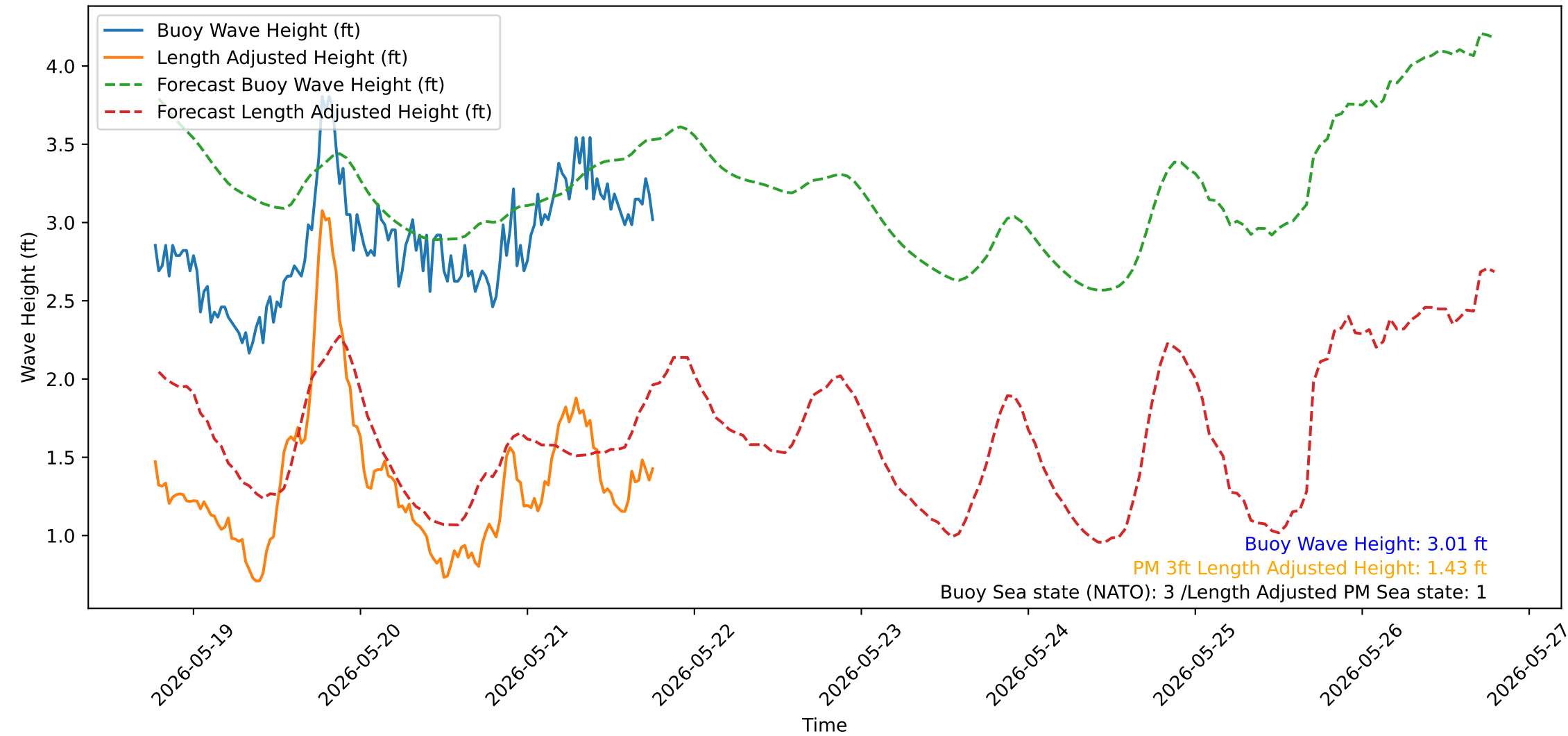
Wave Heights over Time for Green Beach at 2026-05-21 18:41:14
