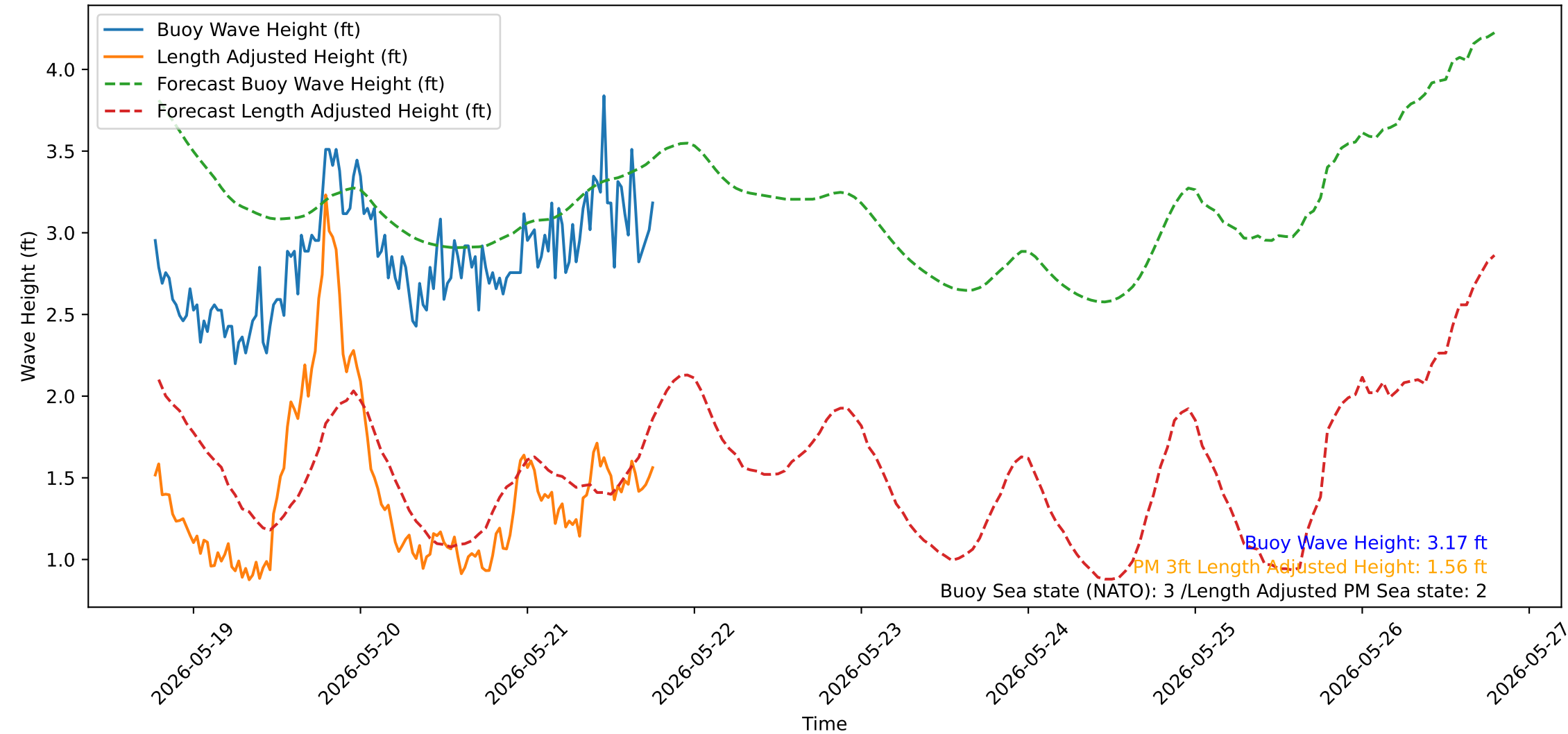
Wave Heights over Time for Oceanside Harbor at 2026-05-21 18:40:32
