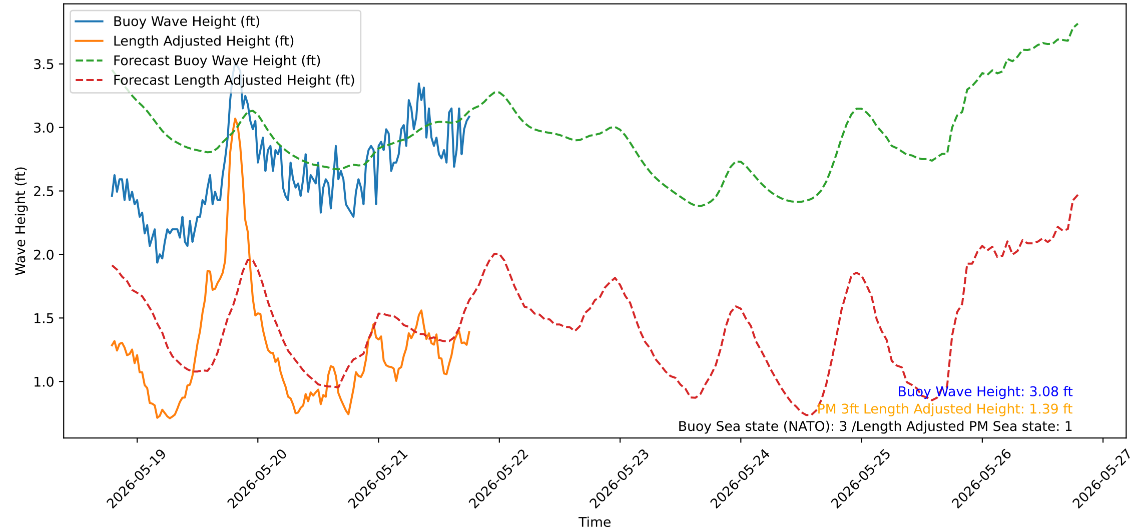
Wave Heights over Time for Red Beach at 2026-05-21 18:40:51
