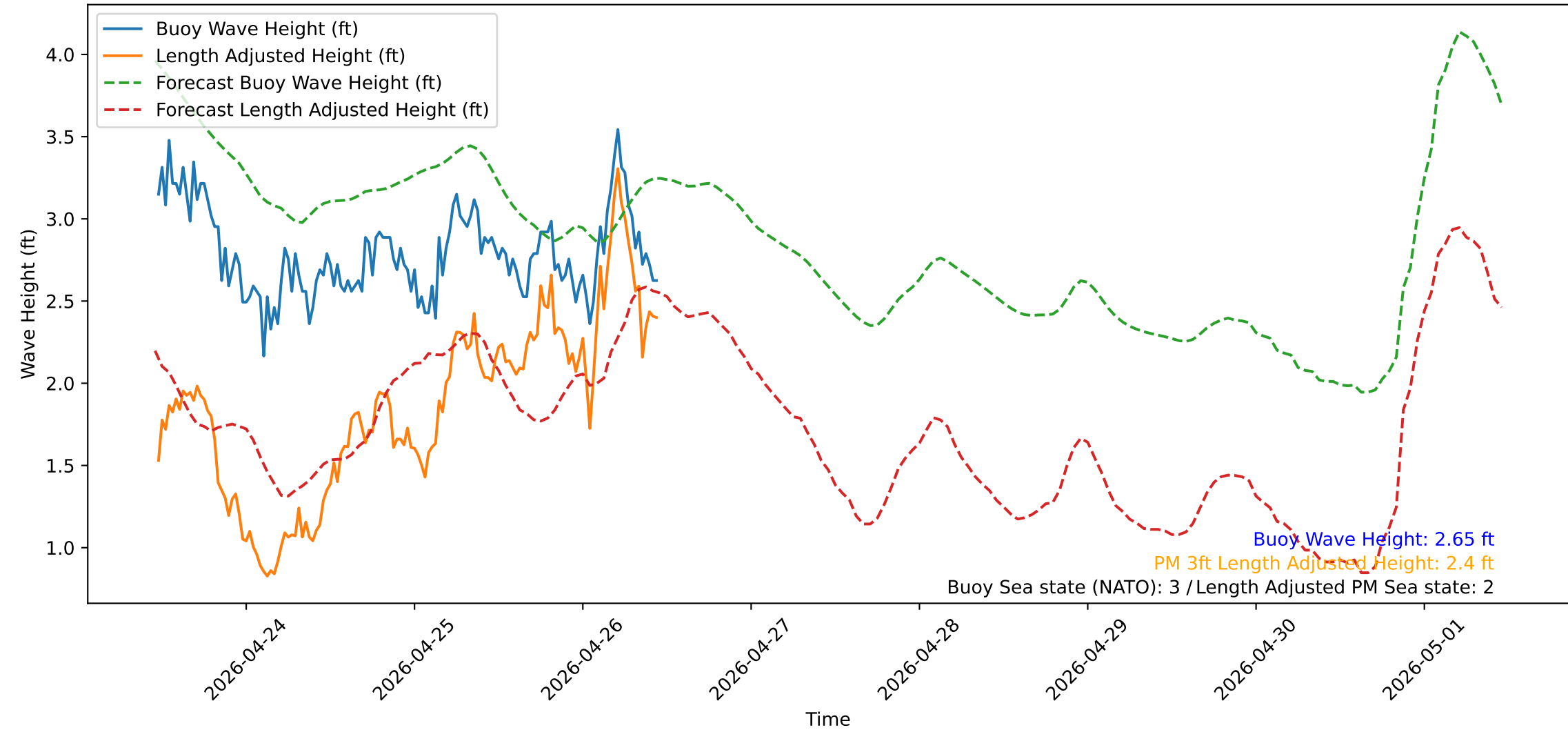
Wave Heights over Time for Red Beach at 2026-04-26 11:10:50
