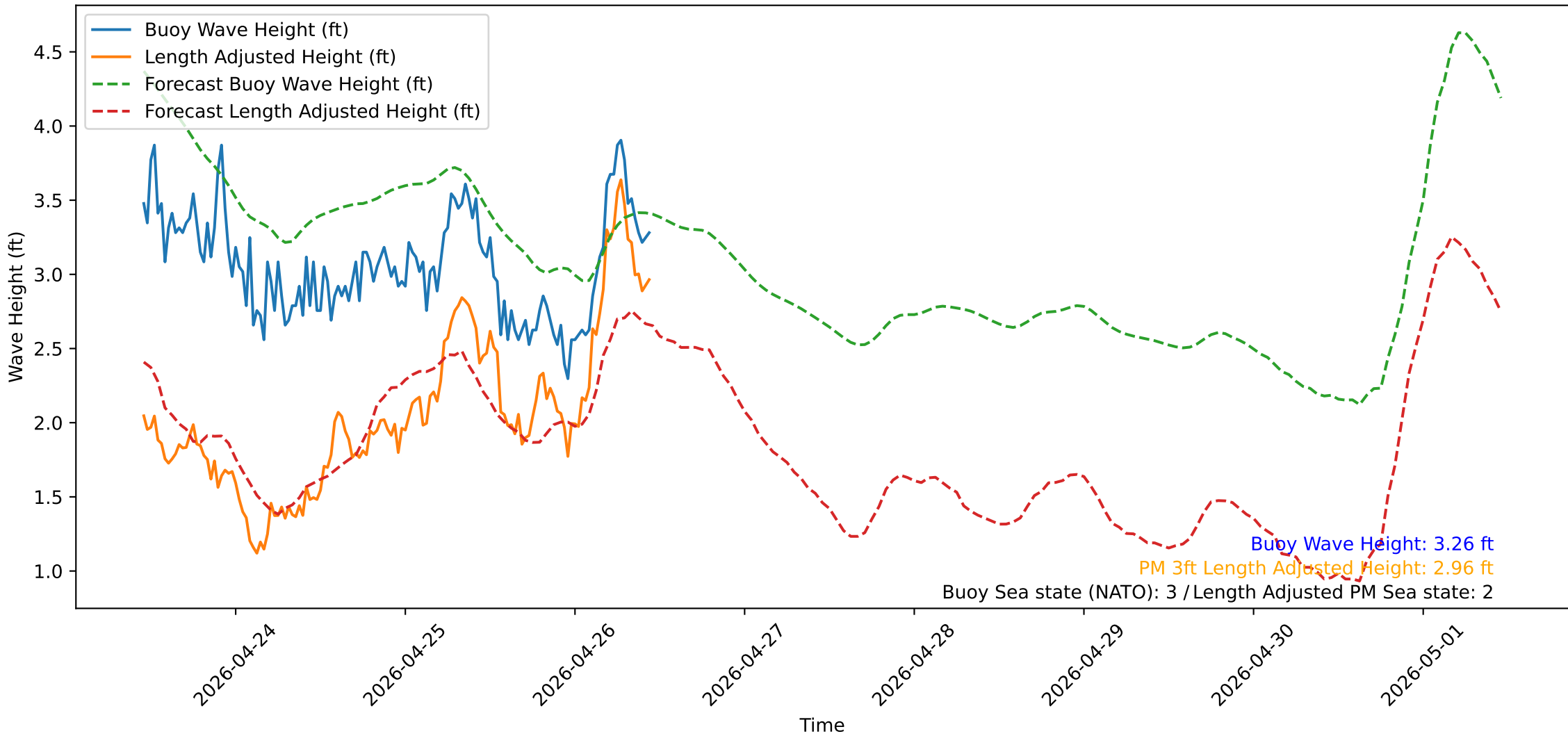
Wave Heights over Time for Oceanside Harbor at 2026-04-26 11:10:31
