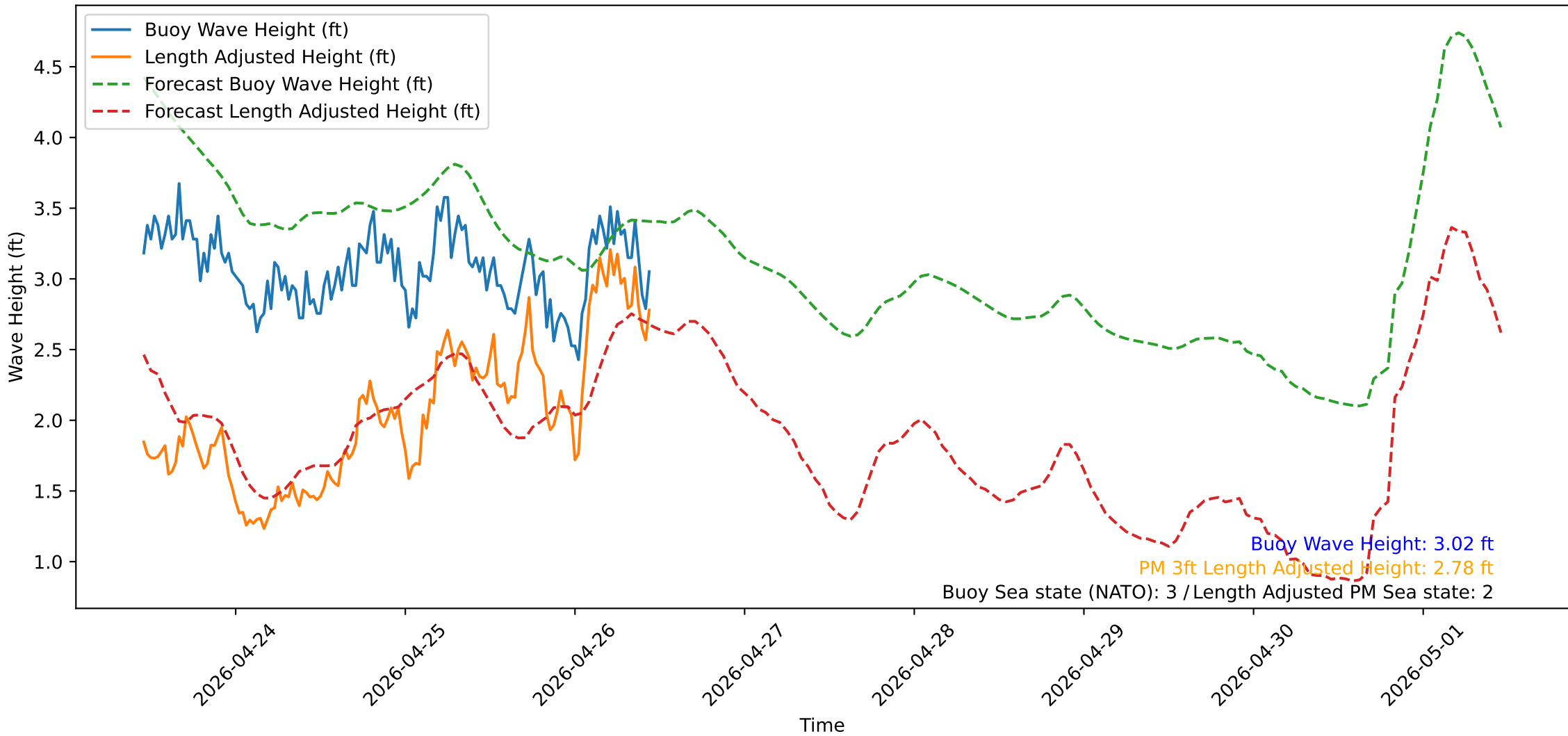
Wave Heights over Time for Green Beach at 2026-04-26 11:11:12
