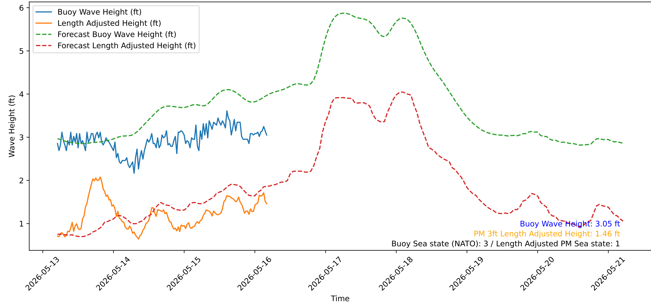
Wave Heights over Time for Oceanside Harbor at 2026-05-16 04:50:31
