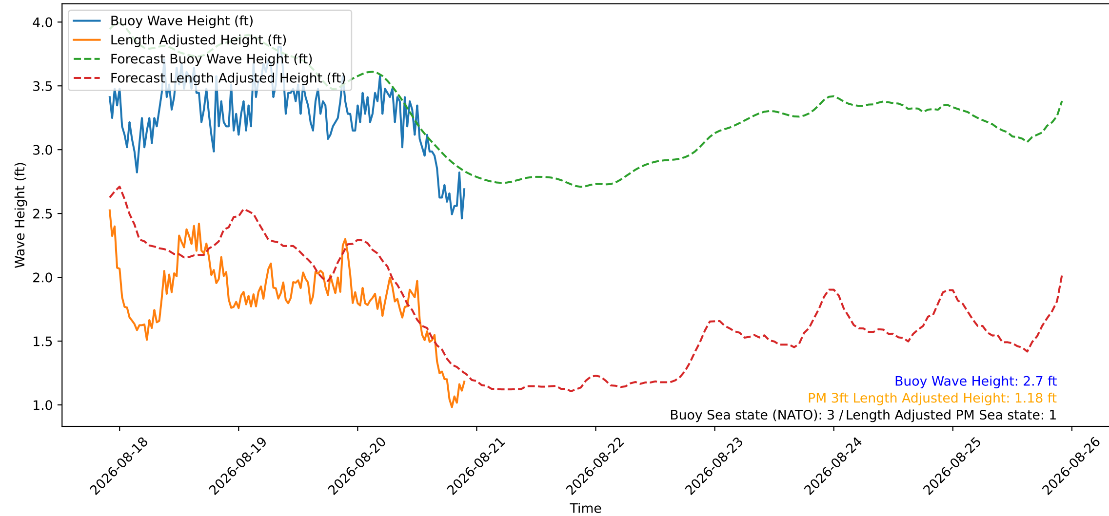
Wave Heights over Time for Oceanside Harbor at 2026-08-20 22:00:26
