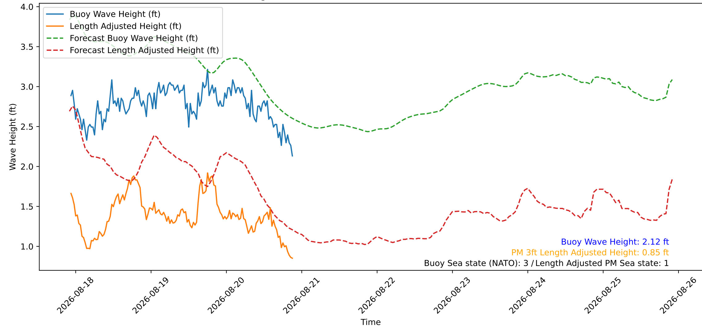
Wave Heights over Time for Red Beach at 2026-08-20 22:00:46
