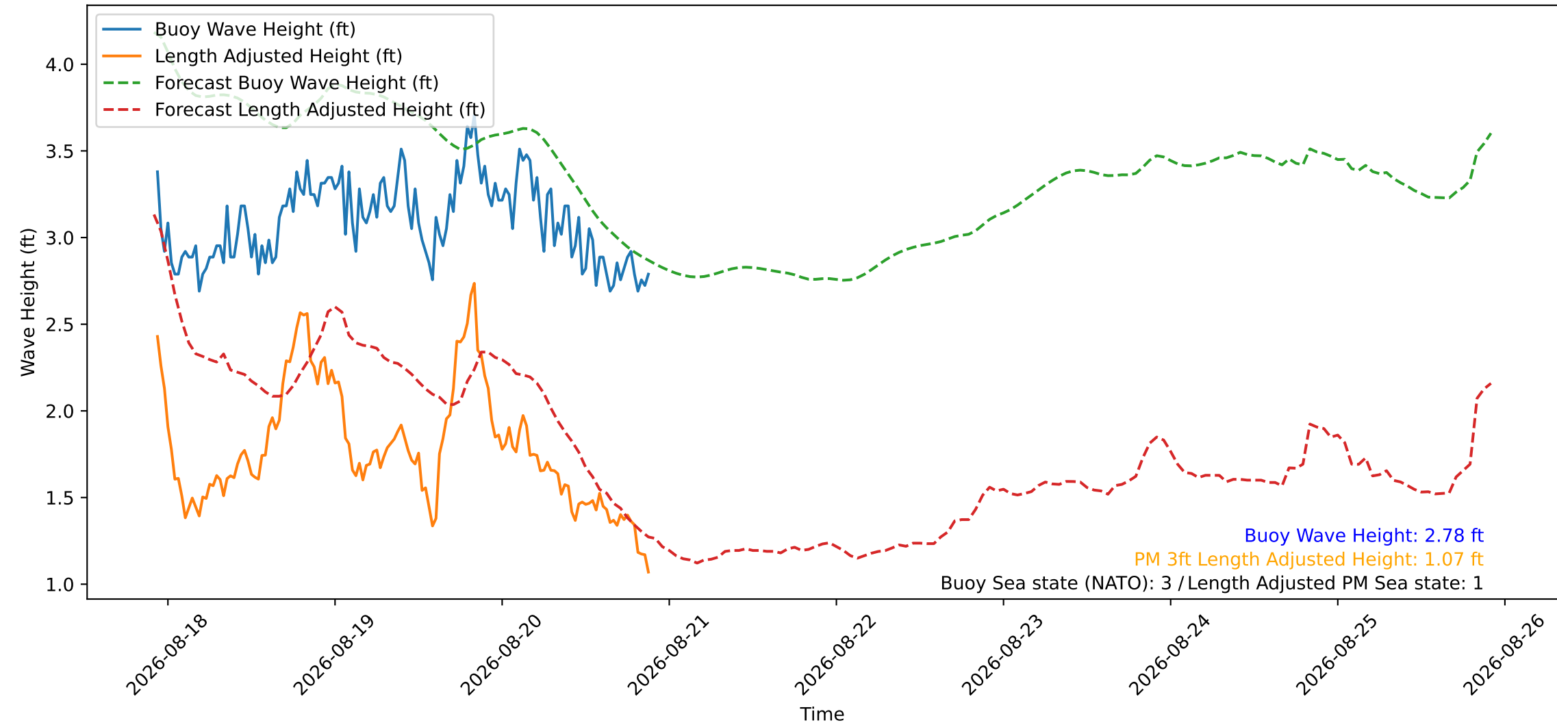
Wave Heights over Time for Green Beach at 2026-08-20 22:01:08
