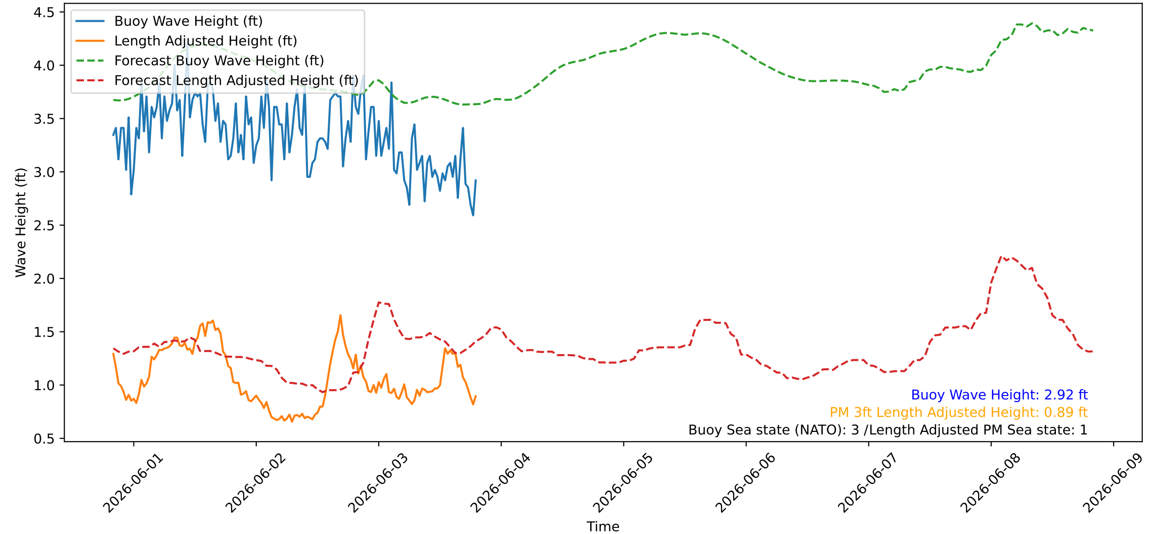
Wave Heights over Time for Red Beach at 2026-06-03 19:50:46
