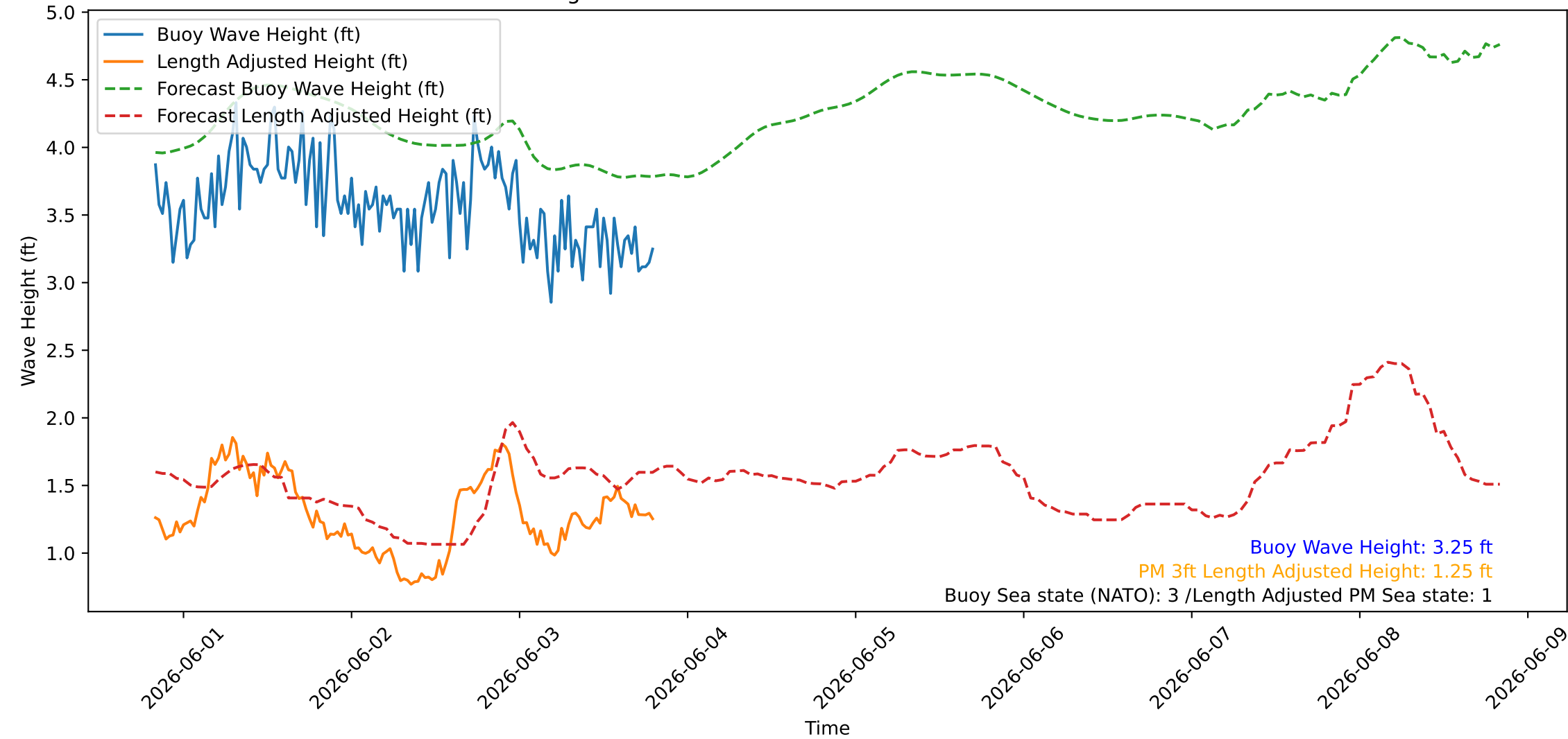
Wave Heights over Time for Green Beach at 2026-06-03 19:51:09
