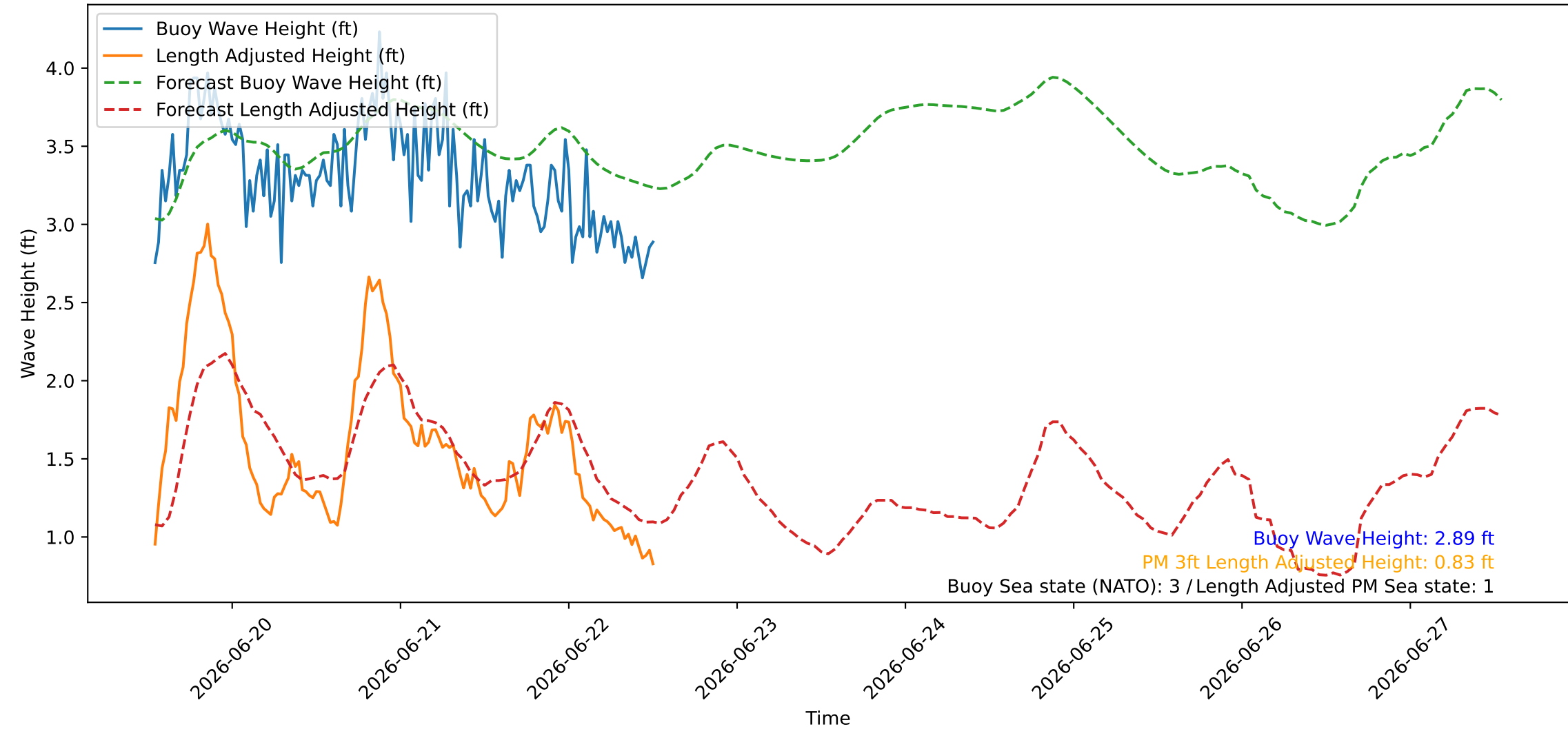
Wave Heights over Time for Green Beach at 2026-06-22 12:51:09
