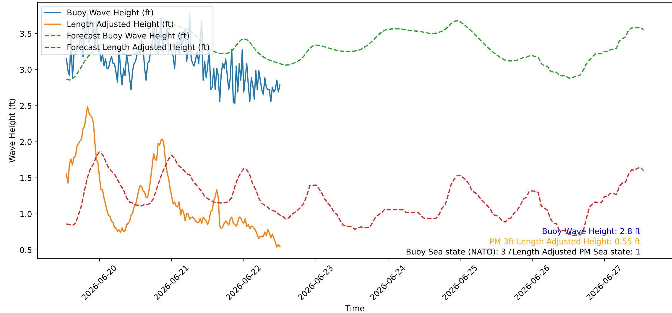
Wave Heights over Time for Red Beach at 2026-06-22 12:50:46
