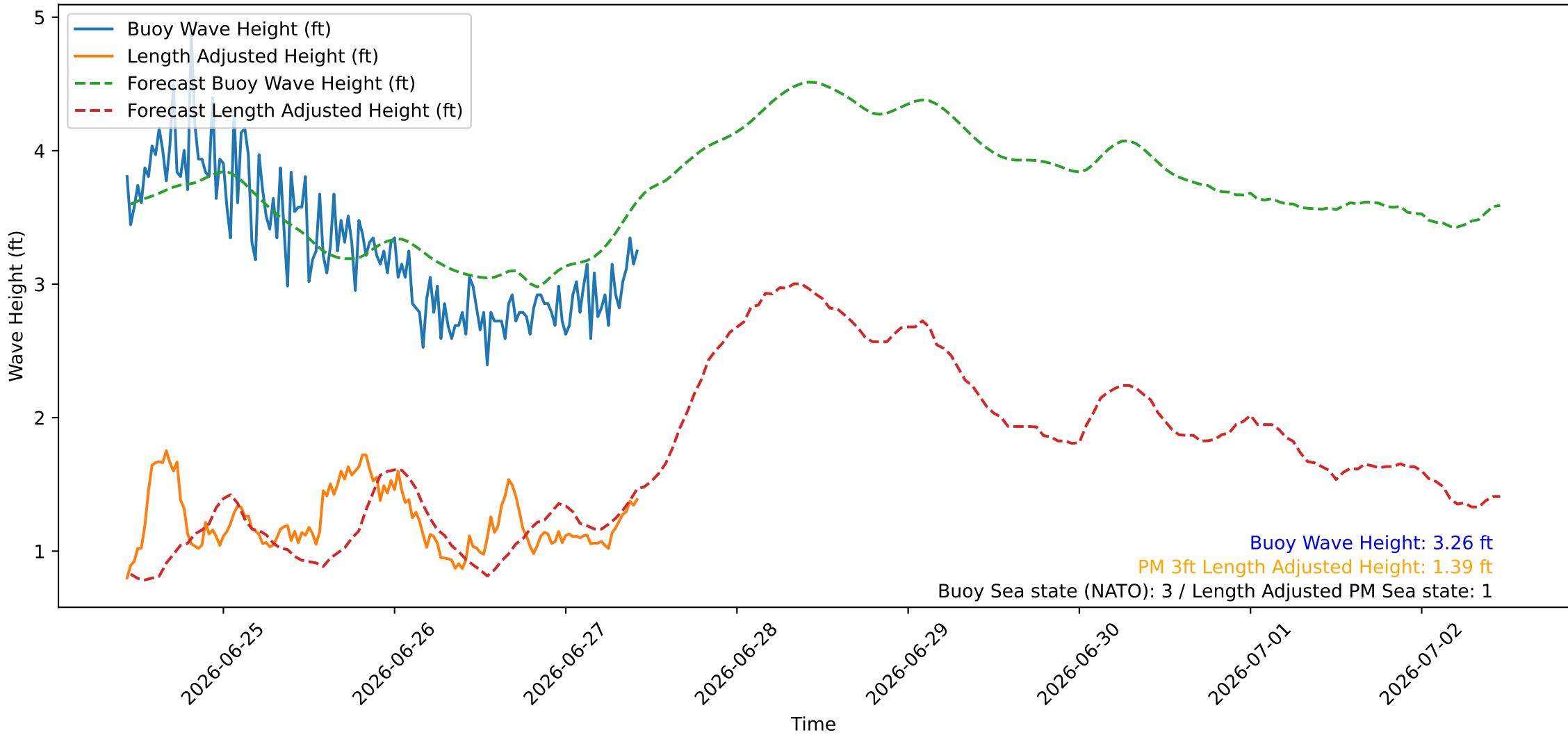
Wave Heights over Time for Oceanside Harbor at 2026-06-27 10:30:26
