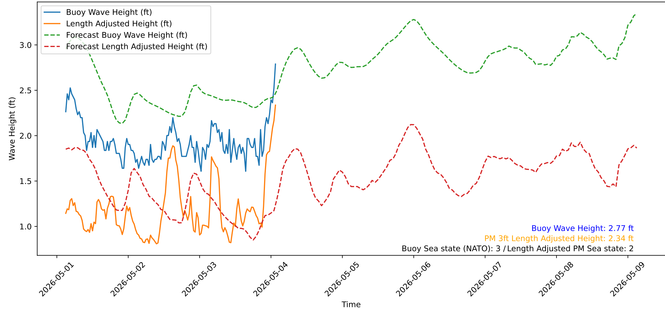
Wave Heights over Time for Red Beach at 2026-05-04 02:30:51
