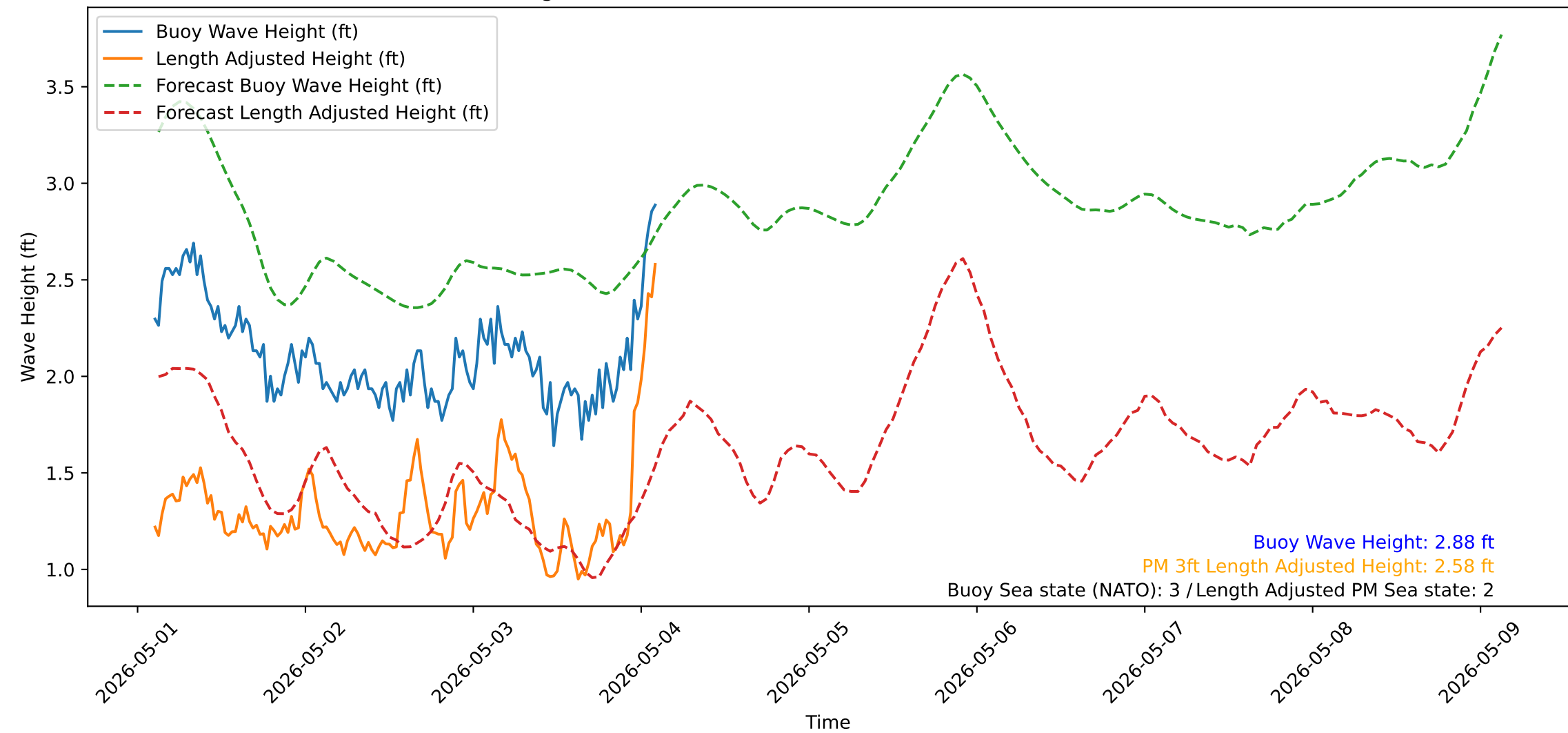
Wave Heights over Time for Oceanside Harbor at 2026-05-04 02:30:32
