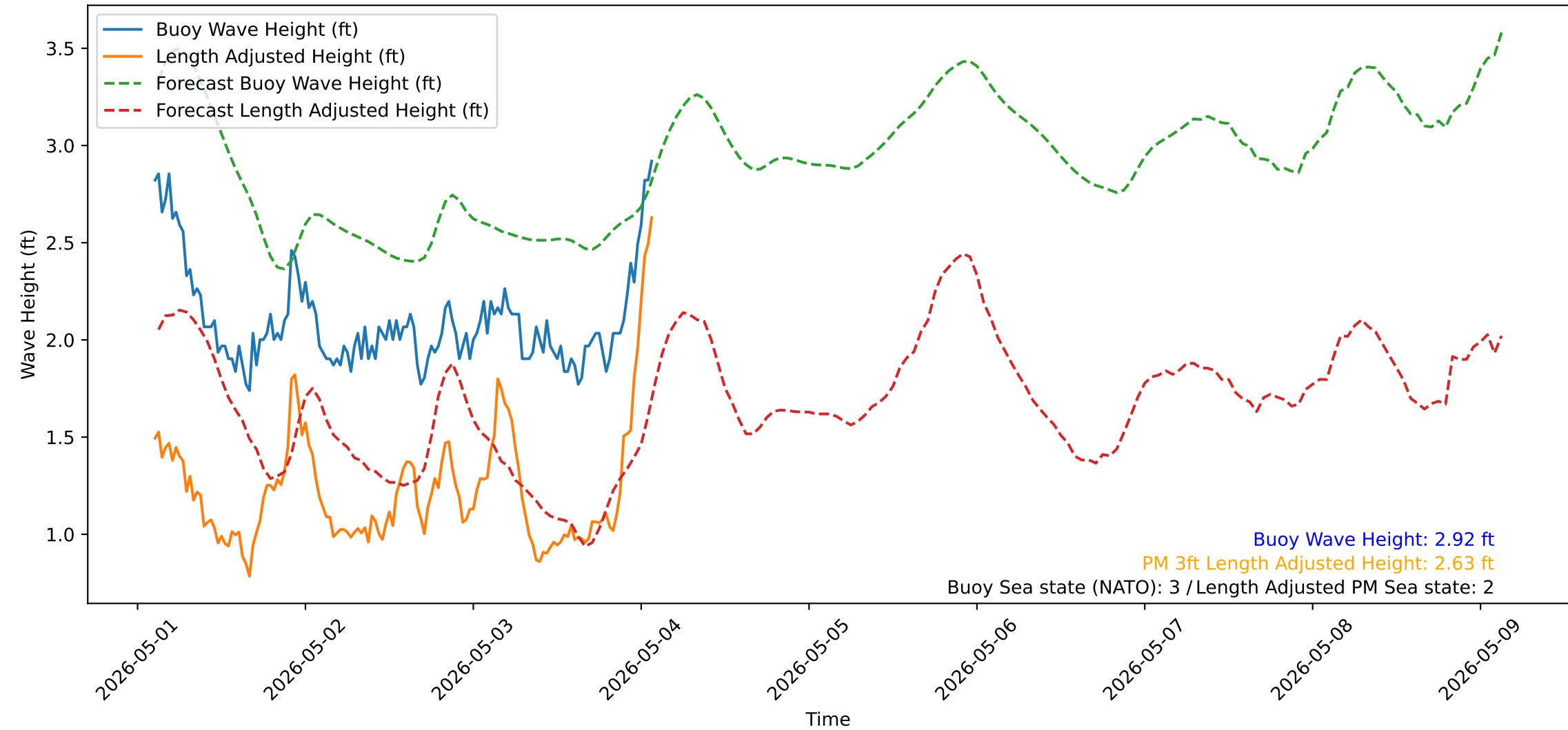
Wave Heights over Time for Green Beach at 2026-05-04 02:31:13
