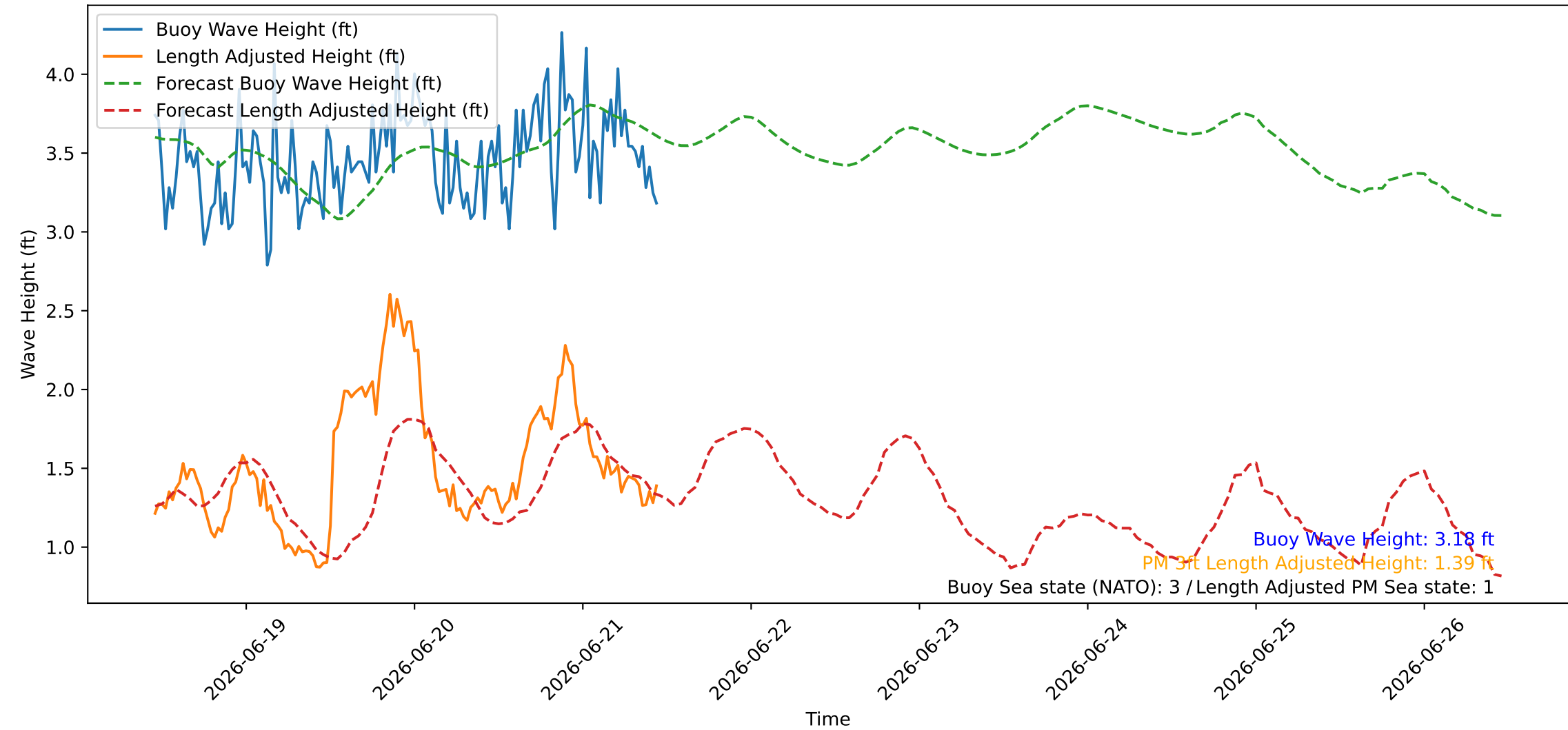
Wave Heights over Time for Oceanside Harbor at 2026-06-21 11:10:26
