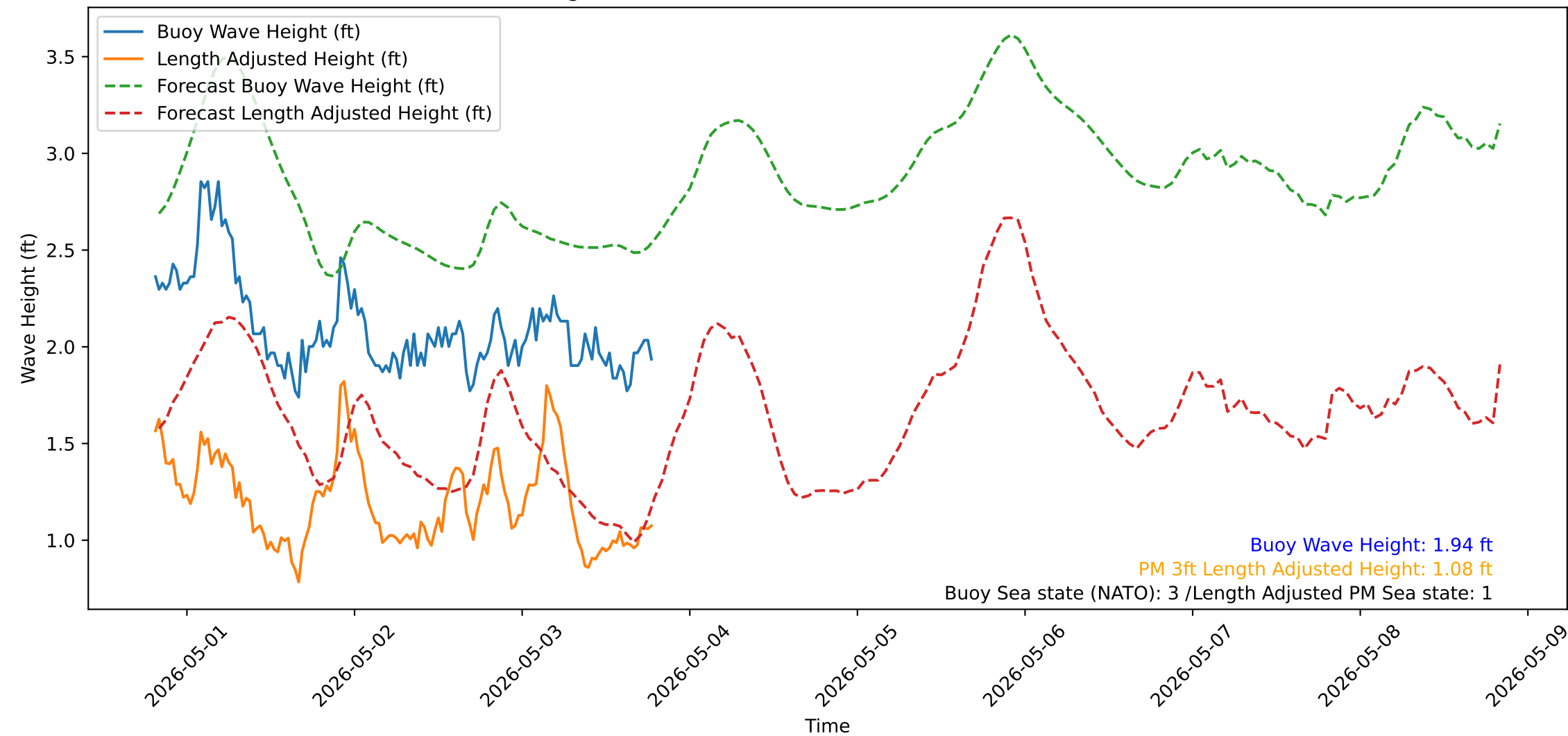
Wave Heights over Time for Green Beach at 2026-05-03 19:31:11
