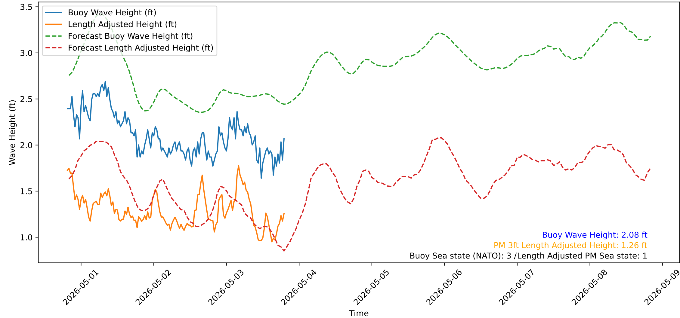
Wave Heights over Time for Oceanside Harbor at 2026-05-03 19:30:31
