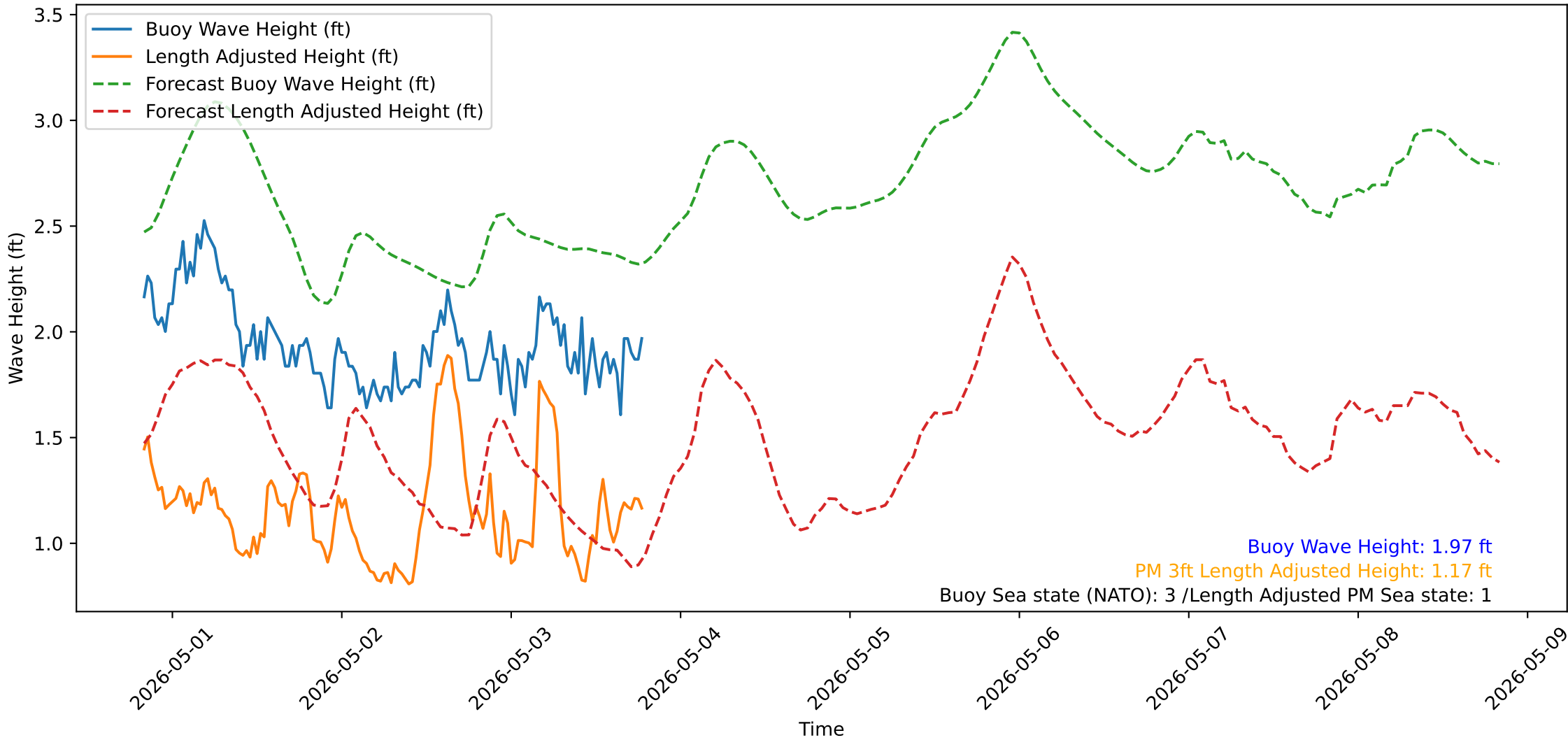
Wave Heights over Time for Red Beach at 2026-05-03 19:30:50
