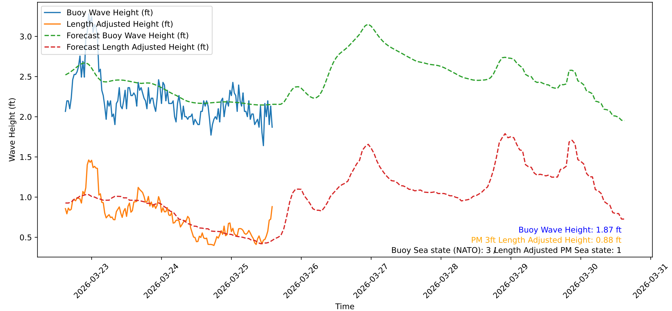
Wave Heights over Time for Green Beach at 2026-03-25 14:51:10
