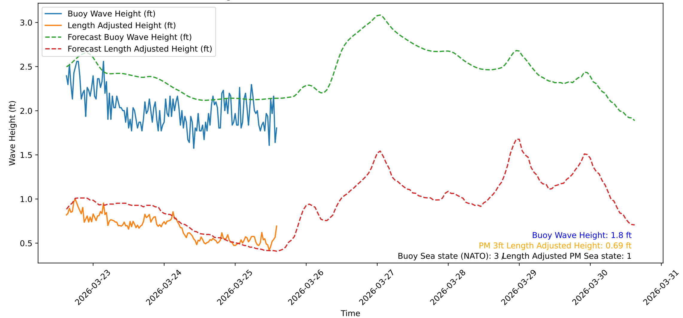
Wave Heights over Time for Oceanside Harbor at 2026-03-25 14:50:31
