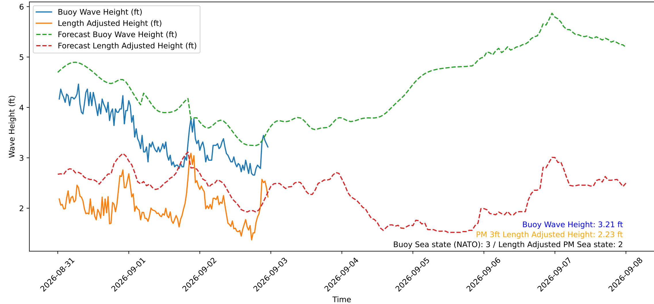
Wave Heights over Time for Green Beach at 2026-09-03 00:01:12
