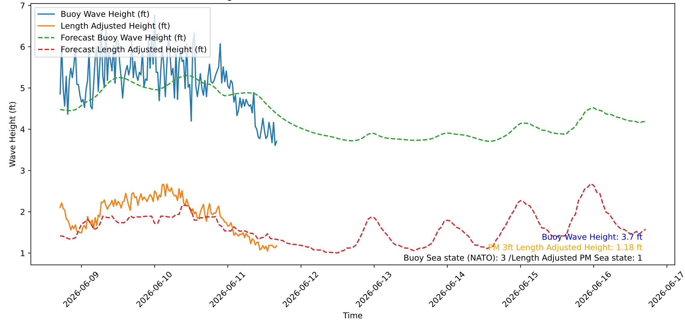
Wave Heights over Time for Oceanside Harbor at 2026-06-11 16:50:26
