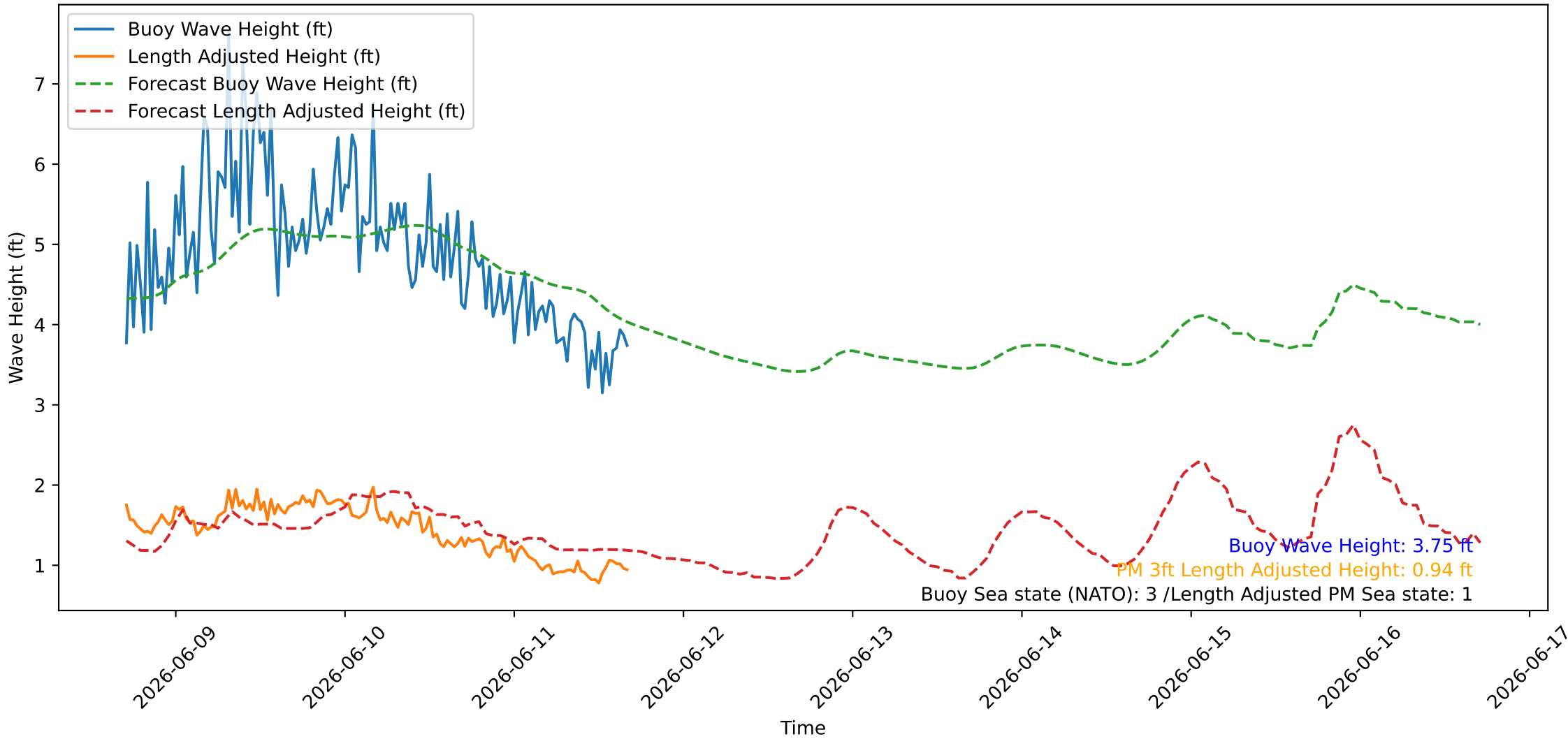
Wave Heights over Time for Red Beach at 2026-06-11 16:50:47
