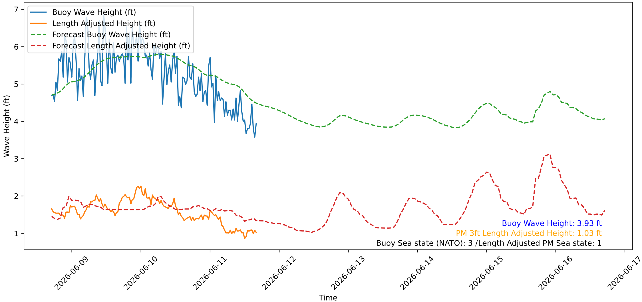
Wave Heights over Time for Green Beach at 2026-06-11 16:51:10
