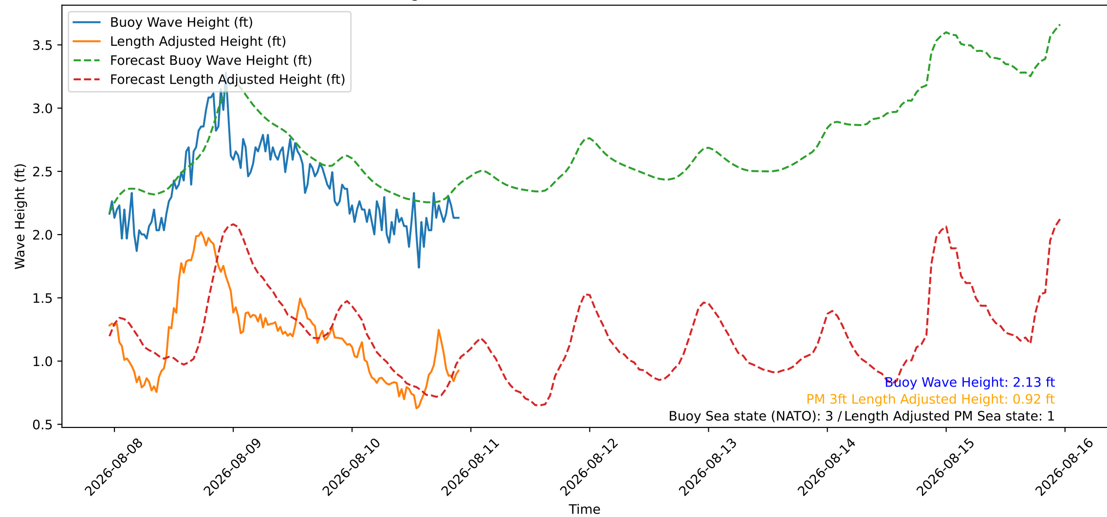
Wave Heights over Time for Red Beach at 2026-08-10 22:30:46
