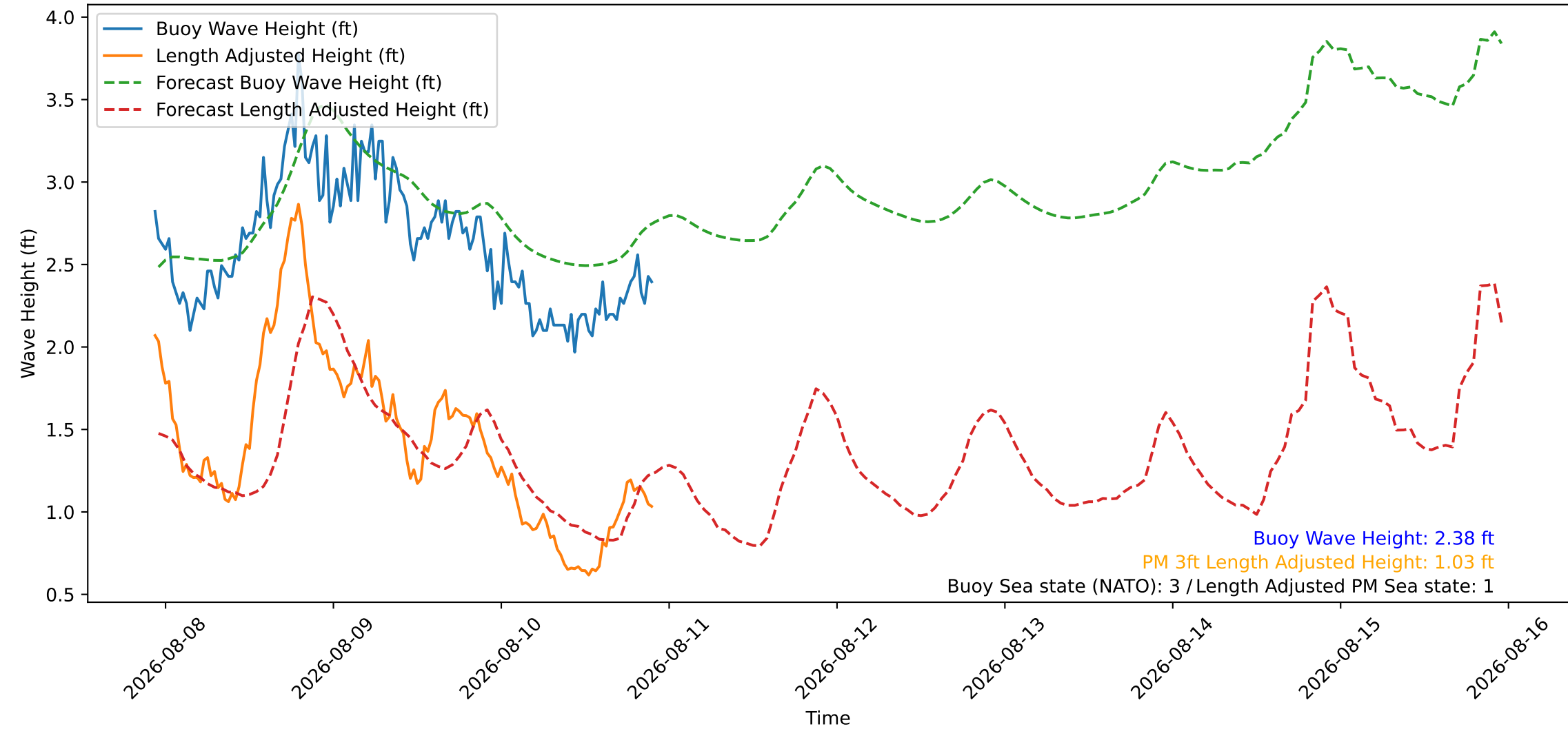
Wave Heights over Time for Green Beach at 2026-08-10 22:31:08
