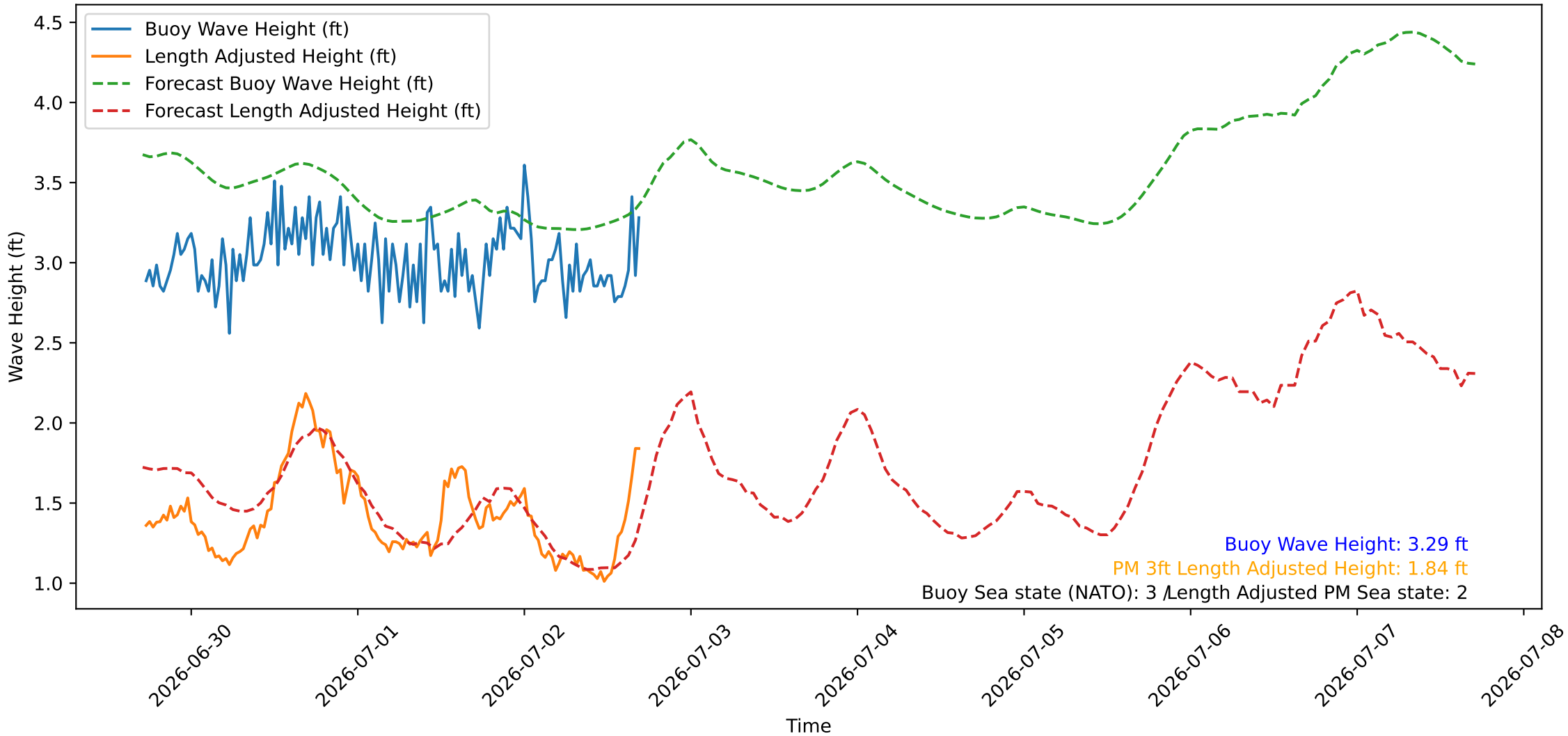
Wave Heights over Time for Oceanside Harbor at 2026-07-02 17:20:26
