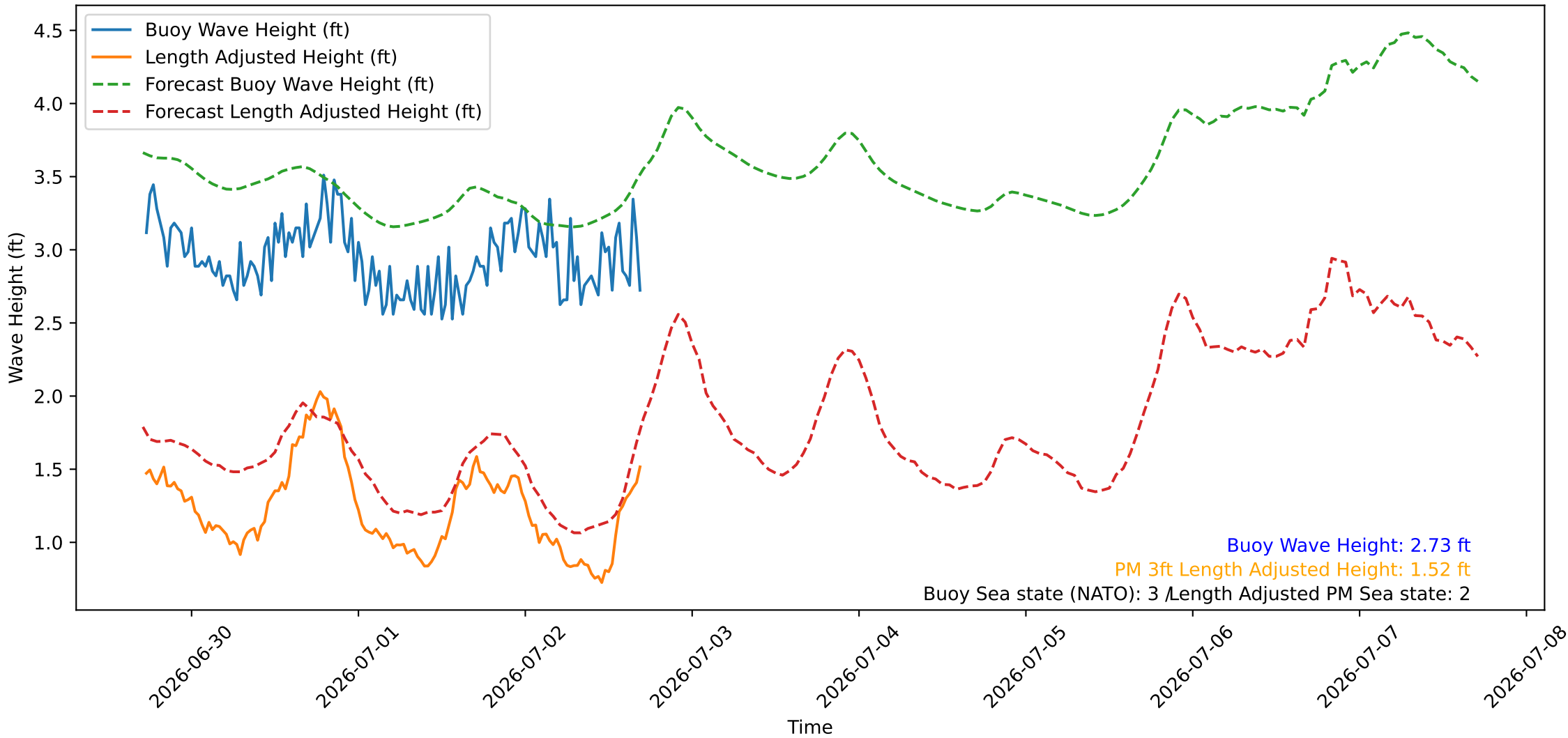
Wave Heights over Time for Green Beach at 2026-07-02 17:21:09
