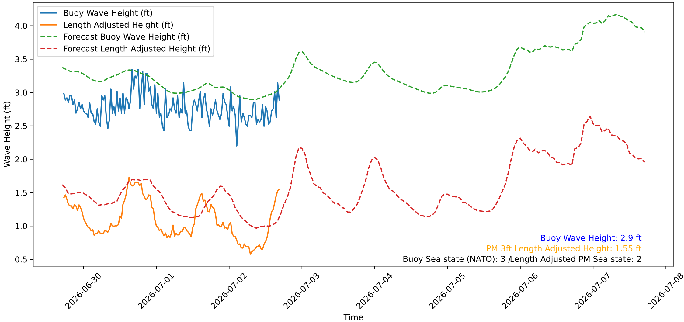
Wave Heights over Time for Red Beach at 2026-07-02 17:20:47
