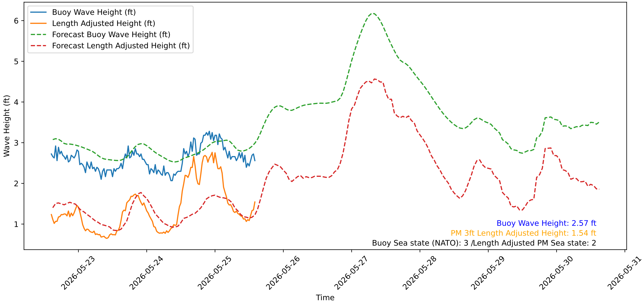
Wave Heights over Time for Green Beach at 2026-05-25 14:41:12
