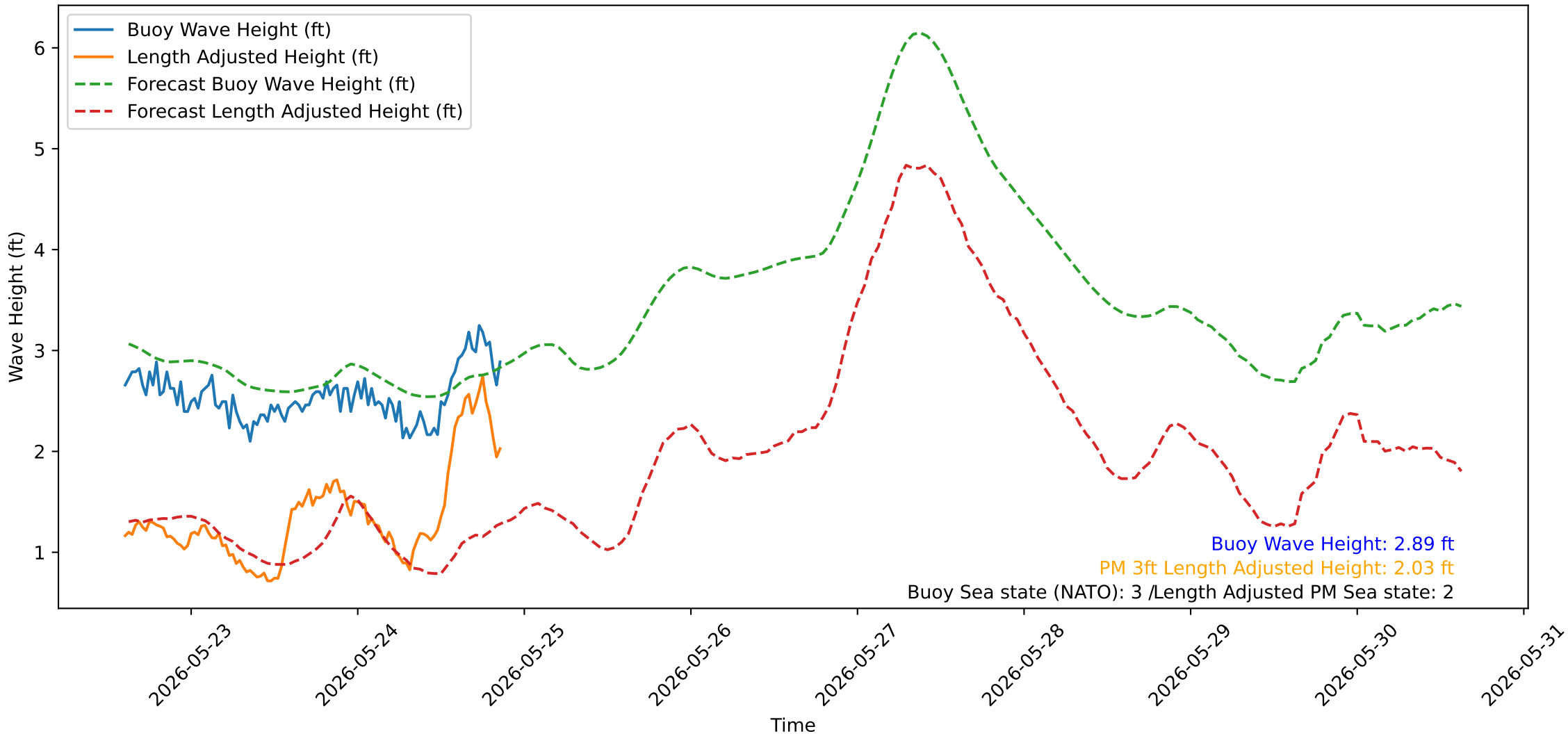
Wave Heights over Time for Oceanside Harbor at 2026-05-25 14:40:30
