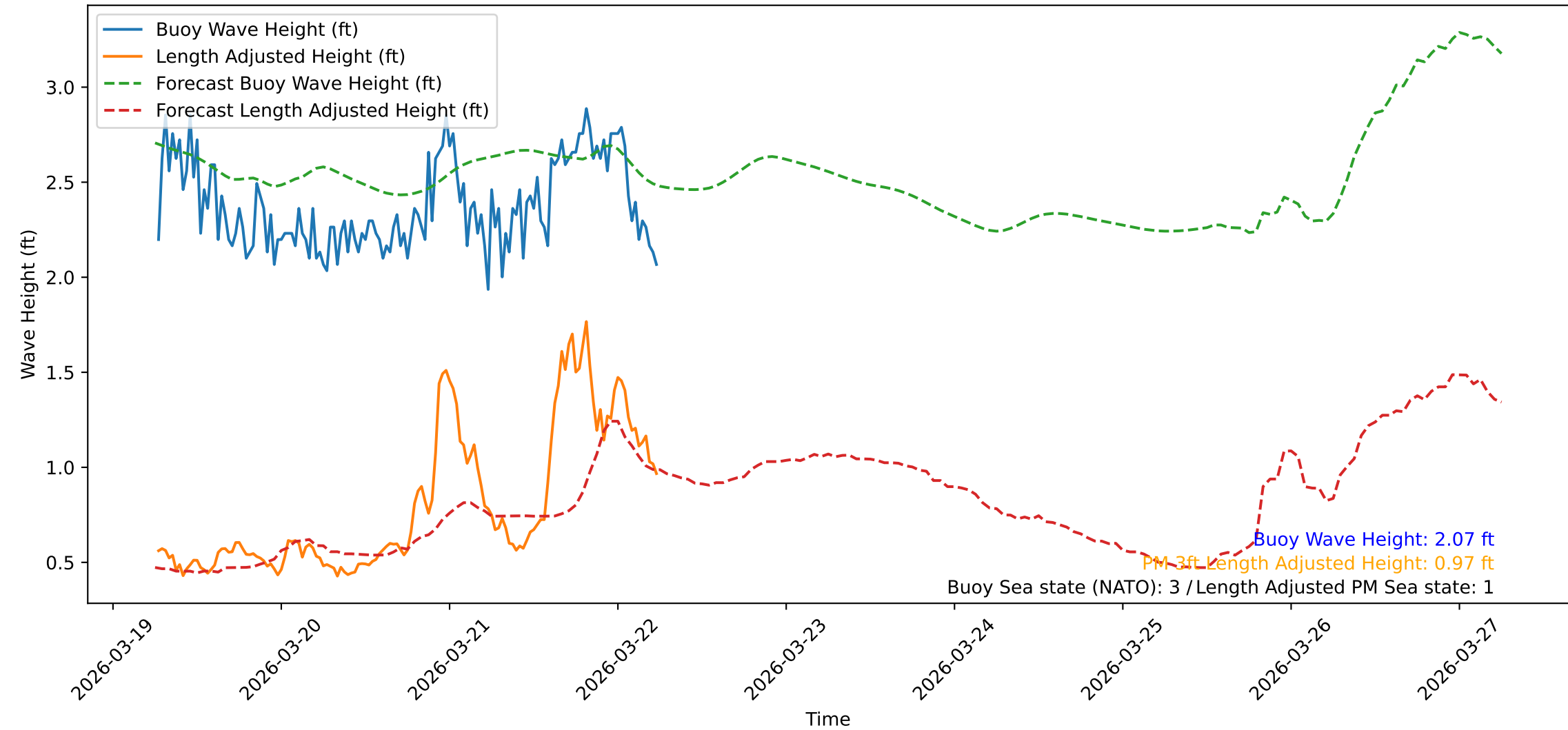
Wave Heights over Time for Green Beach at 2026-03-22 06:21:10
