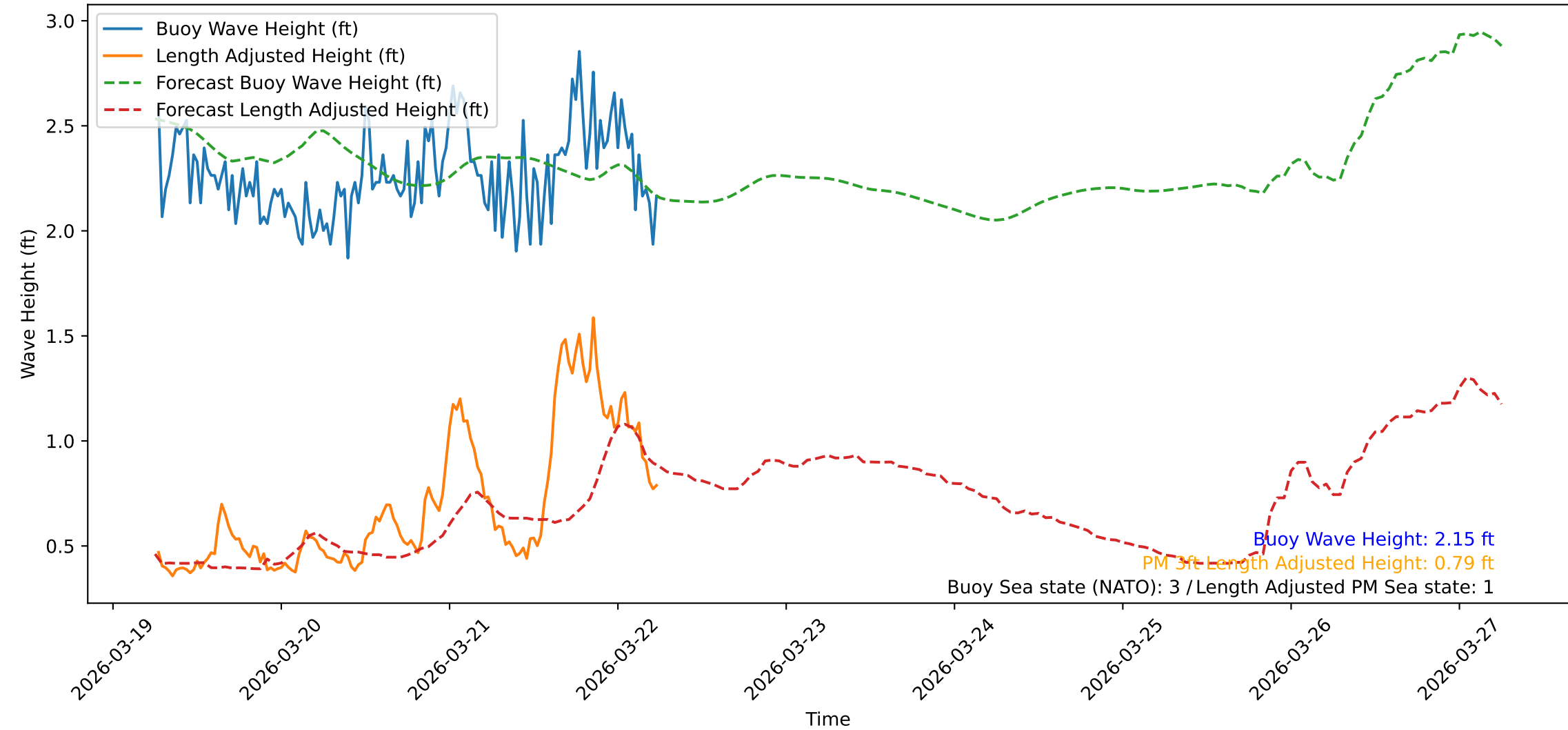
Wave Heights over Time for Red Beach at 2026-03-22 06:20:48
