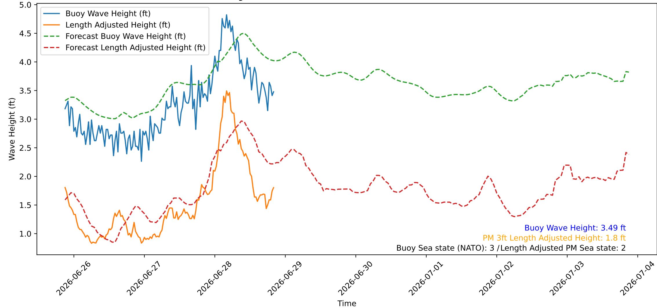
Wave Heights over Time for Green Beach at 2026-06-28 20:51:09
