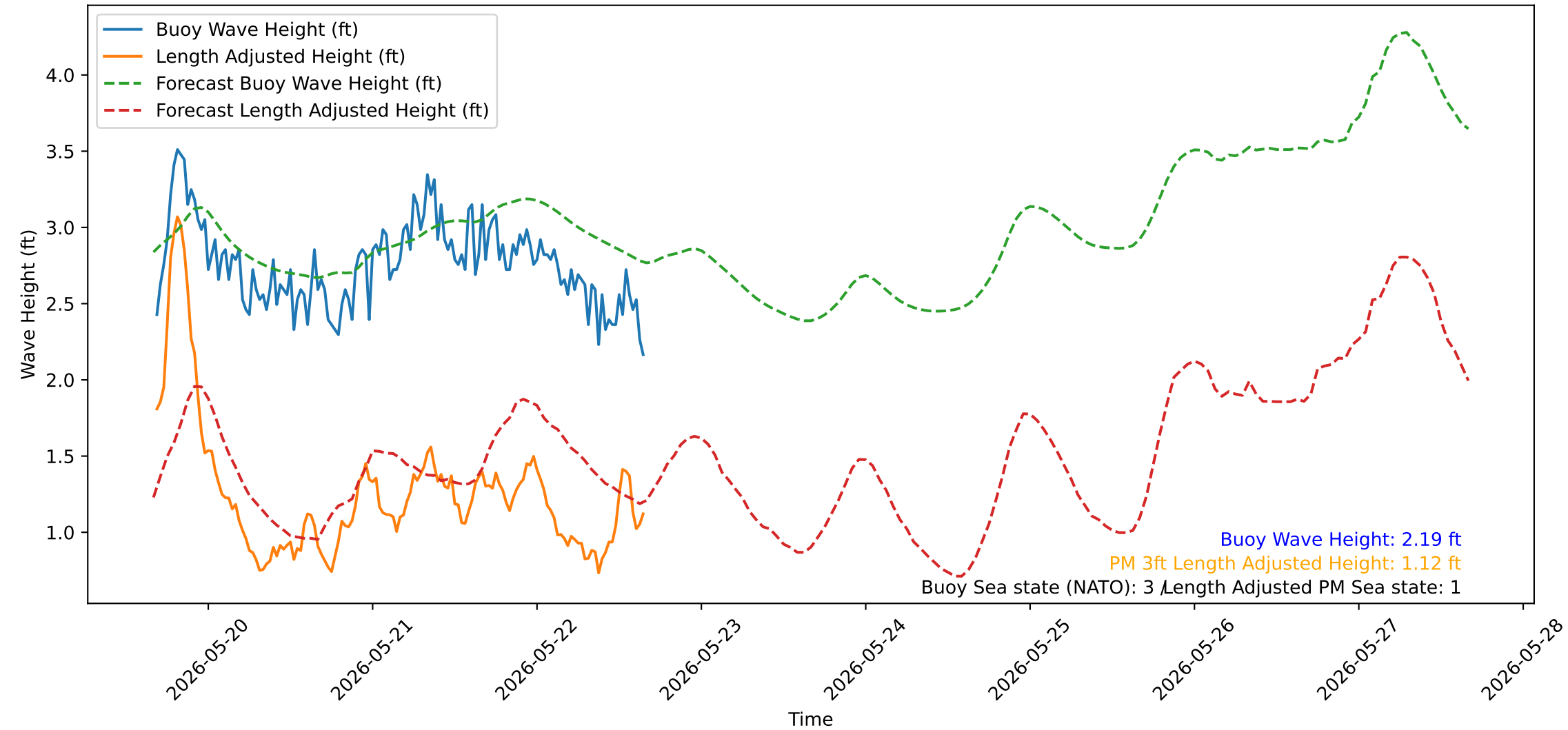
Wave Heights over Time for Red Beach at 2026-05-22 16:10:51
