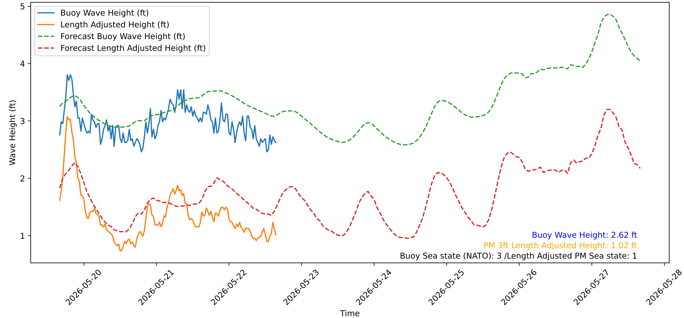
Wave Heights over Time for Green Beach at 2026-05-22 16:11:13
