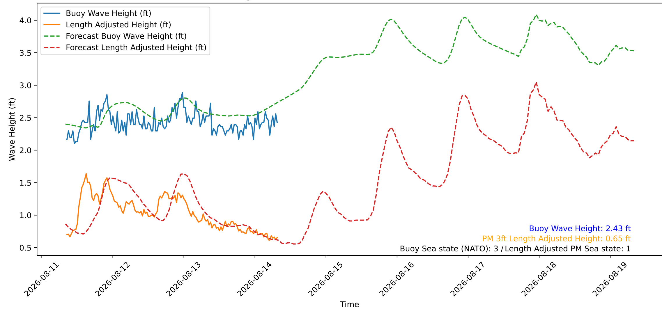
Wave Heights over Time for Red Beach at 2026-08-14 08:10:46
