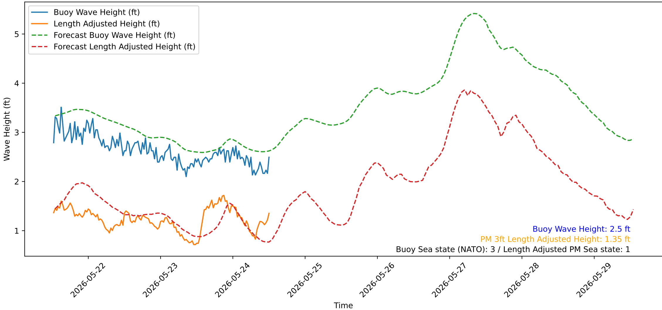
Wave Heights over Time for Oceanside Harbor at 2026-05-24 12:40:32
