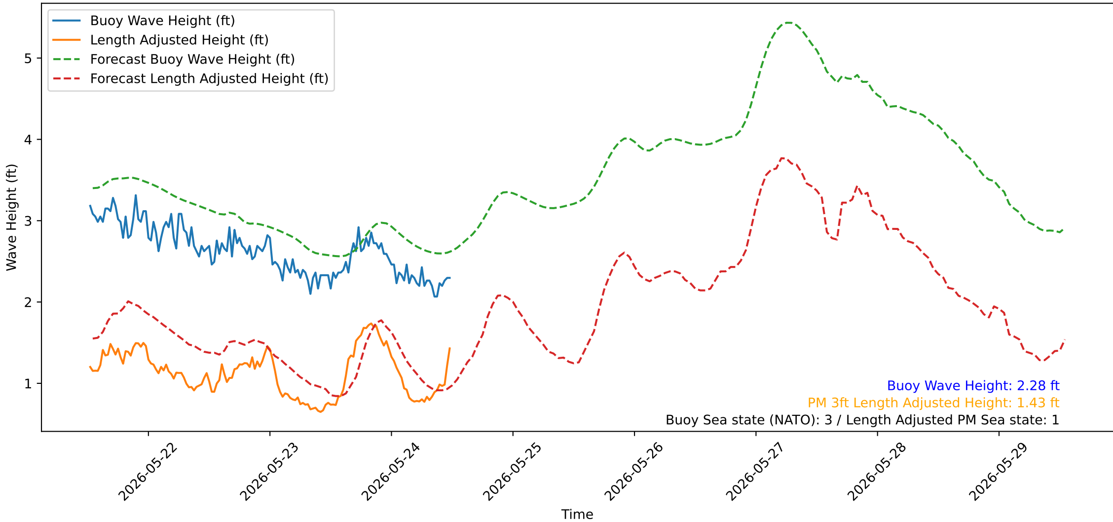
Wave Heights over Time for Green Beach at 2026-05-24 12:41:15
