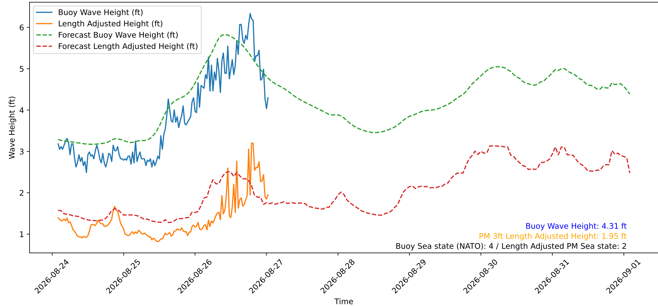
Wave Heights over Time for Green Beach at 2026-08-27 01:31:10
