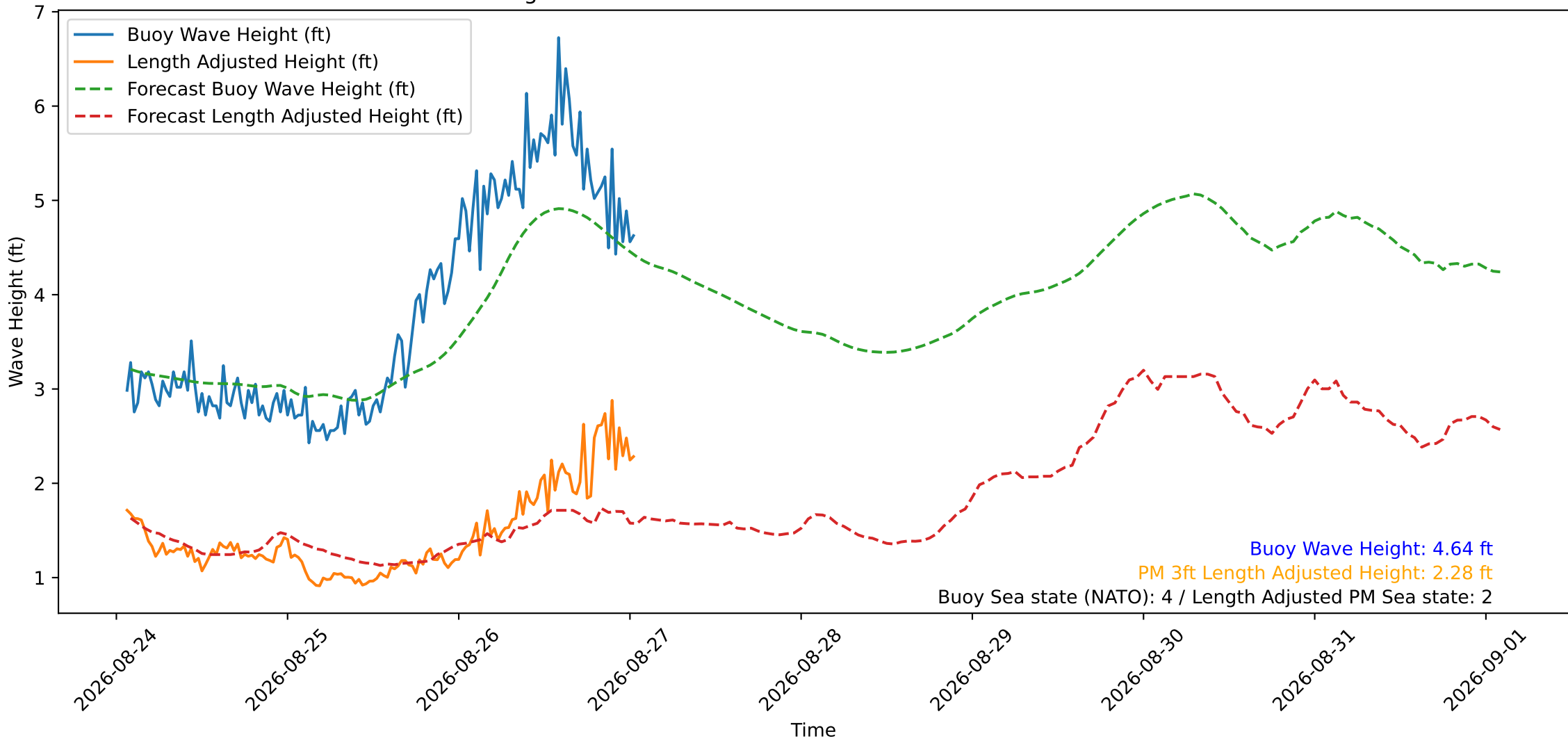
Wave Heights over Time for Oceanside Harbor at 2026-08-27 01:30:29
