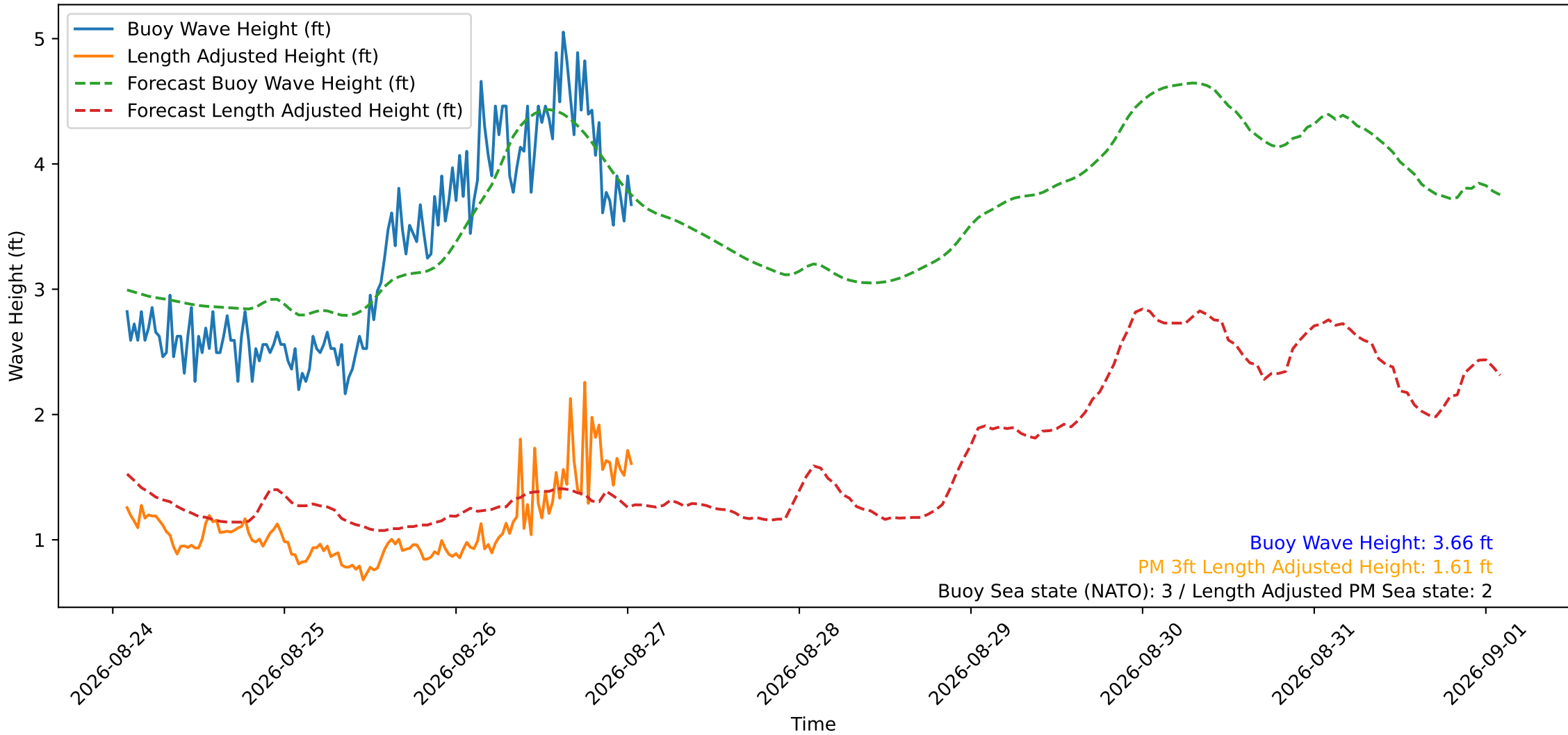
Wave Heights over Time for Red Beach at 2026-08-27 01:30:48
