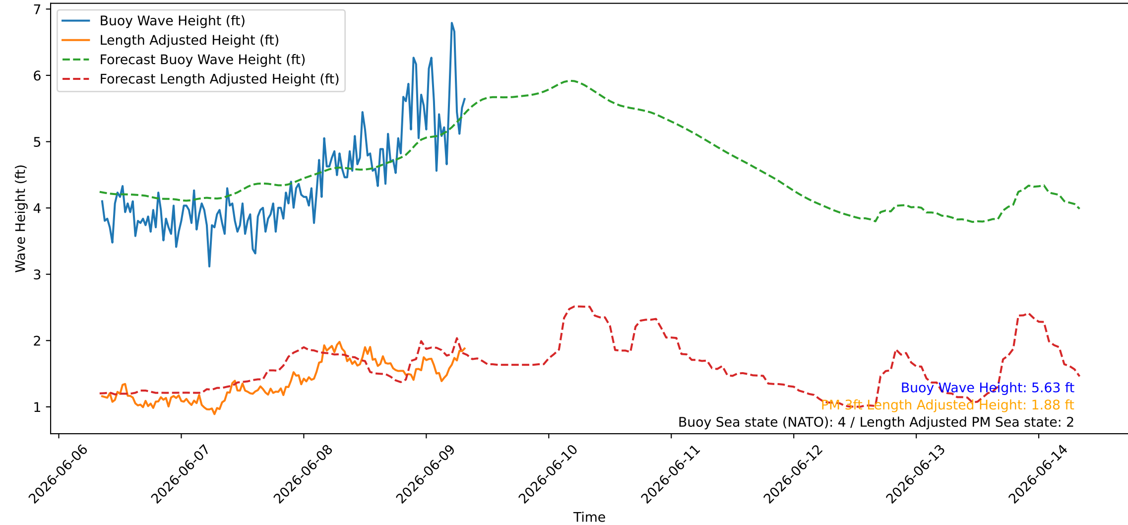
Wave Heights over Time for Green Beach at 2026-06-09 08:21:09
