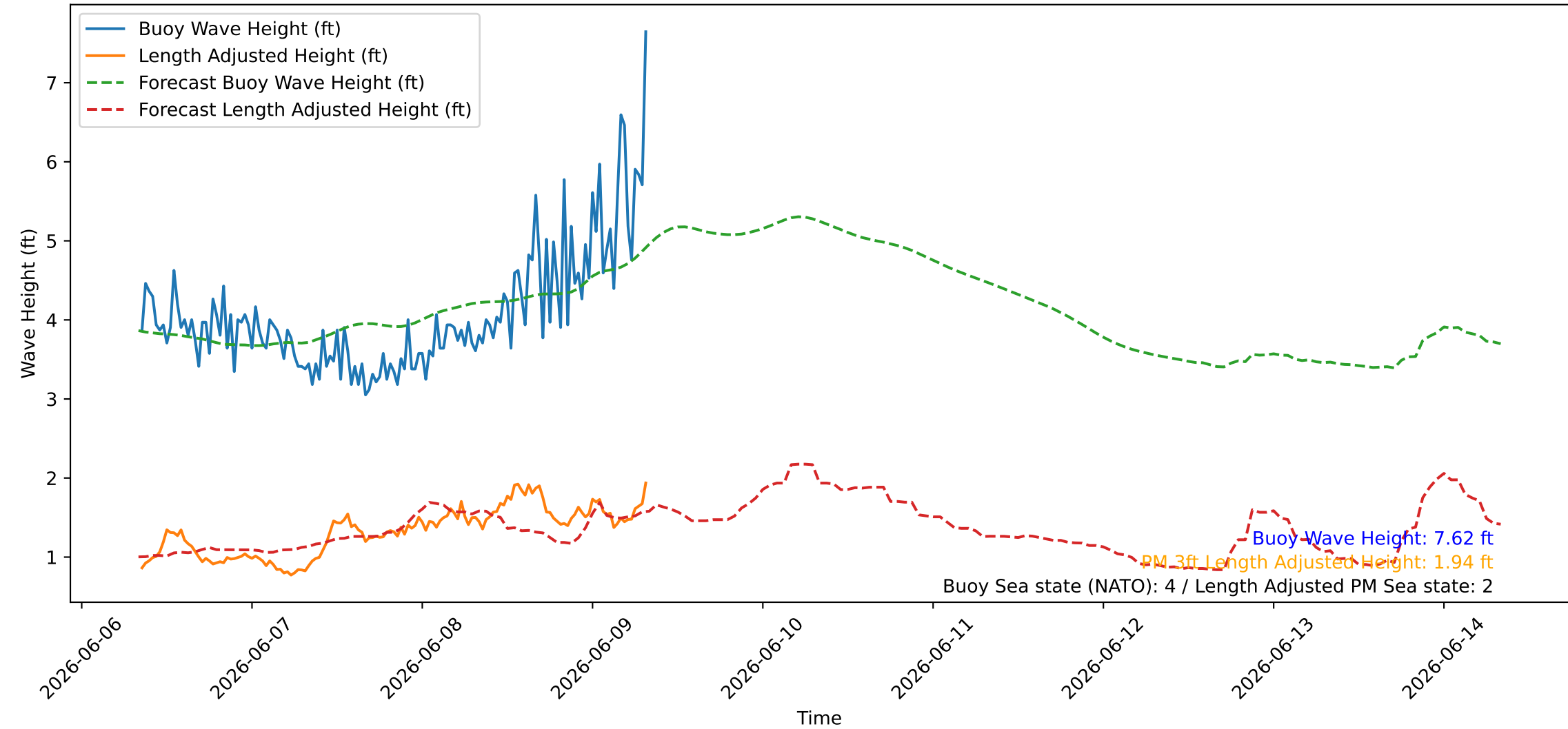
Wave Heights over Time for Red Beach at 2026-06-09 08:20:47
