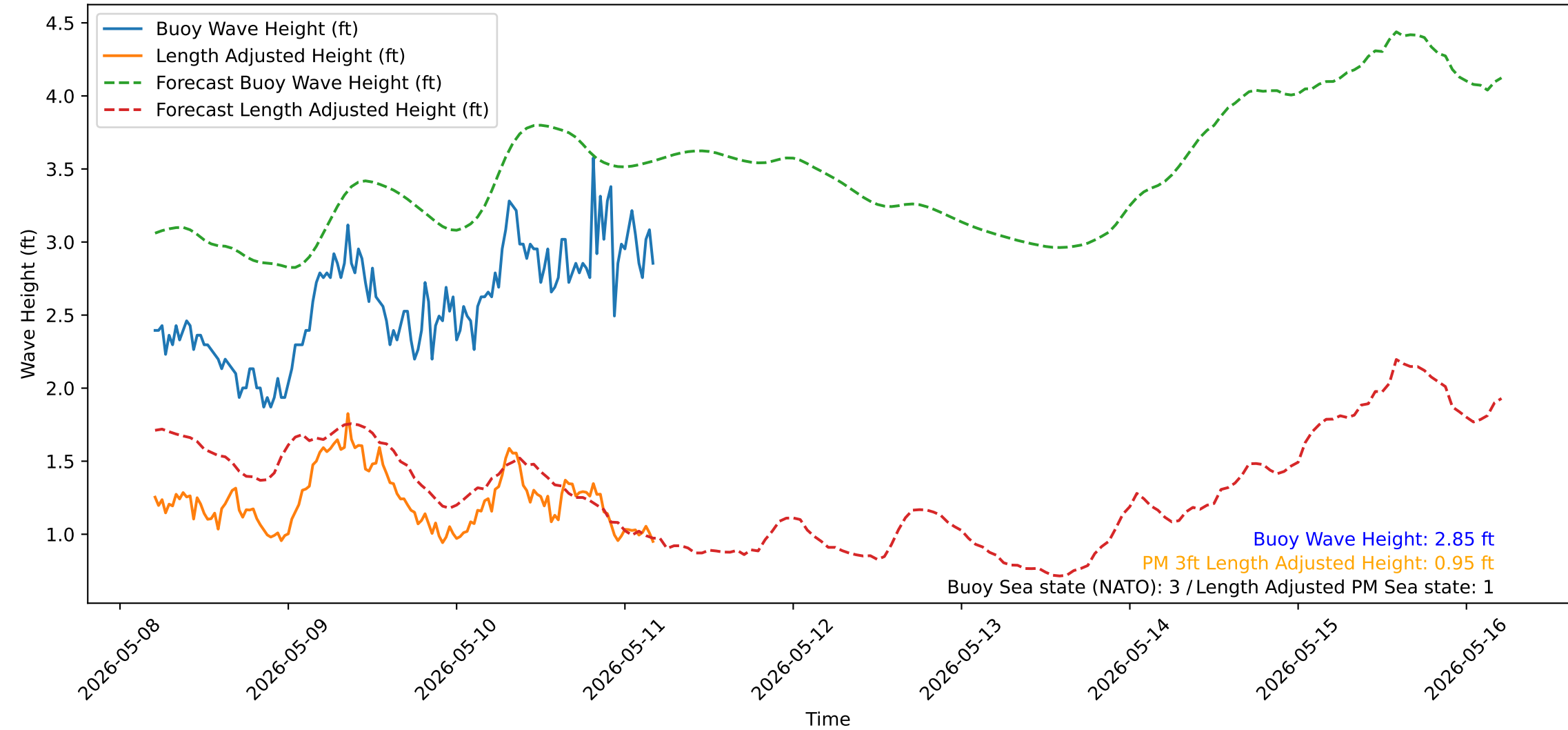
Wave Heights over Time for Oceanside Harbor at 2026-05-11 05:00:30
