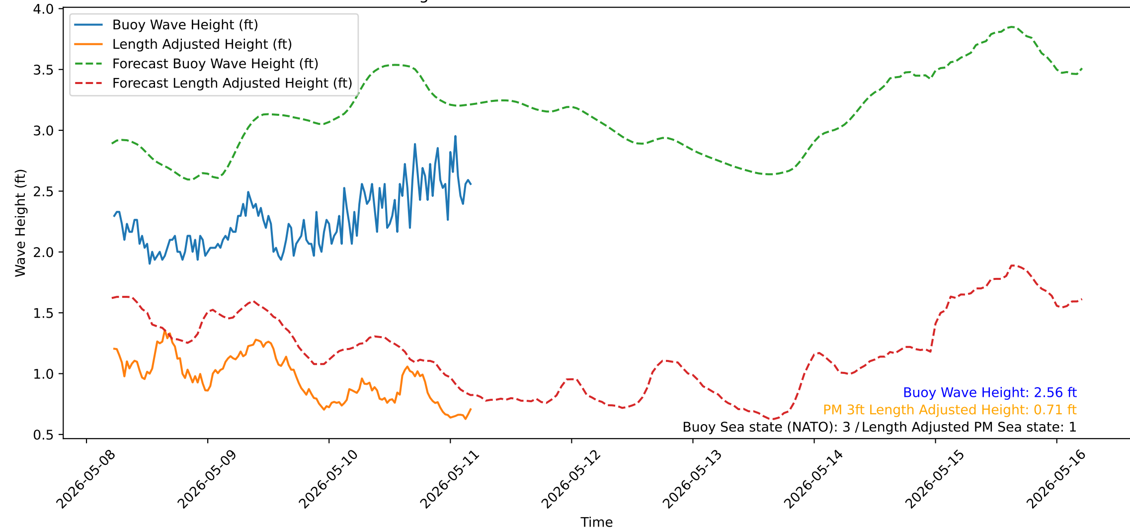
Wave Heights over Time for Red Beach at 2026-05-11 05:00:49
