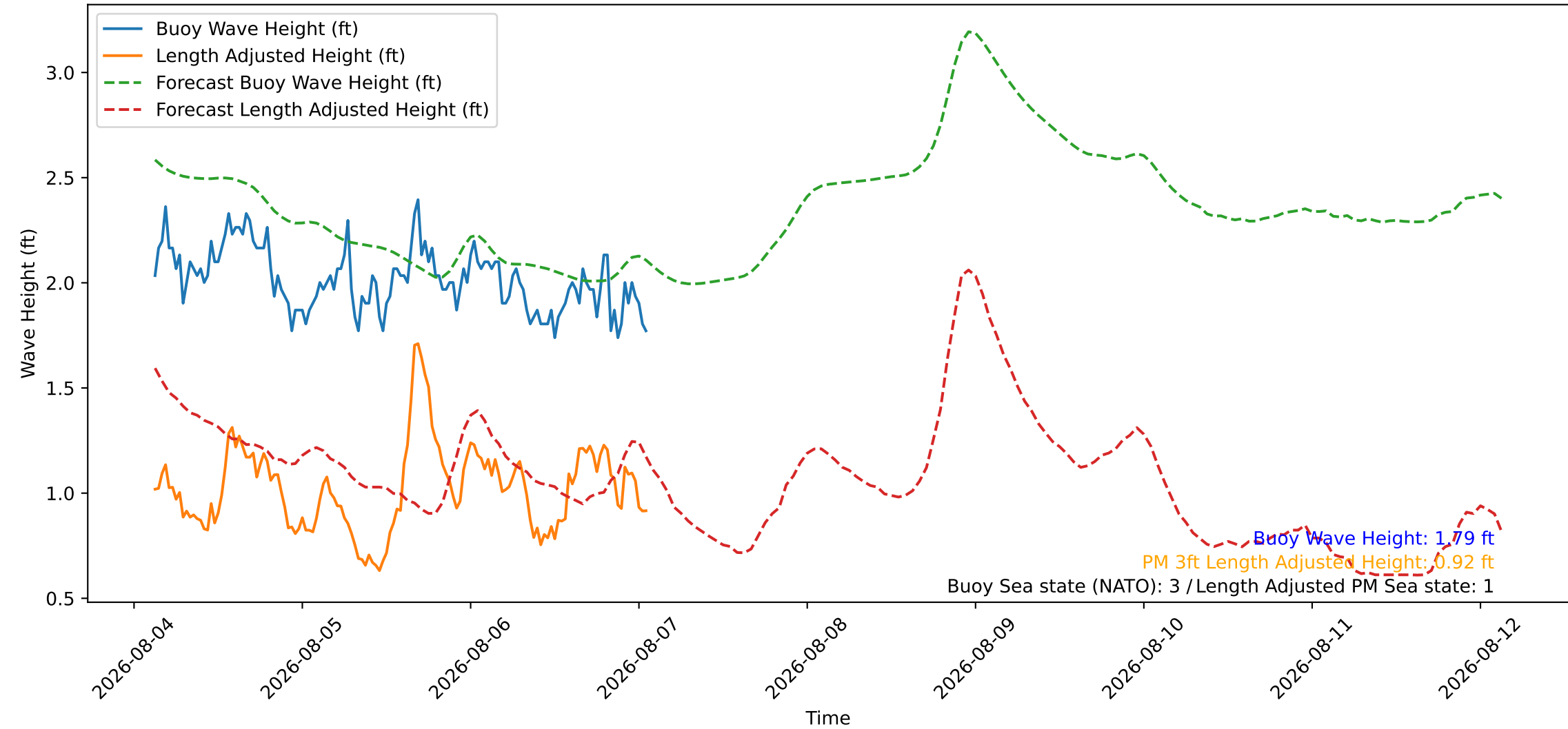
Wave Heights over Time for Red Beach at 2026-08-07 02:30:45
