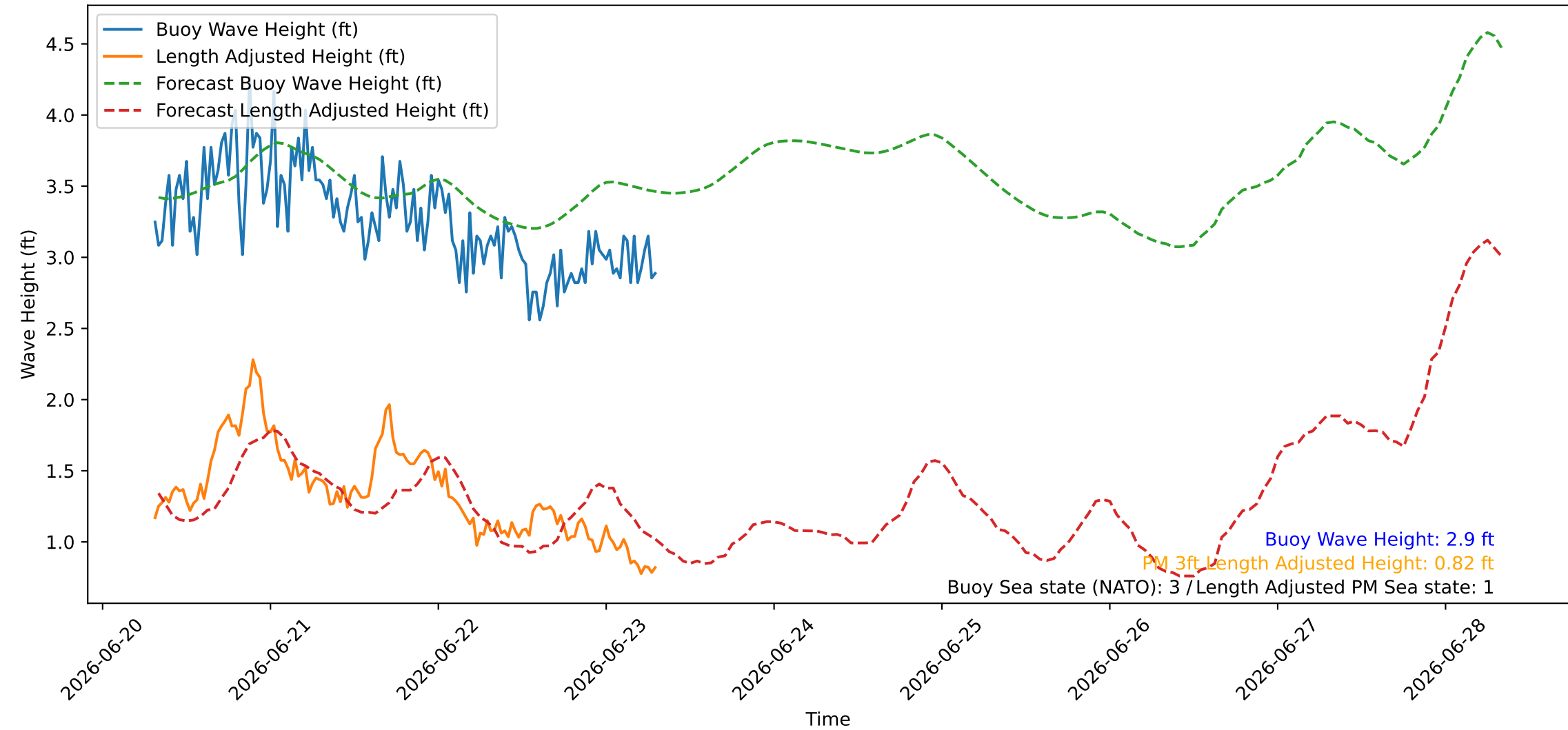
Wave Heights over Time for Oceanside Harbor at 2026-06-23 07:40:26
