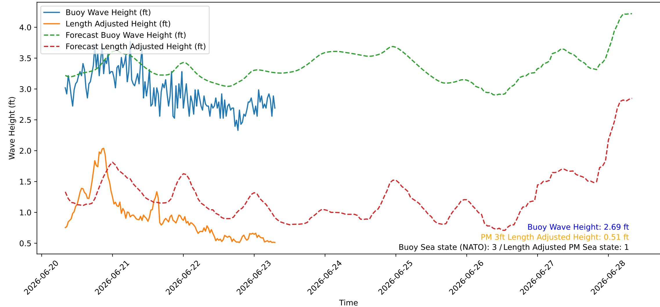
Wave Heights over Time for Red Beach at 2026-06-23 07:40:45
