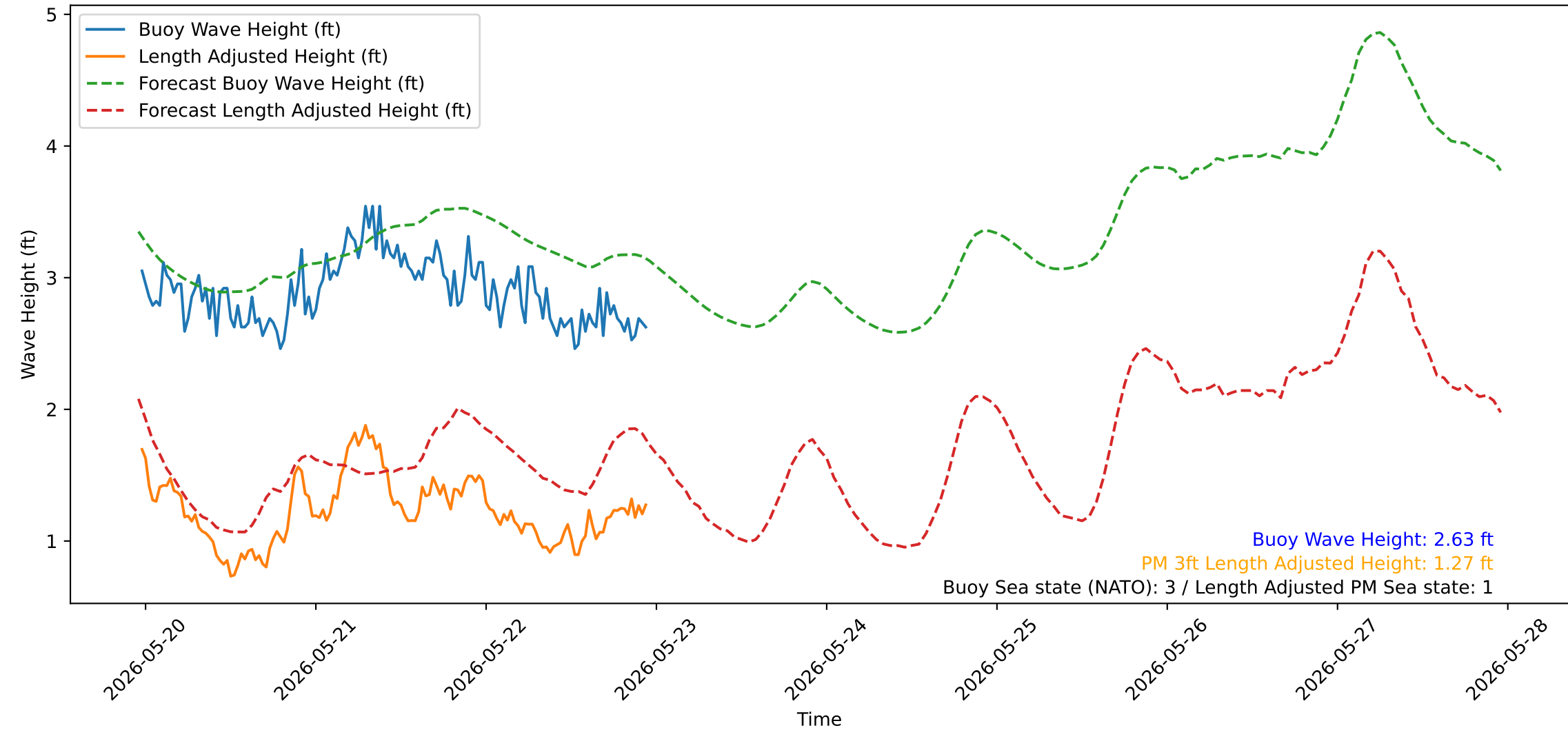
Wave Heights over Time for Green Beach at 2026-05-22 23:21:15
