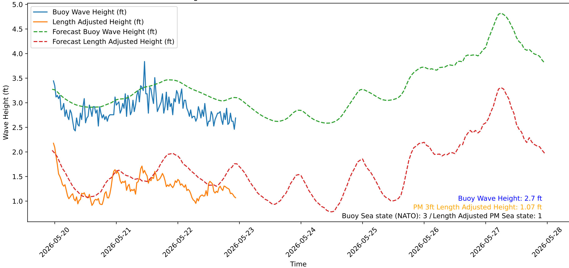
Wave Heights over Time for Oceanside Harbor at 2026-05-22 23:20:32
