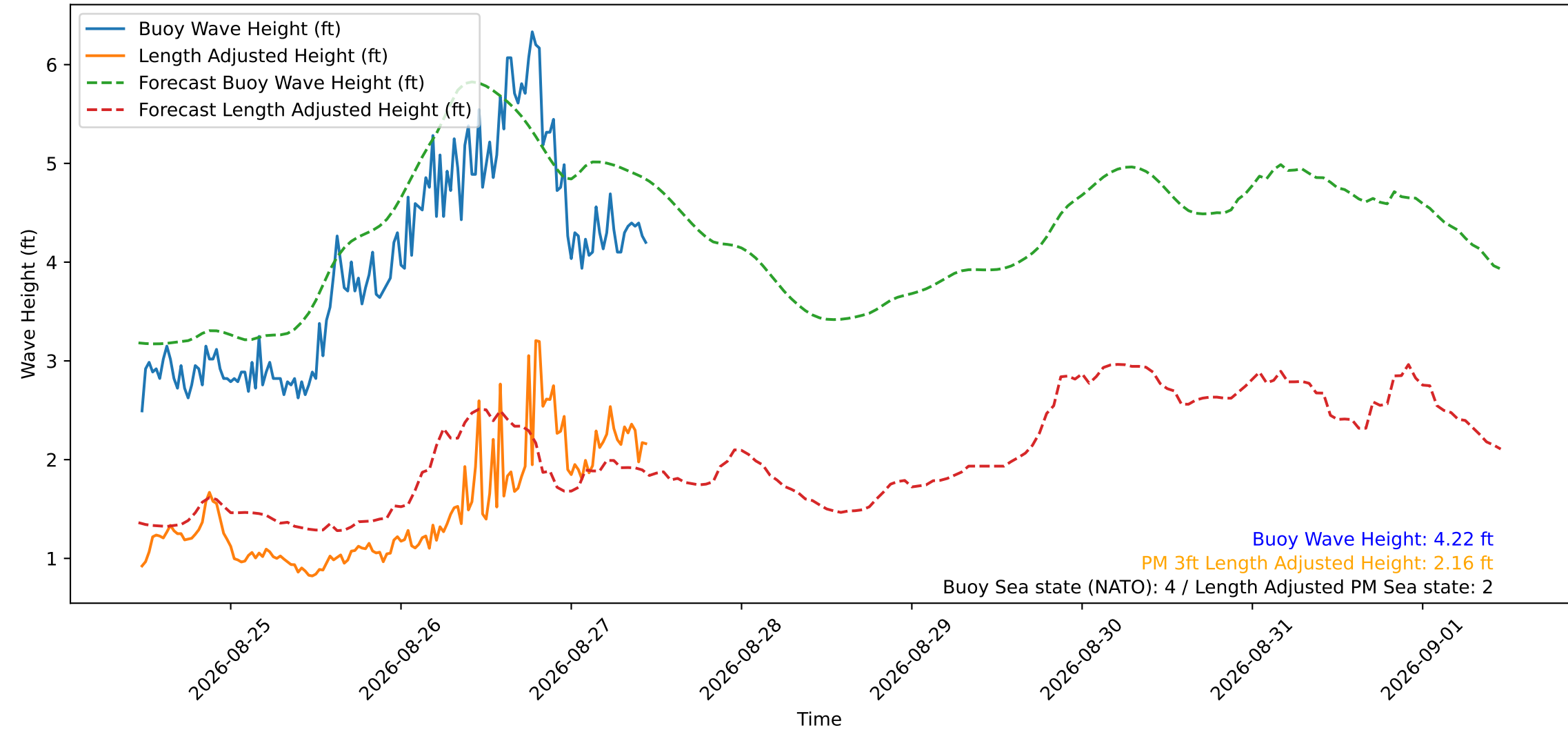
Wave Heights over Time for Green Beach at 2026-08-27 11:11:12
