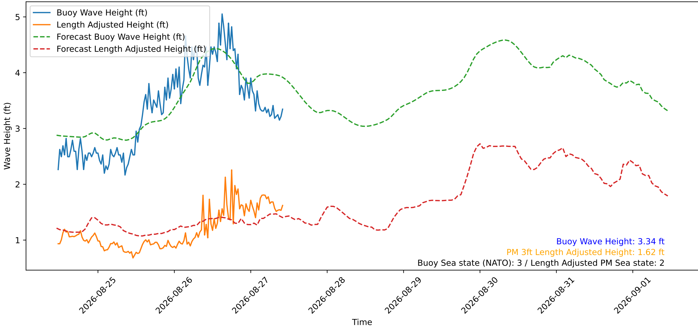
Wave Heights over Time for Red Beach at 2026-08-27 11:10:50
