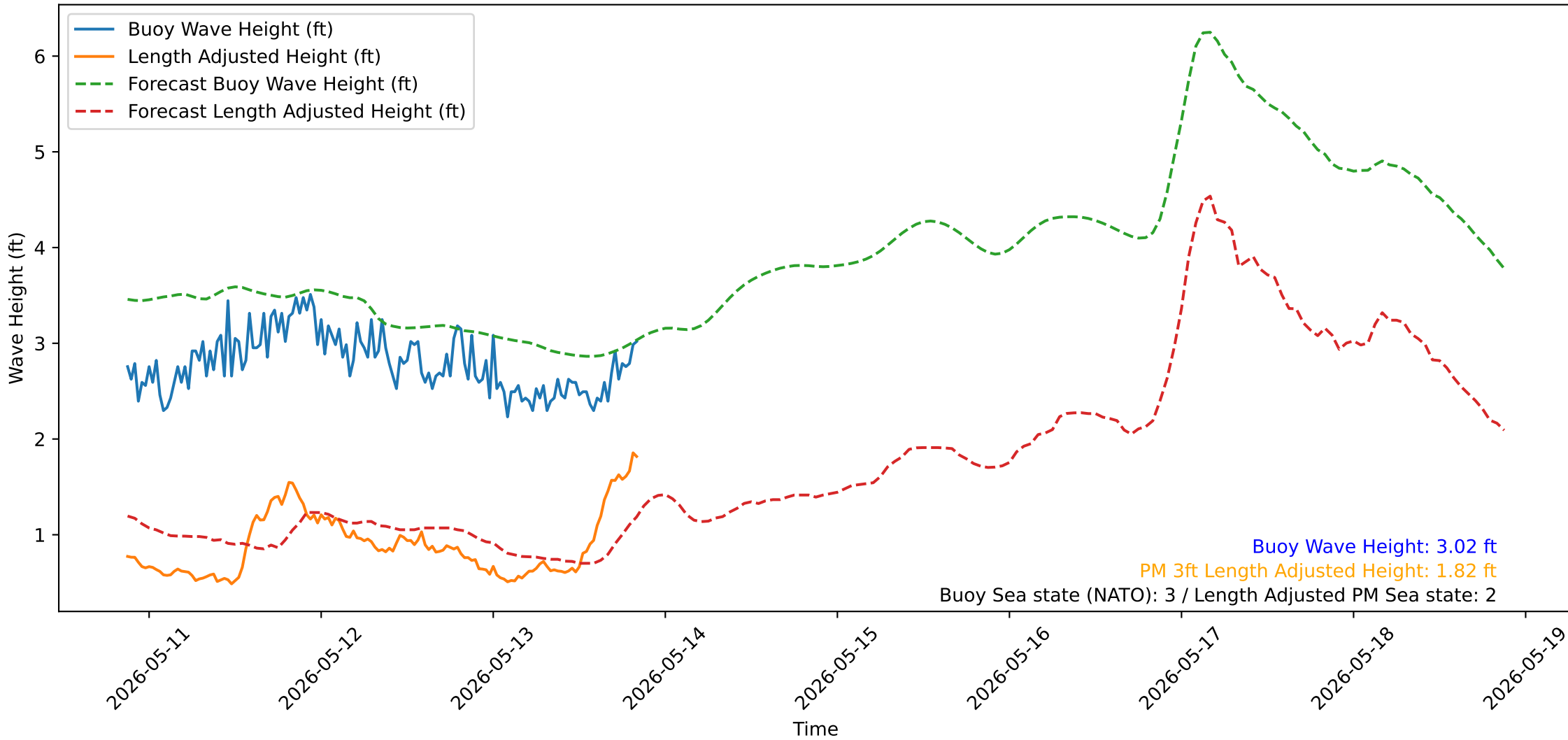
Wave Heights over Time for Green Beach at 2026-05-13 21:11:13
