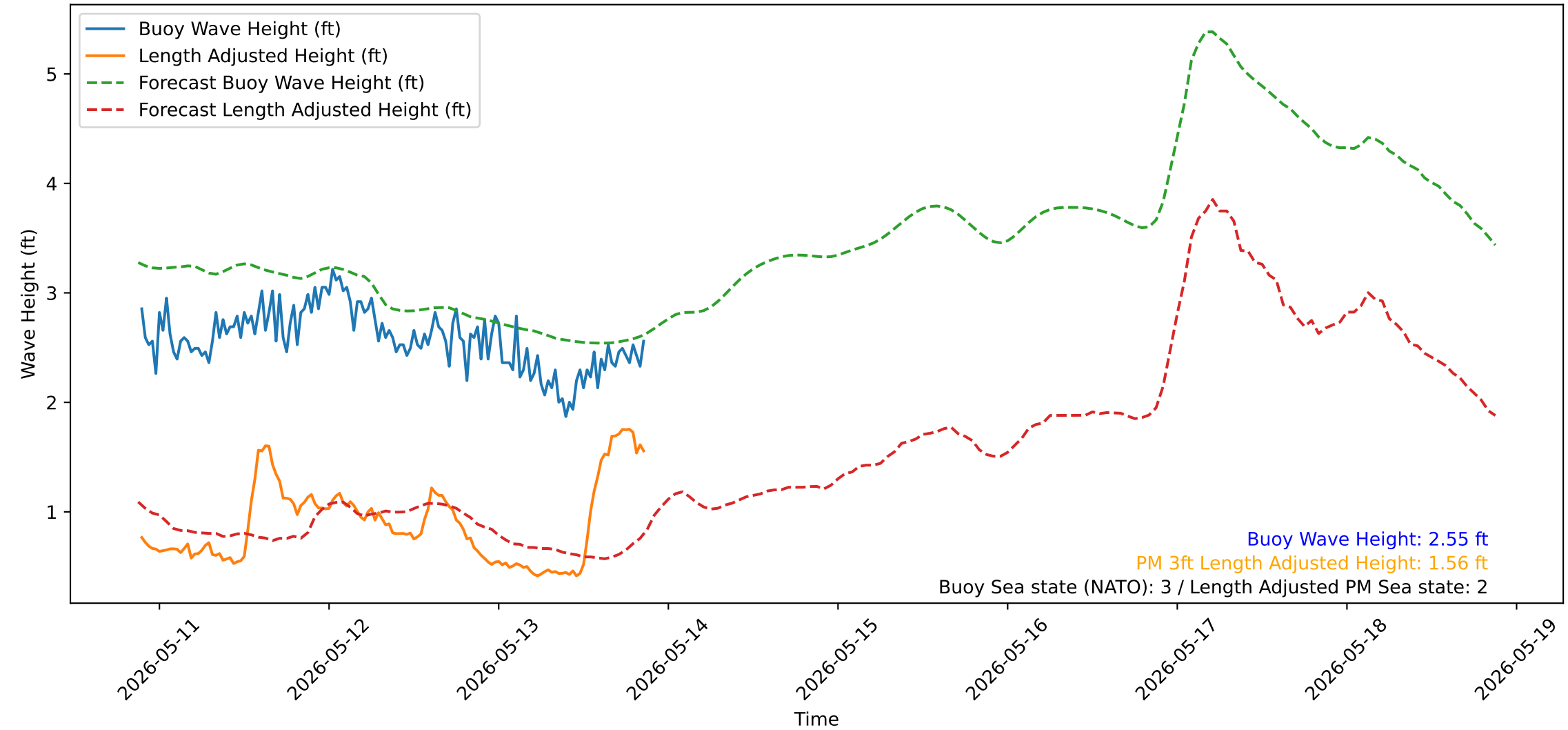
Wave Heights over Time for Red Beach at 2026-05-13 21:10:50
