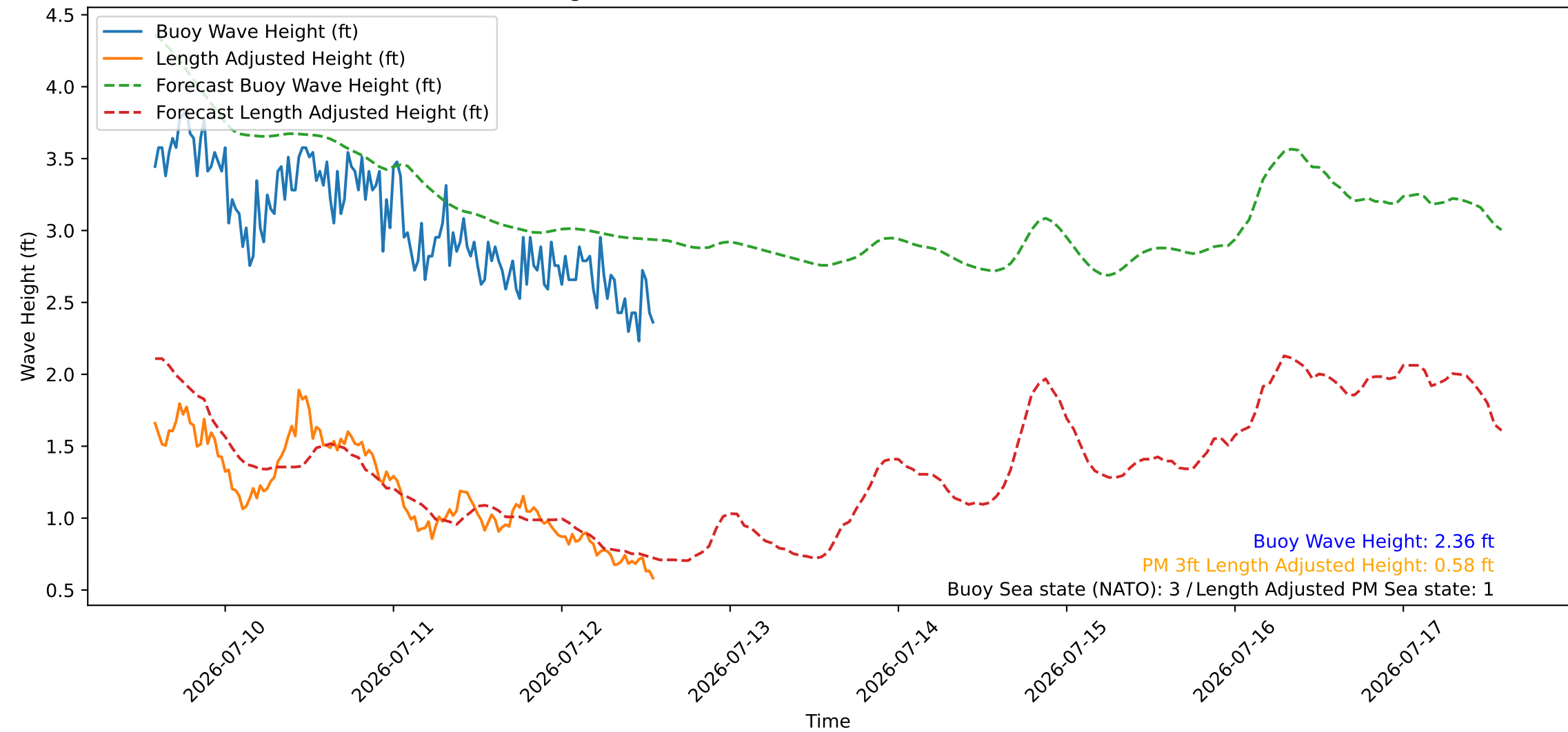
Wave Heights over Time for Green Beach at 2026-07-12 13:51:10
