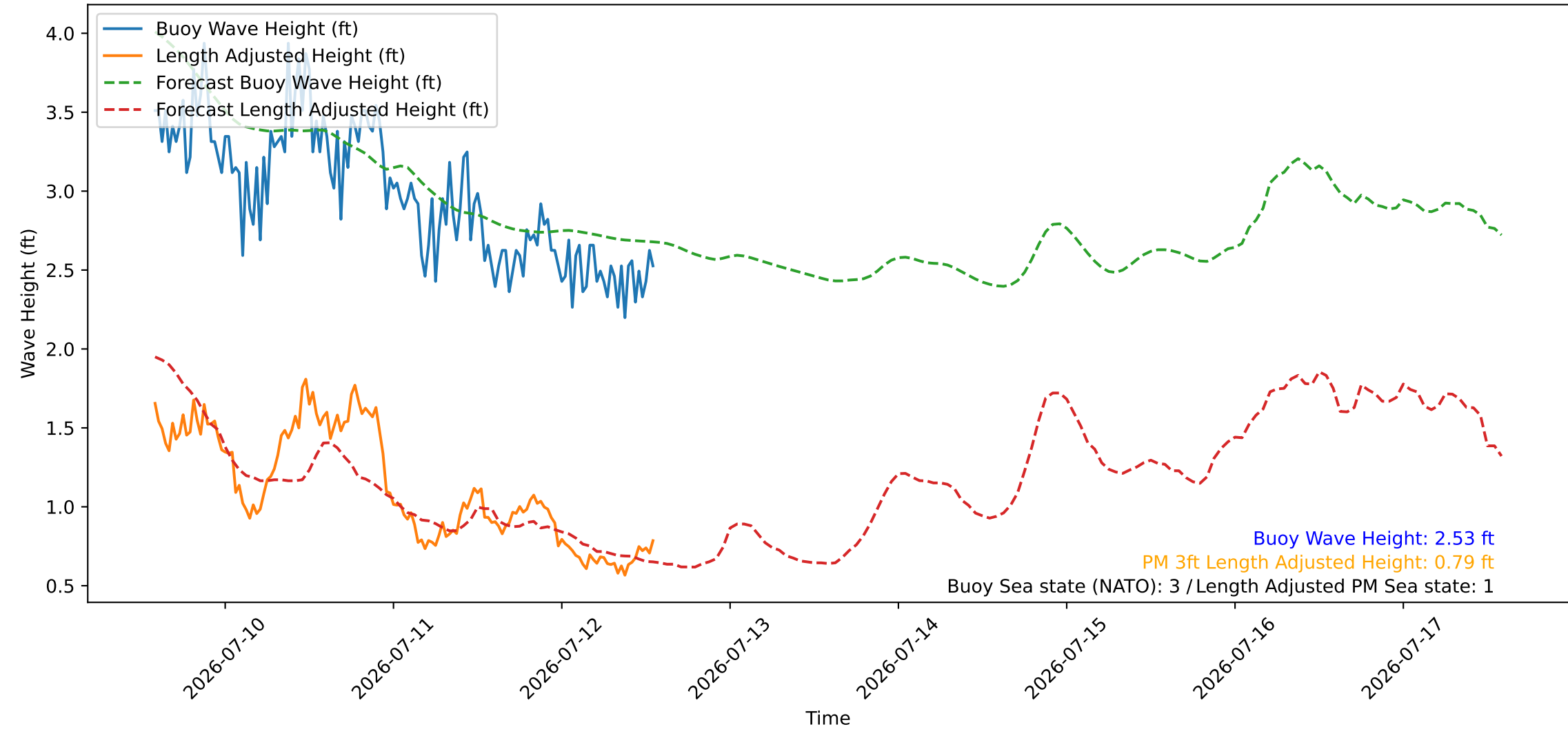
Wave Heights over Time for Red Beach at 2026-07-12 13:50:48
