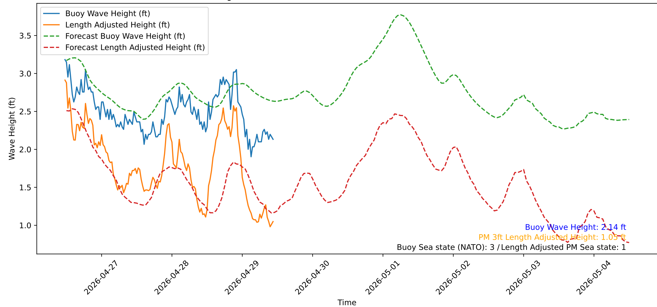
Wave Heights over Time for Oceanside Harbor at 2026-04-29 11:30:32
