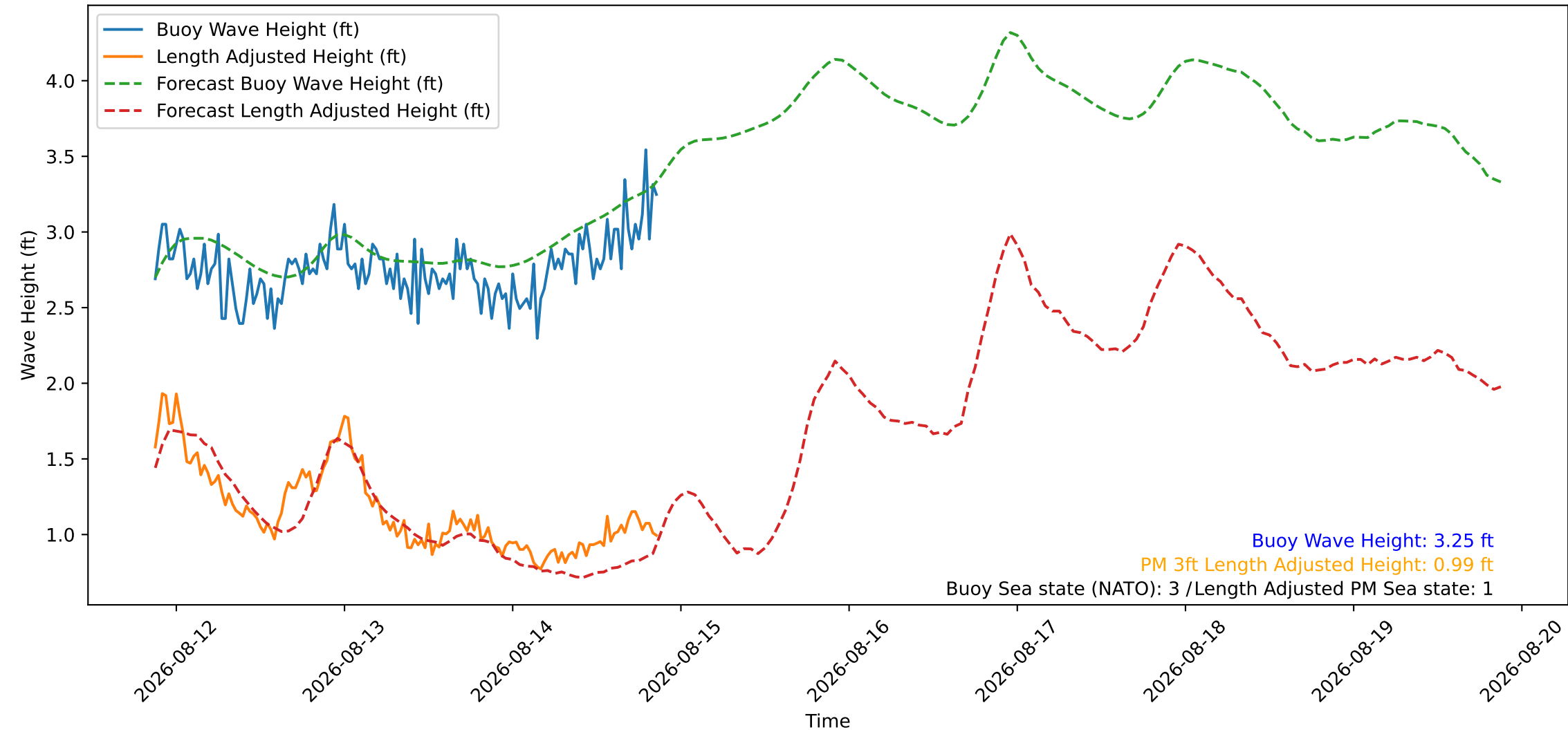
Wave Heights over Time for Oceanside Harbor at 2026-08-14 21:10:27
