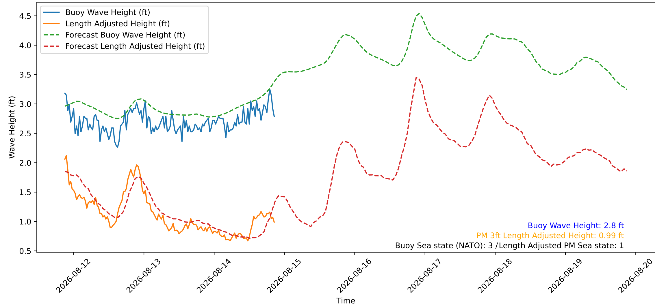
Wave Heights over Time for Green Beach at 2026-08-14 21:11:08
