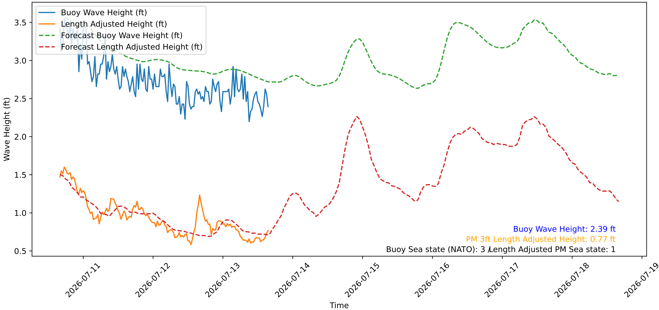
Wave Heights over Time for Green Beach at 2026-07-13 16:11:08
