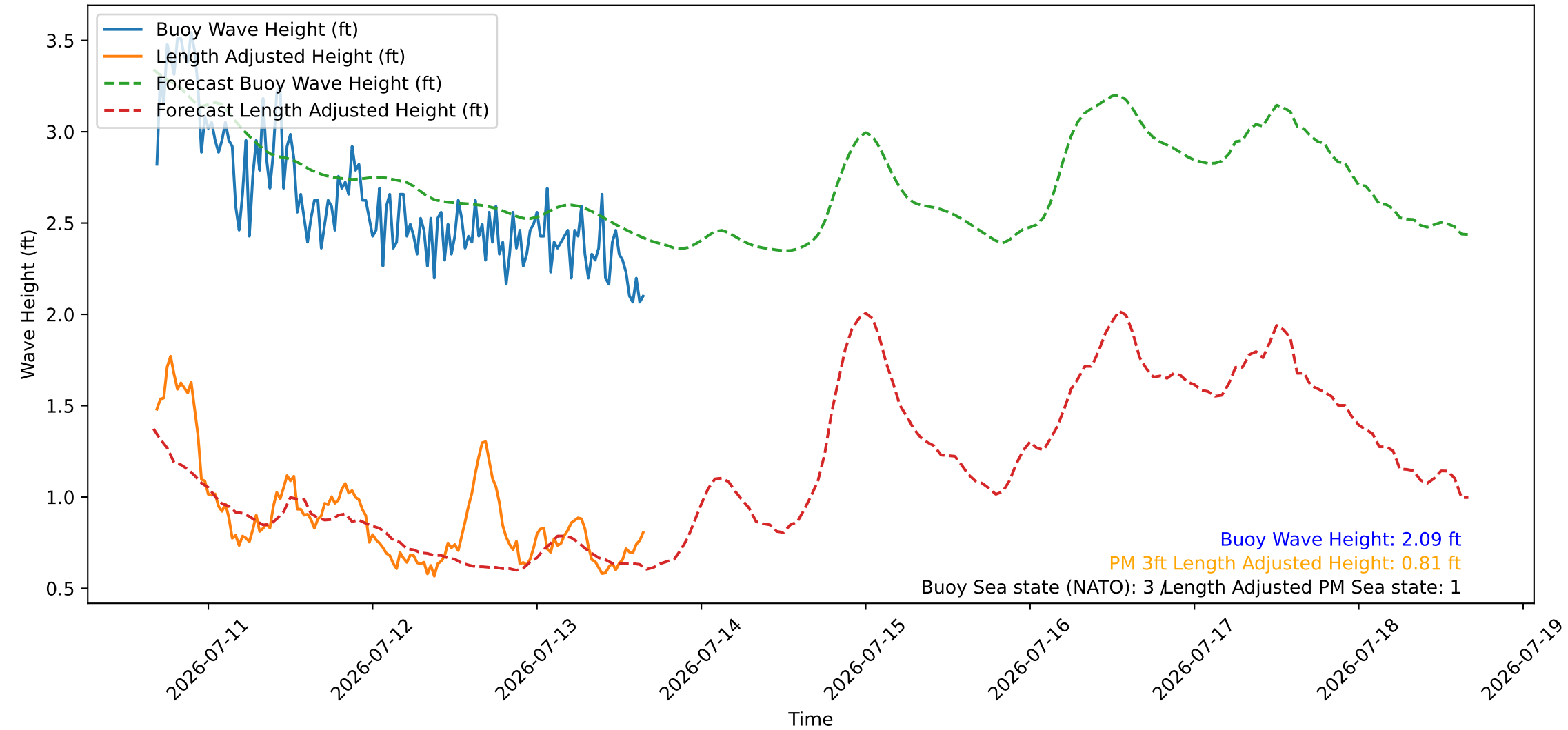
Wave Heights over Time for Red Beach at 2026-07-13 16:10:46
