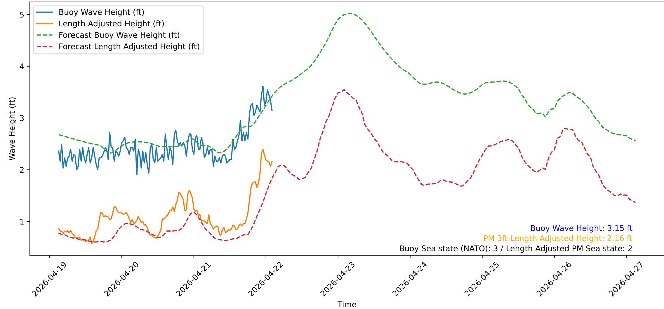
Wave Heights over Time for Oceanside Harbor at 2026-04-22 02:50:31
