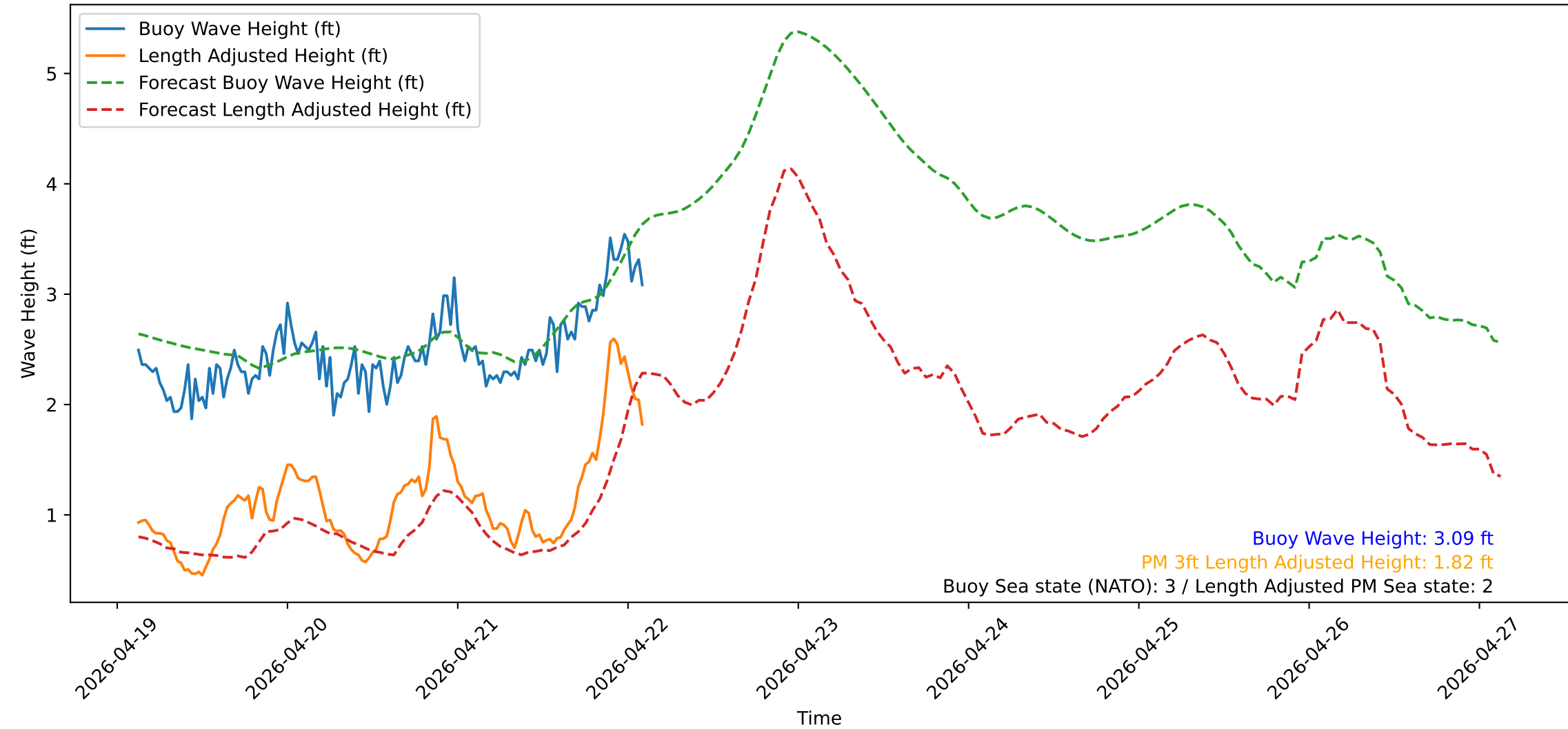
Wave Heights over Time for Green Beach at 2026-04-22 02:51:13
