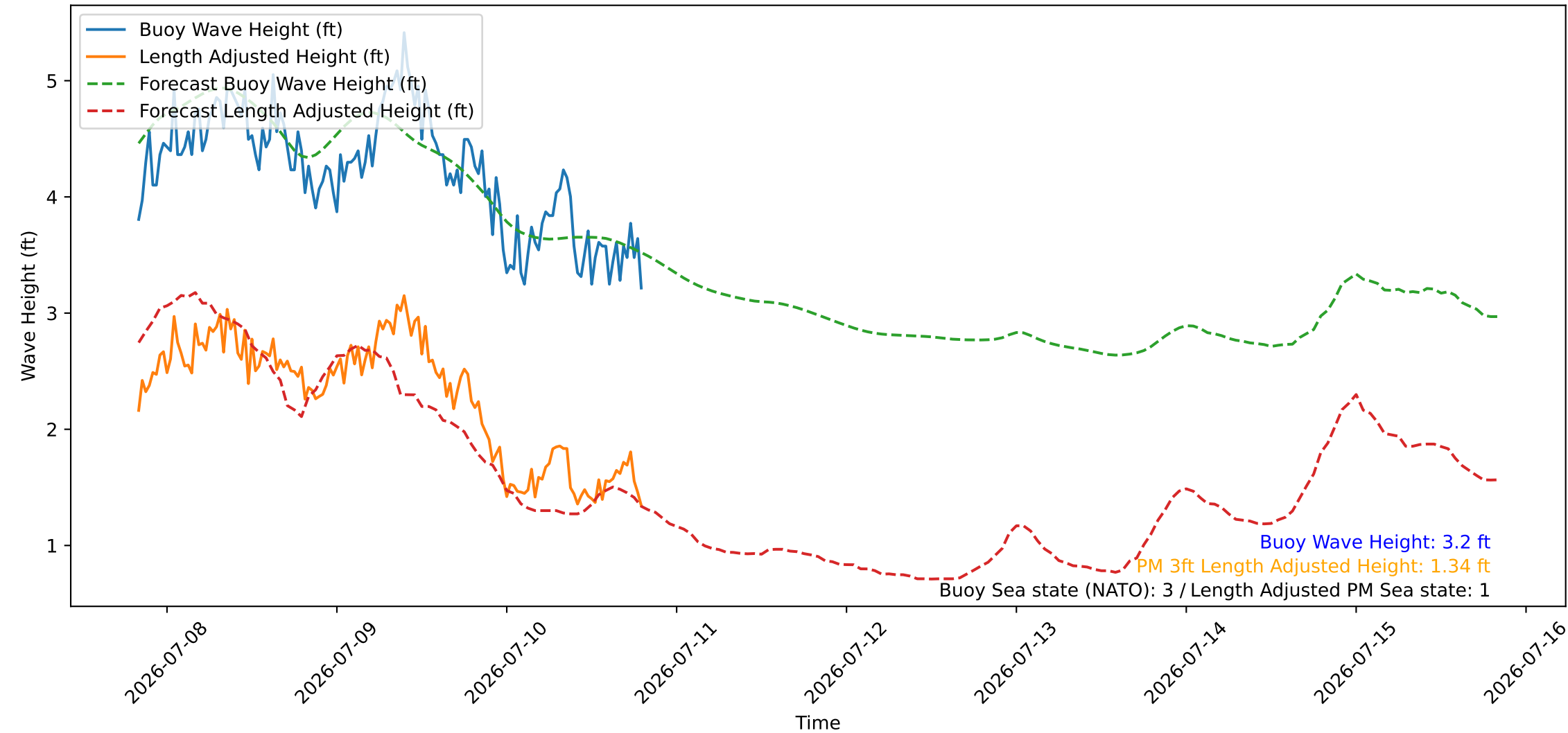
Wave Heights over Time for Oceanside Harbor at 2026-07-10 19:50:26
