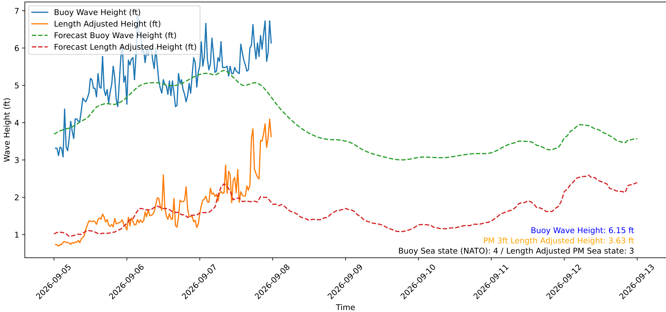
Wave Heights over Time for Red Beach at 2026-09-08 00:20:50
