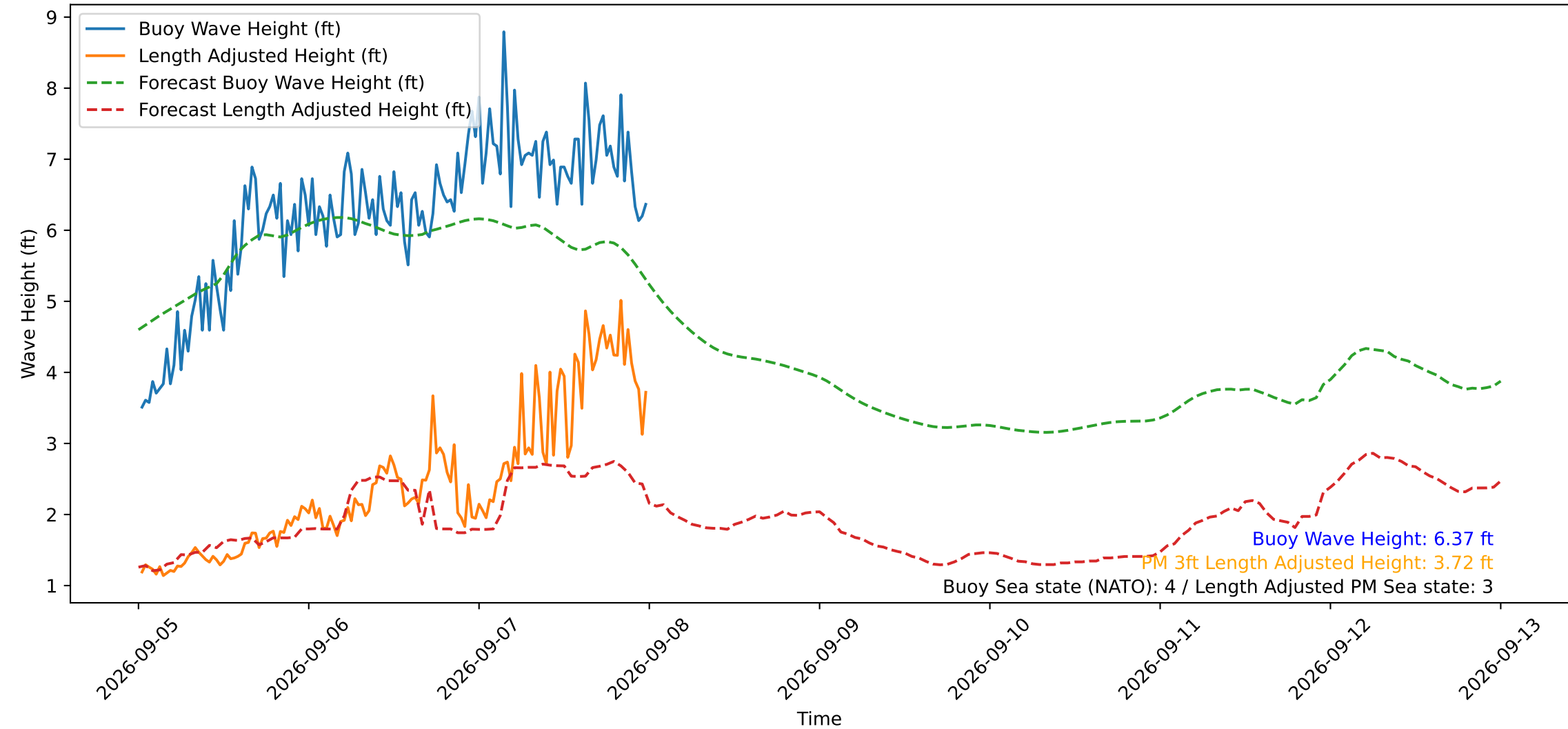
Wave Heights over Time for Green Beach at 2026-09-08 00:21:14
