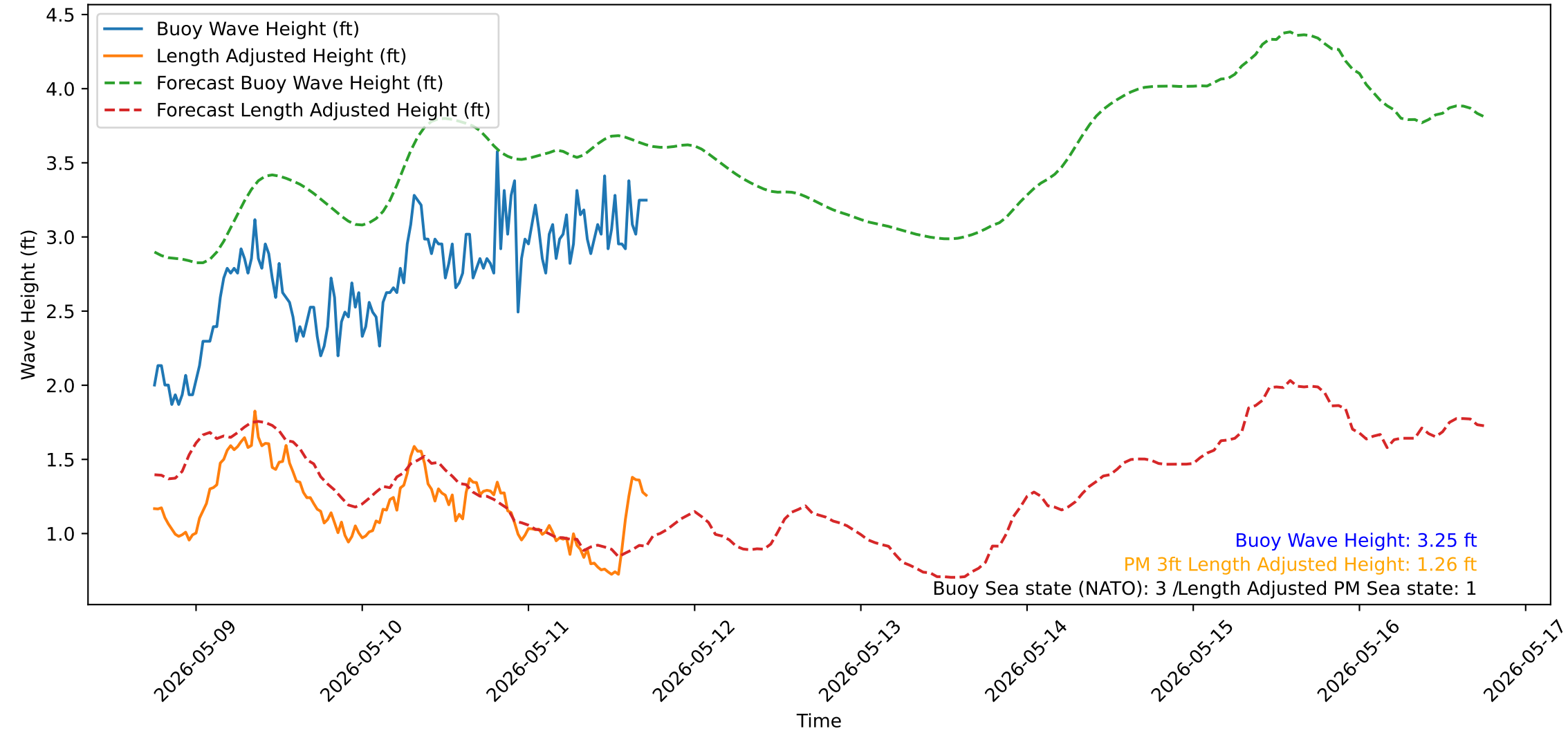
Wave Heights over Time for Oceanside Harbor at 2026-05-11 17:50:31
