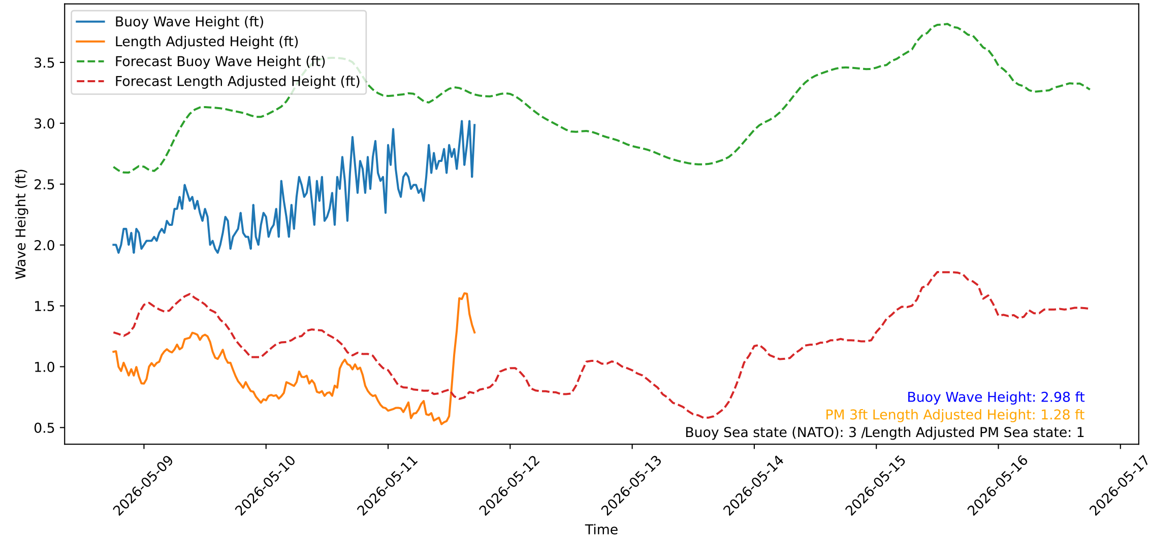
Wave Heights over Time for Red Beach at 2026-05-11 17:50:51
