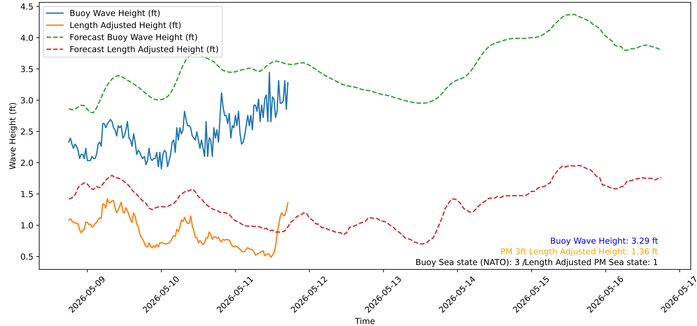
Wave Heights over Time for Green Beach at 2026-05-11 17:51:14
