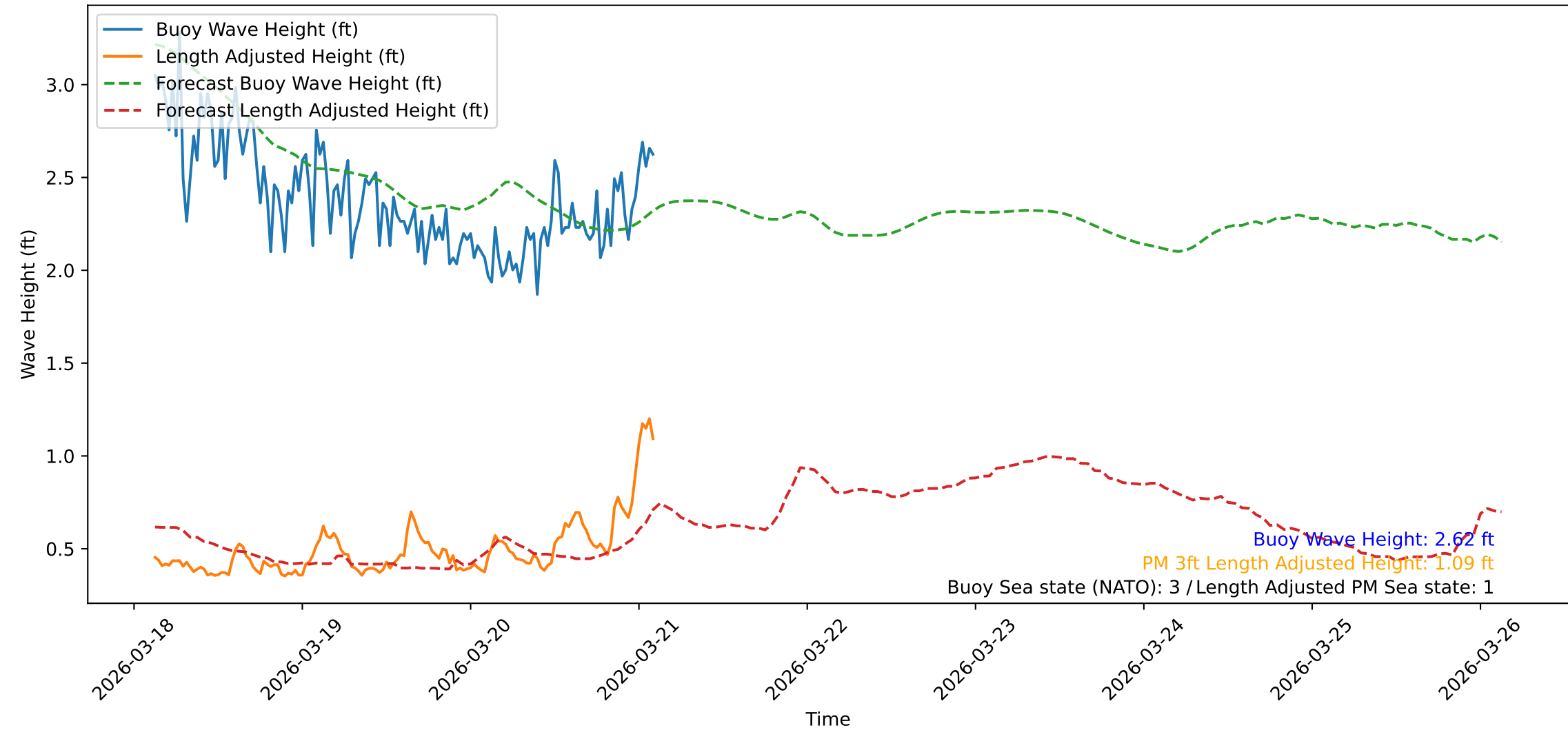
Wave Heights over Time for Red Beach at 2026-03-21 02:50:47
