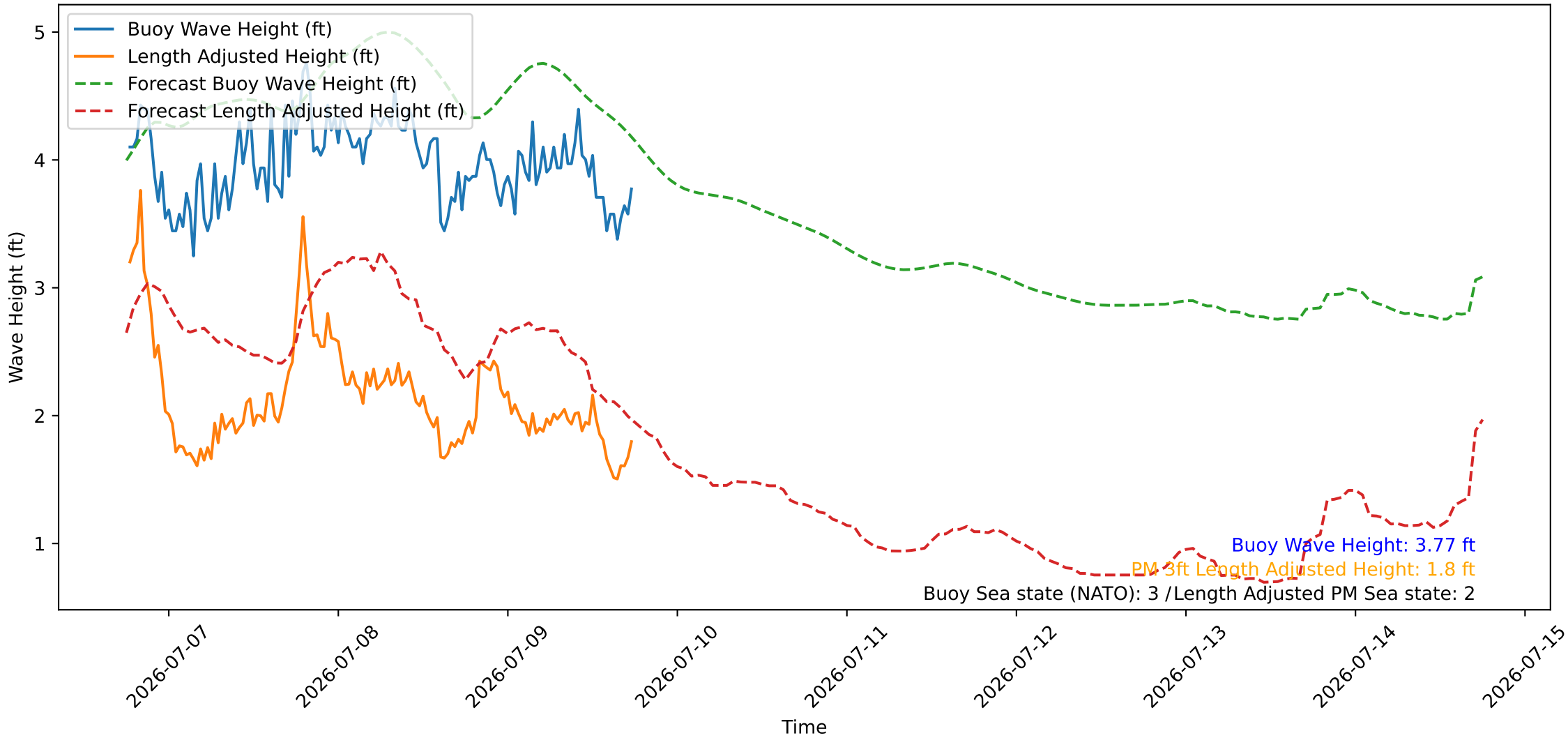
Wave Heights over Time for Green Beach at 2026-07-09 18:21:10
