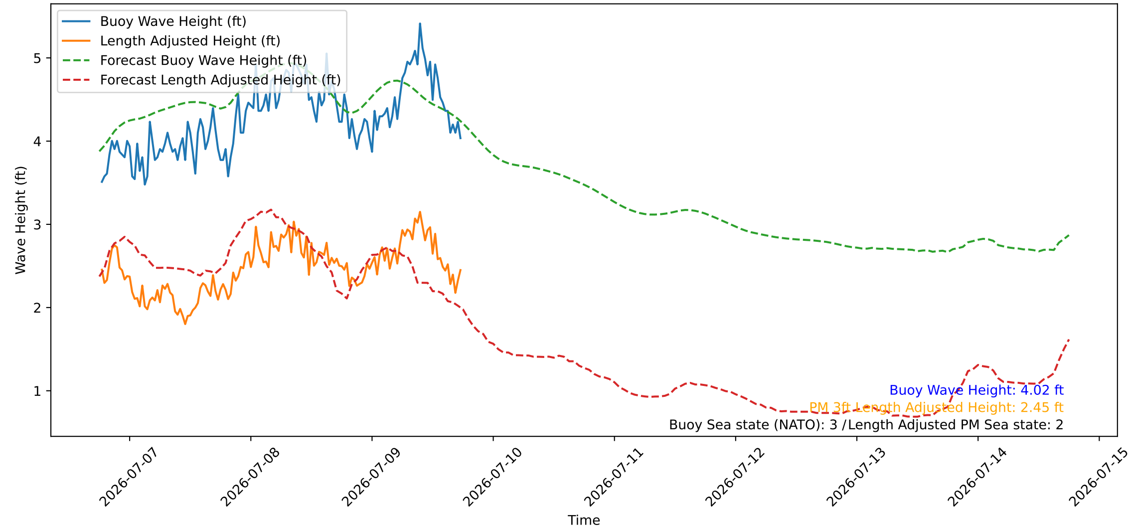
Wave Heights over Time for Oceanside Harbor at 2026-07-09 18:20:26
