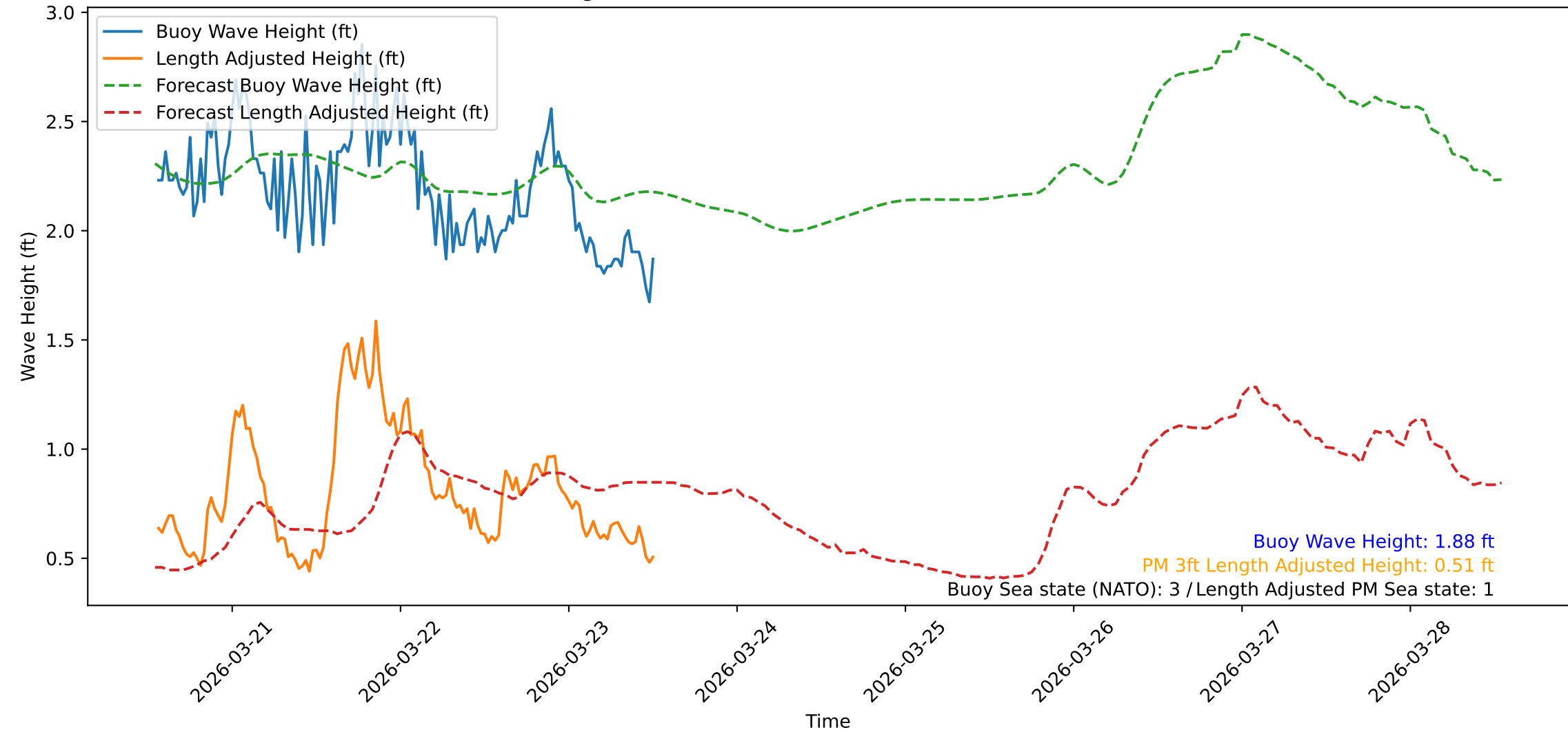
Wave Heights over Time for Red Beach at 2026-03-23 13:10:47
