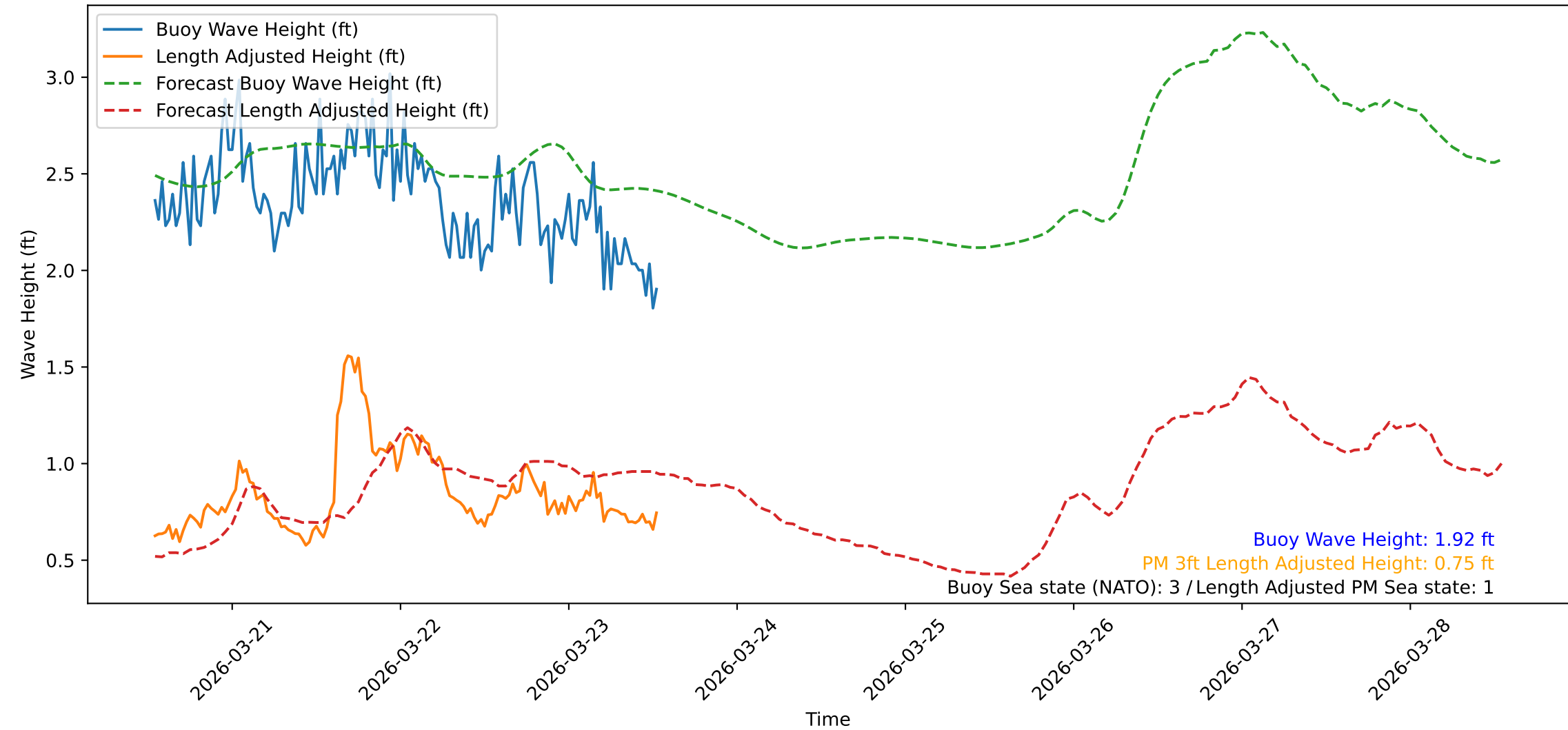
Wave Heights over Time for Oceanside Harbor at 2026-03-23 13:10:31
