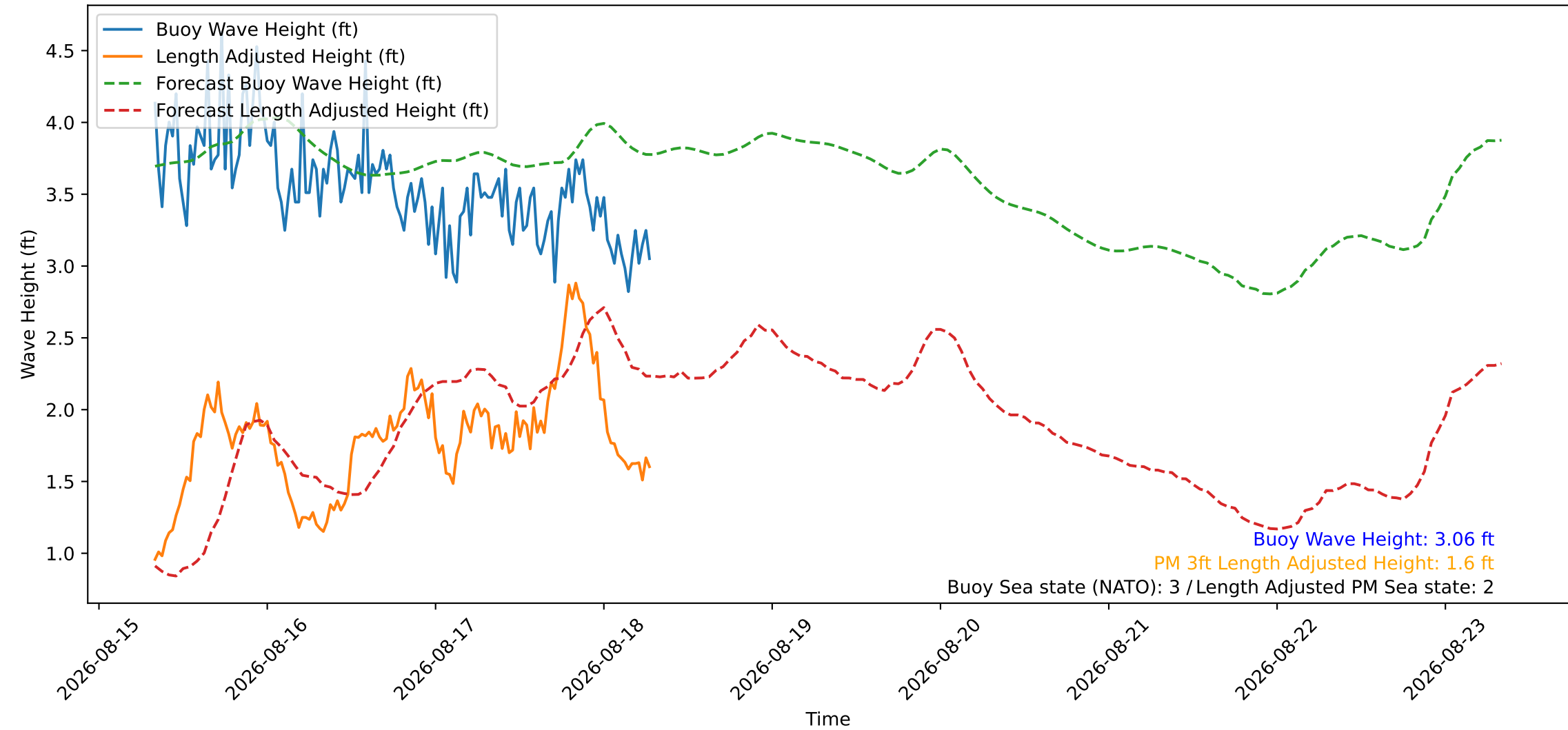
Wave Heights over Time for Oceanside Harbor at 2026-08-18 07:50:27
