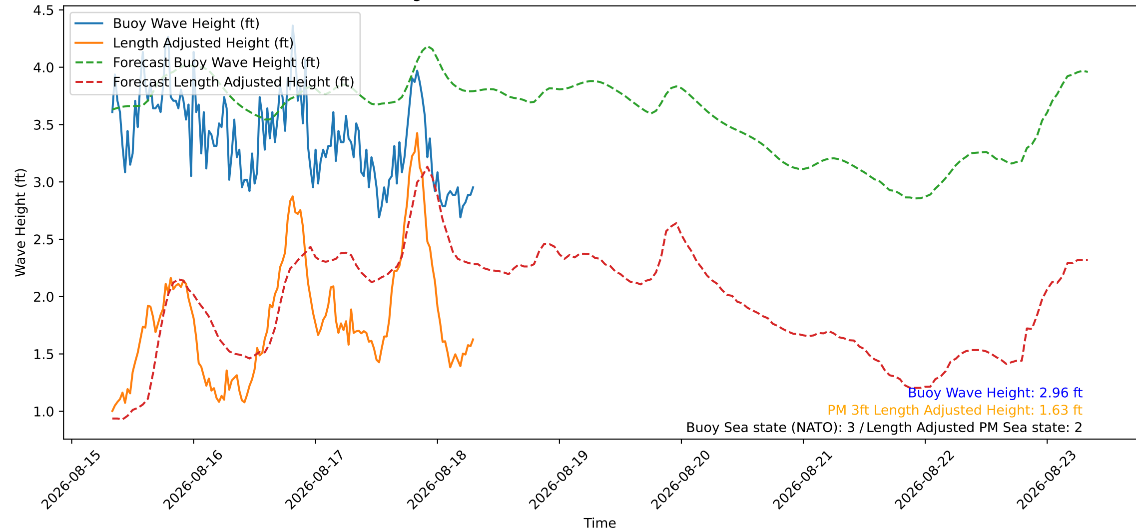
Wave Heights over Time for Green Beach at 2026-08-18 07:51:11
