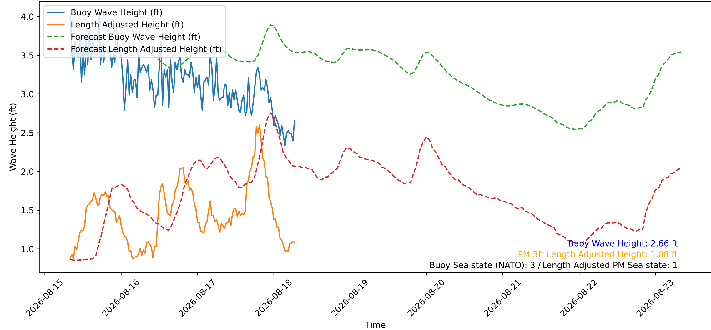
Wave Heights over Time for Red Beach at 2026-08-18 07:50:47
